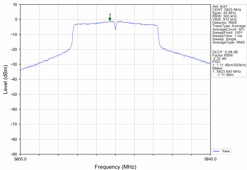
802.11ac(VHT20)_HCH_5825MHz_Ant1_NTNV
