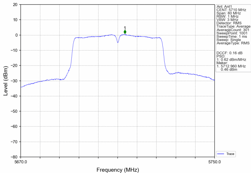
802.11ac(VHT40)_HCH_5710MHz_Ant1_NTNV
