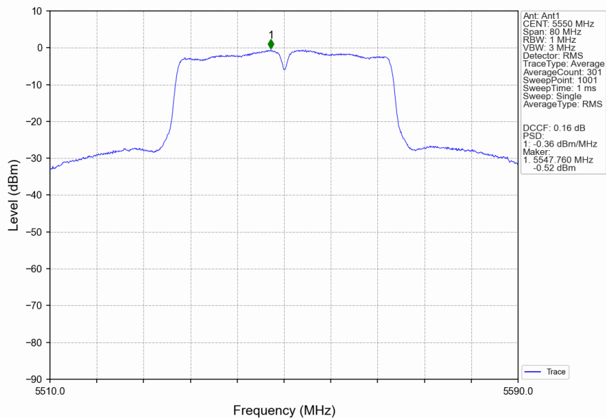
802.11n(HT40)_MCH_5550MHz_Ant1_NTNV
