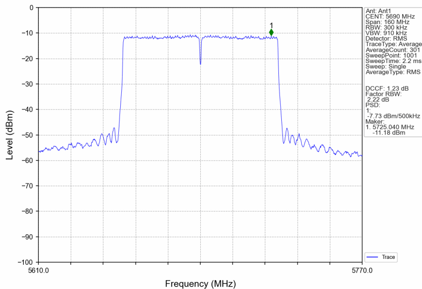
802.11ac(VHT80)_HCH_5690MHz_Ant1_NTNV
