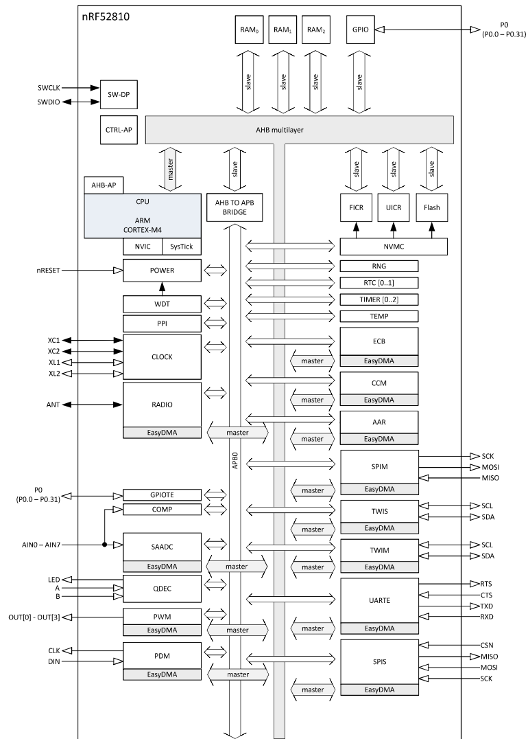
Figure 1: Block diagram
