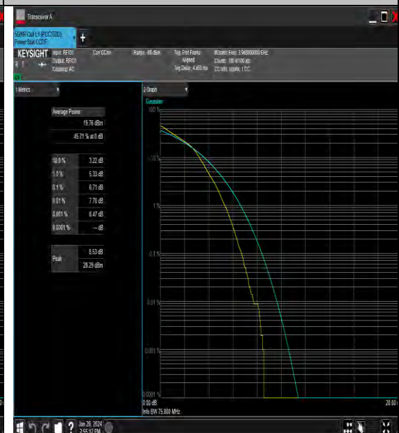
NTNV_N77-3700-3980_PC3_30_70_H_TID3_#1
