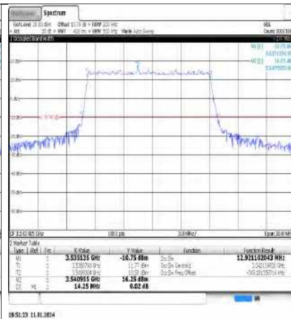
NTNV_N77-3450- 3550_PC3_30_15_H_TID2_Ant1#1
