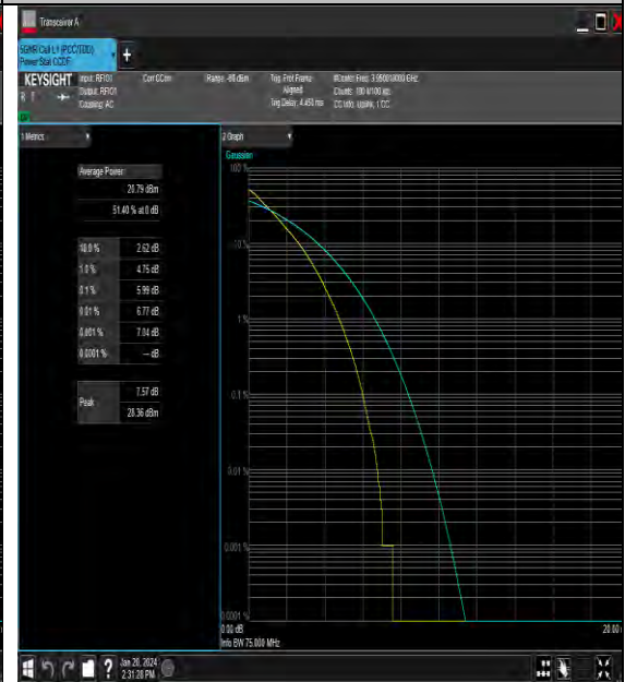
NTNV_N77-3700-3980_PC3_30_60_H_TID2_#1
