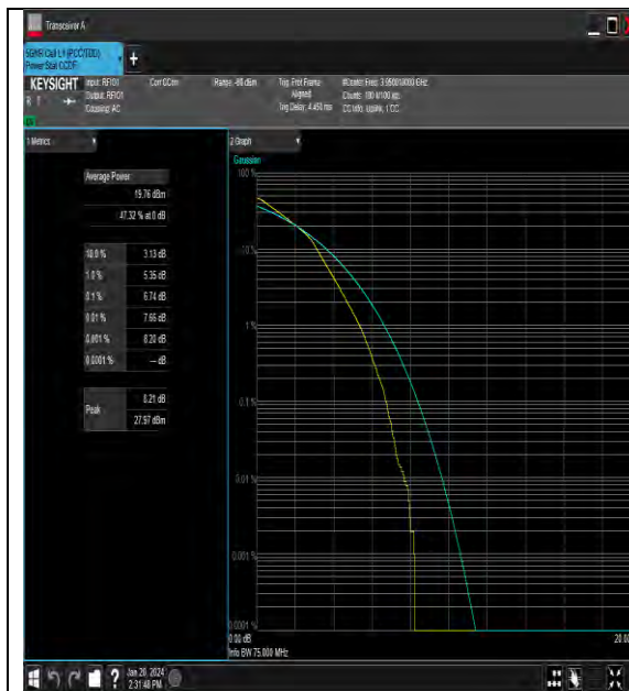
NTNV_N77-3700-3980_PC3_30_60_H_TID3_#1
