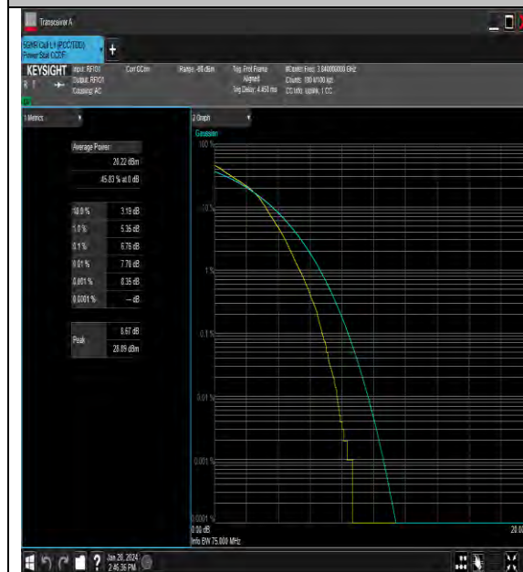
NTNV_N77-3700-3980_PC3_30_70_M_TID3_#1
