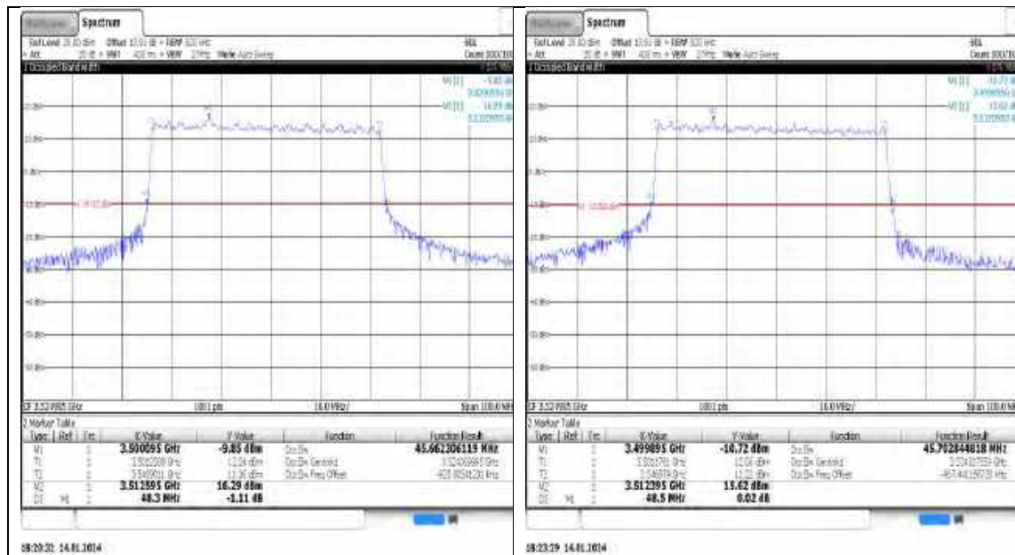
NTNV_N77-3450- 3550_PC3_30_50_H_TID1_Ant1#1
