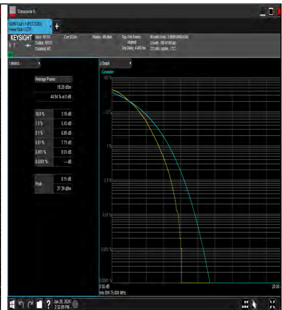
NTNV_N77-3700-3980_PC3_30_60_H_TID4_#1
