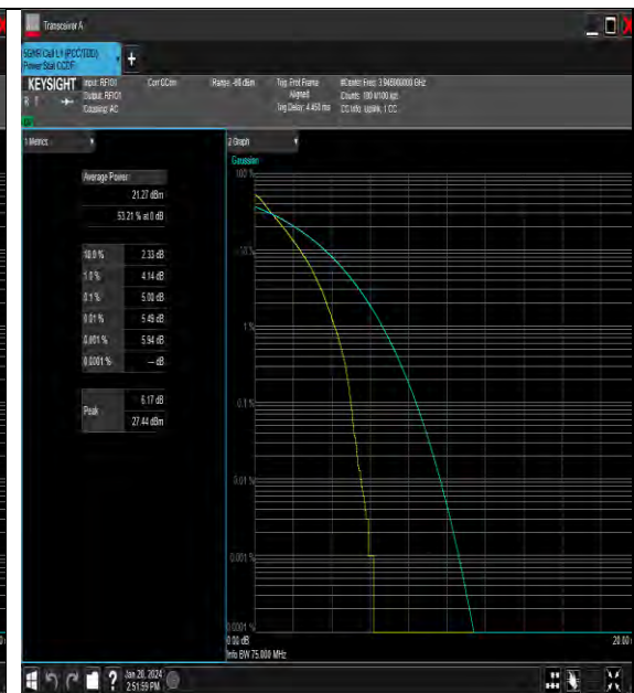
NTNV_N77-3700-3980_PC3_30_70_H_TID1_#1
