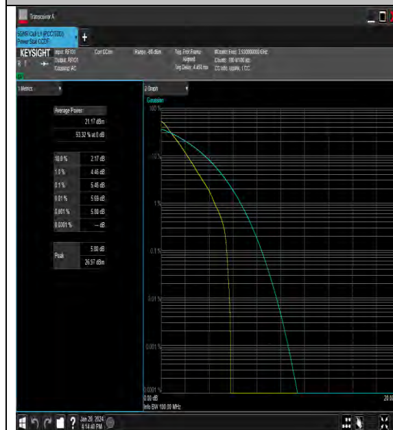
NTNV_N77-3700-3980_PC3_30_100_H_TID1_#1
