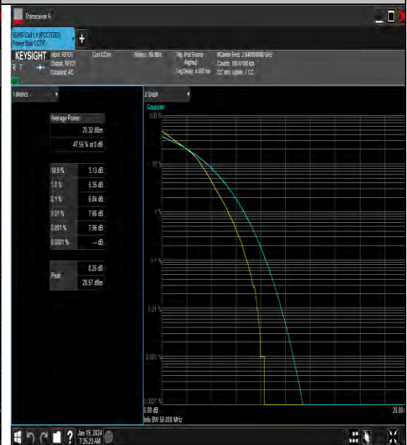
NTNV_N77-3700-3980_PC3_30_40_M_TID3_#1
