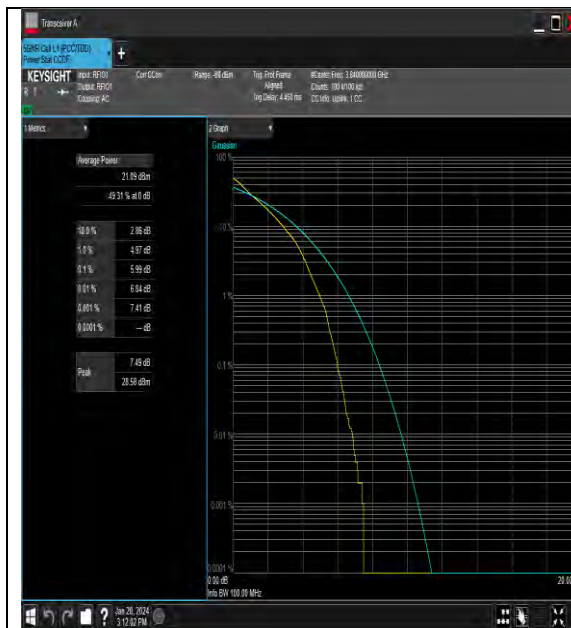
NTNV_N77-3700-3980_PC3_30_80_M_TID2_#1
