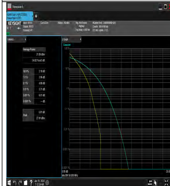
NTNV_N77-3700-3980_PC3_30_40_M_TID1_#1
