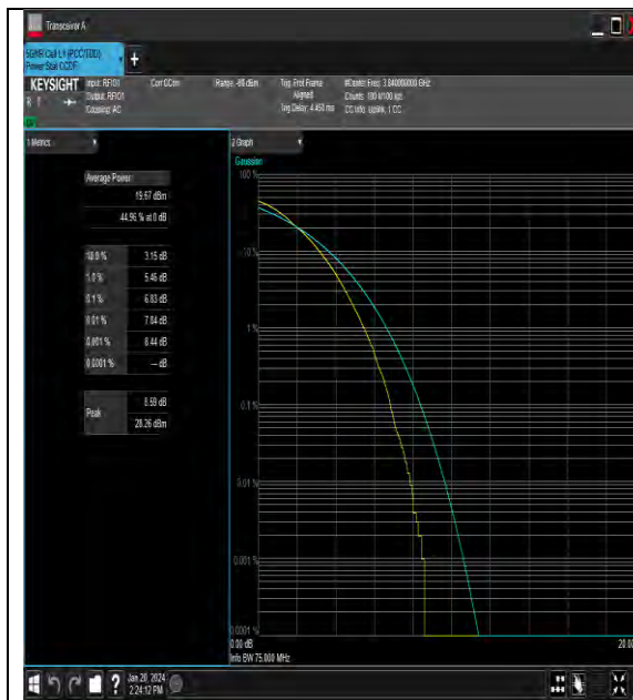
NTNV_N77-3700-3980_PC3_30_60_M_TID4_#1
