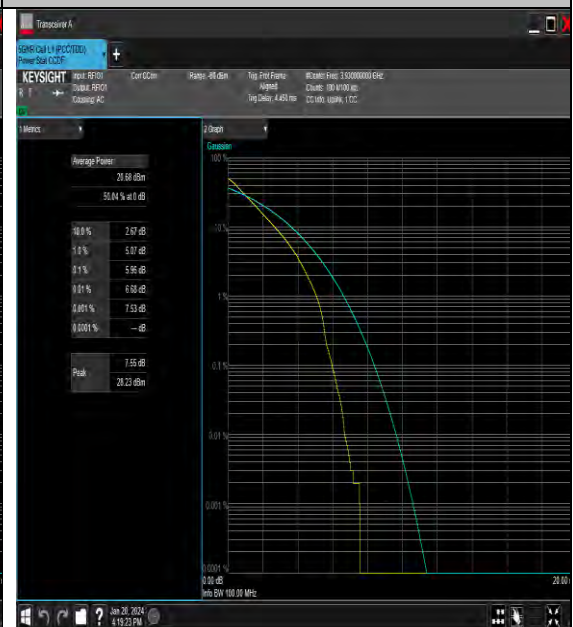
NTNV_N77-3700-3980_PC3_30_100_H_TID2_#1
