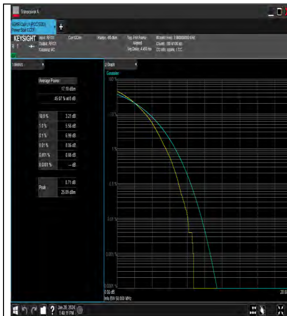
NTNV_N77-3700-3980_PC3_30_40_H_TID5_#1
