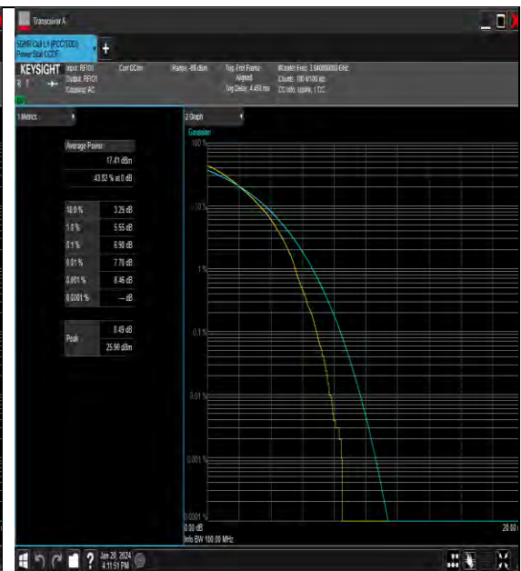
NTNV_N77-3700-3980_PC3_30_100_M_TID5_#1
