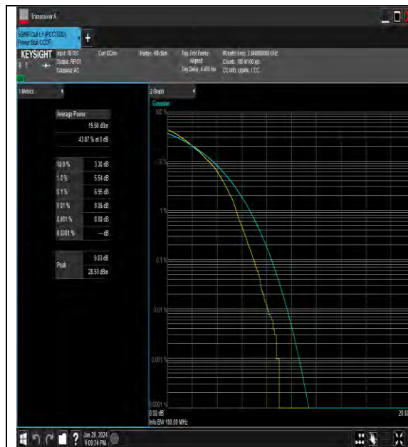
NTNV_N77-3700-3980_PC3_30_100_M_TID4_#1
