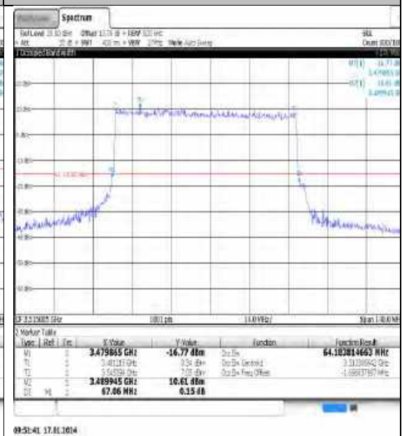
NTNV_N77-3450- 3550_PC3_30_70_H_TID4_Ant1#1
