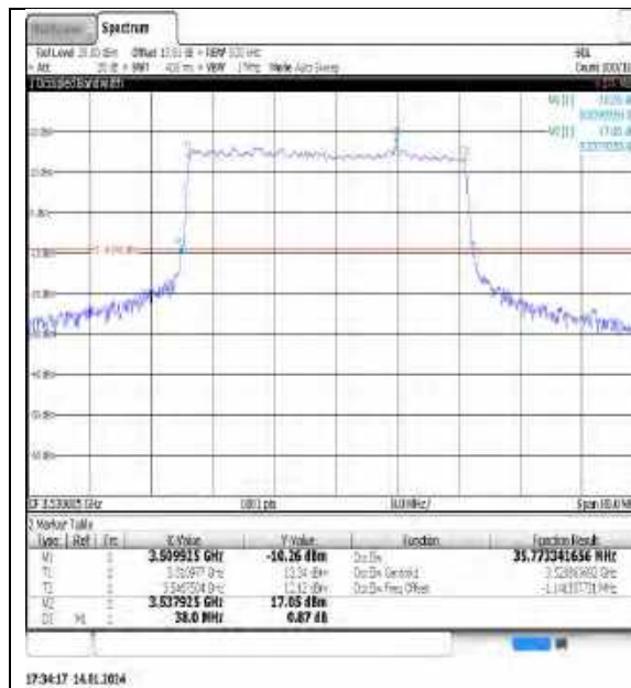
NTNV_N77-3450- 3550_PC3_30_40_H_TID1_Ant1#1
