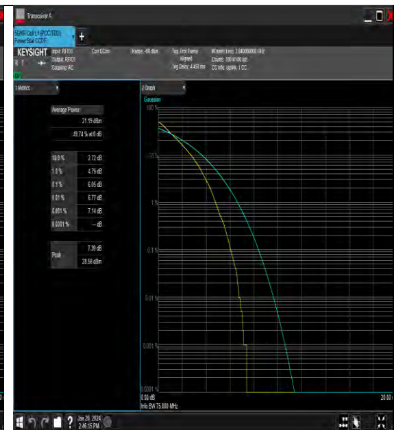
NTNV_N77-3700-3980_PC3_30_70_M_TID2_#1
