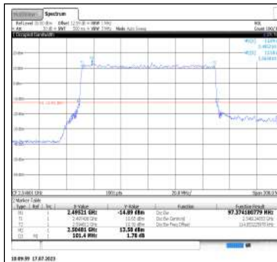
1-N41-PC3-30-100-L-6-CP-16QAM- Outer_Full-273@0-Ant1-97.374-101.400- ≤100-PASS
