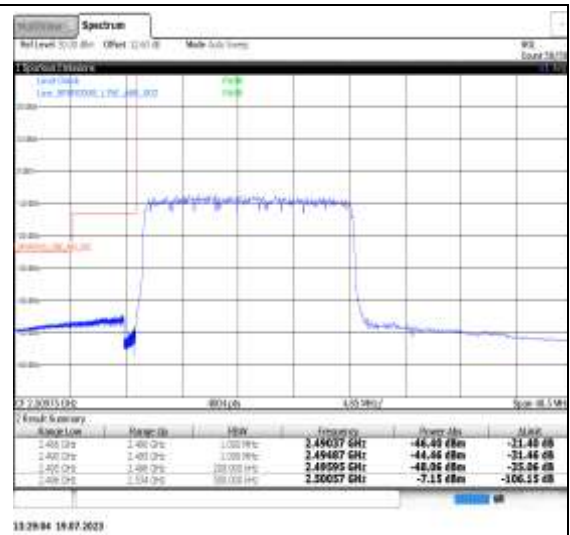
1-N41-PC3-30-20-L-15-DFT-256QAM-Outer_Full-50@0-Ant1-1--PASS-see graph
