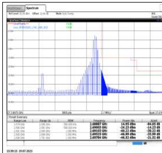
1-N41-PC3-30-20-H-11-DFT-64QAM-Edge_1RB_Right-1@50-Ant1-1--PASS-see graph
