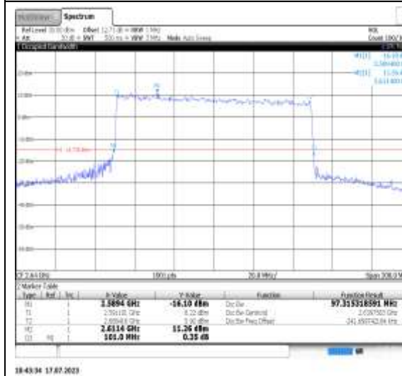
1-N41-PC3-30-100-H-8-CP-256QAM- Outer_Full-273@0-Ant1-97.315-101.000- ≤100-PASS
