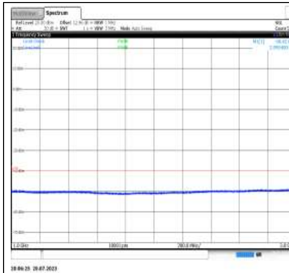
1-N48-PC3-30-100-M-4-N/A-DFT-QPSK- Edge_1RB_Left-1@0-1000-3000-Ant1- 2999.40--48.42--40-PASS
