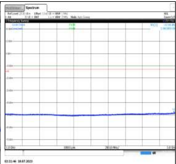
1-N5-PC3-15-20-H-8-N/A-DFT-16QAM- Edge_1RB_Right-1@105-1000-3000-Ant1- 2965.80--47.90--13-PASS
