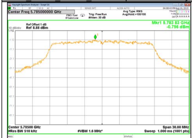
W58_11n20_Middle_Power Spectrum Density
