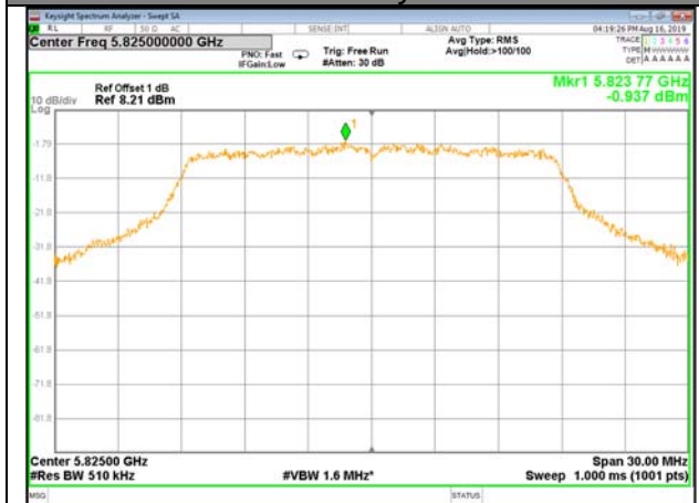
W58_11ac20_Higher_Power Spectrum Density
