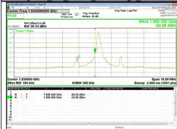
QPSK_5M_Lower_Band edge_1-RB
