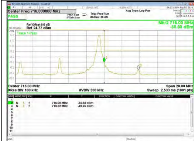
B17_Q16_10M_High_1-RB_Bedge
