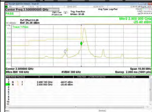
B7_Q16_5M_Low_1-RB_Bedge
