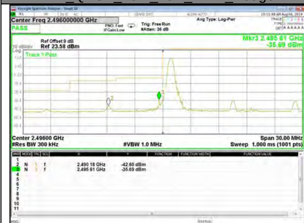
B41_QPSK_15M_Low_1-RB_Bedge
