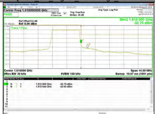
QPSK_3M_Higher_Band edge_Full-RB
