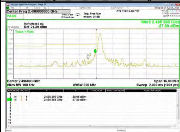
B41_Q16_5M_Low_1-RB_Bedge
