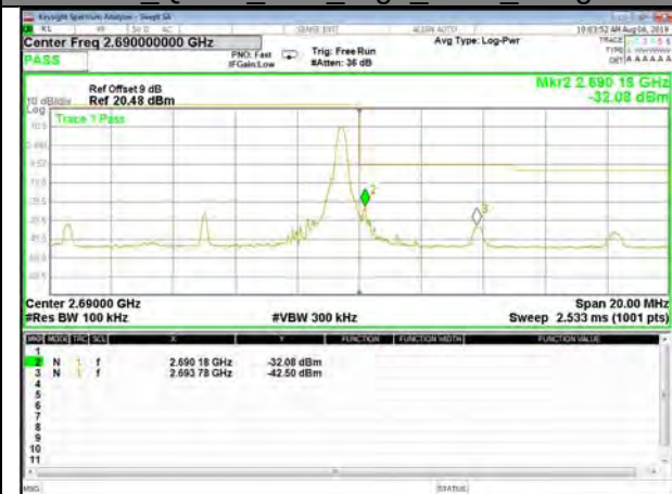
B41_QPSK_10M_High_1-RB_Bedge
