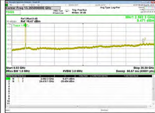
B41_Q16_20M_Mid_CDT_Spurious
