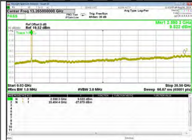
B41_Q16_15M_High_CDT_Spurious
