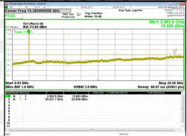
B41_Q16_5M_High_CDT_Spurious
