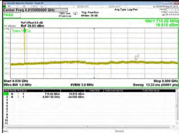
B12_QPSK_1.4M_High_CDT_Spurious
