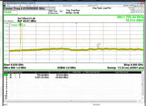
B17_Q16_5M_High_CDT_Spurious
