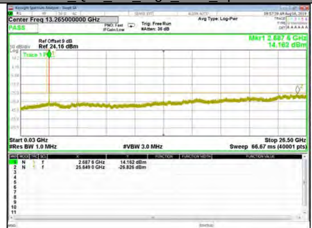
B41_Q16_5M_High_CDT_Spurious
