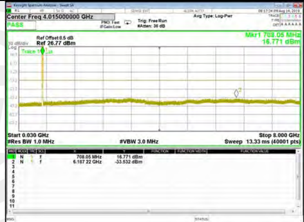
B17_QPSK_10M_High_CDT_Spurious
