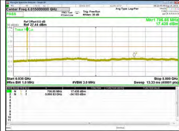
B17_QPSK_5M_Mid_CDT_Spurious
