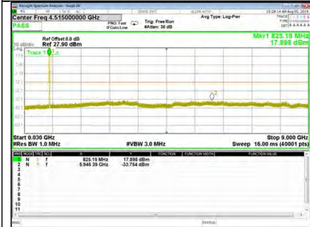
B5_QPSK_3M_Mid_CDT_Spurious
