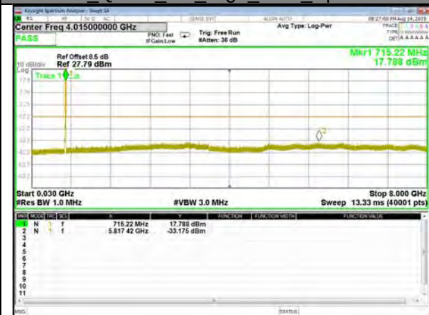
B17_QPSK_5M_High_CDT_Spurious
