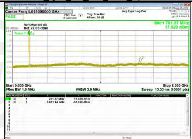
B13_Q16_5M_High_CDT_Spurious
