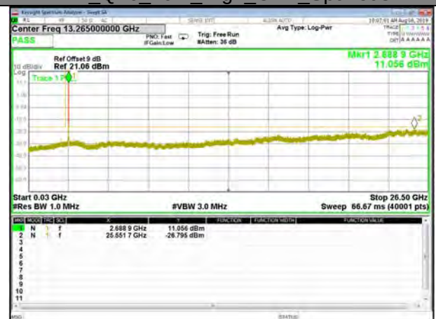
B41_Q16_10M_High_CDT_Spurious
