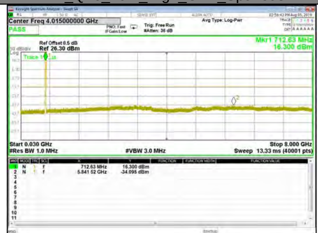
B12_Q16_10M_High_CDT_Spurious
