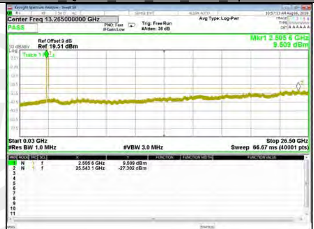
B41_Q16_20M_Low_CDT_Spurious
