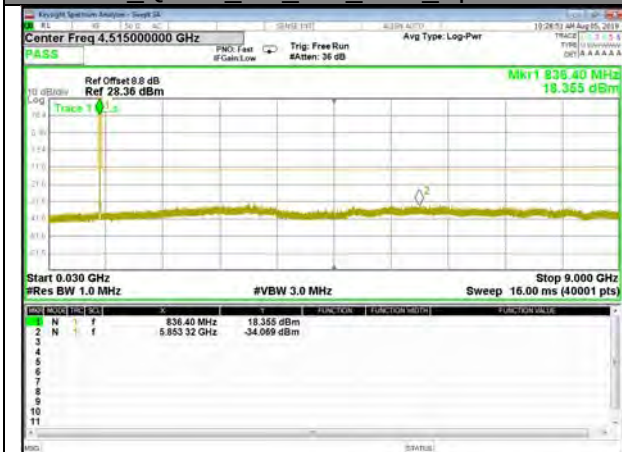
B5_QPSK_3M_High_CDT_Spurious
