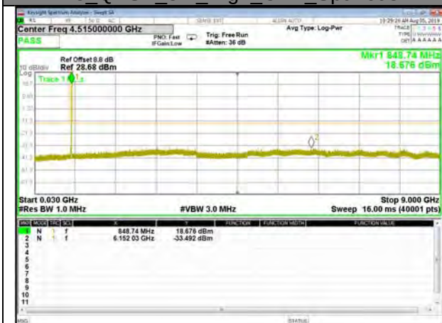
B5_QPSK_3M_High_CDT_Spurious
