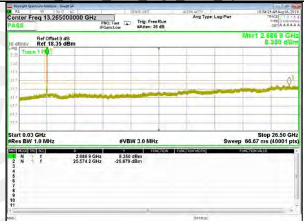
B41_Q16_20M_High_CDT_Spurious
