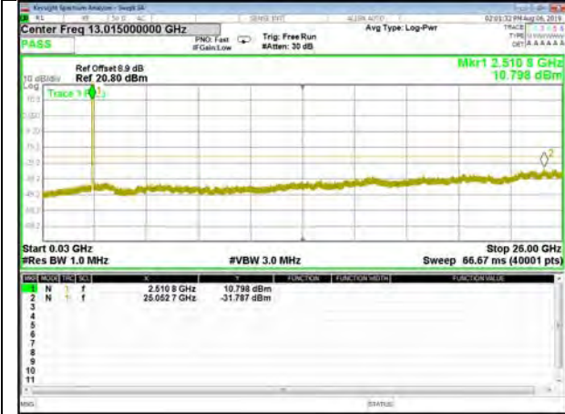
B7_QPSK_20M_Mid_CDT_Spurious
