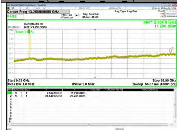
B41_Q16_15M_Low_CDT_Spurious
