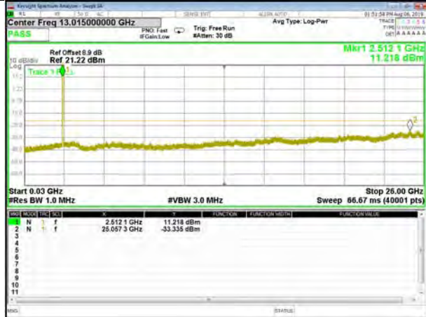
B7_QPSK_15M_Mid_CDT_Spurious
