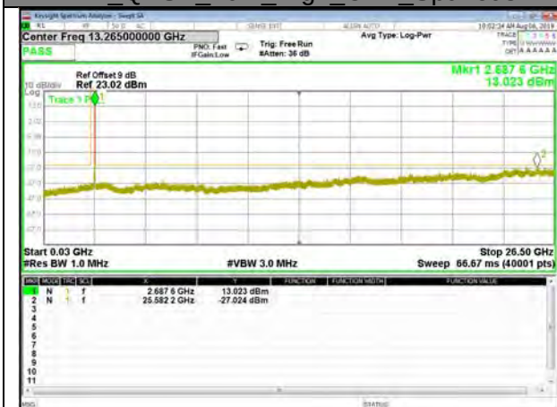
B41_QPSK_10M_High_CDT_Spurious
