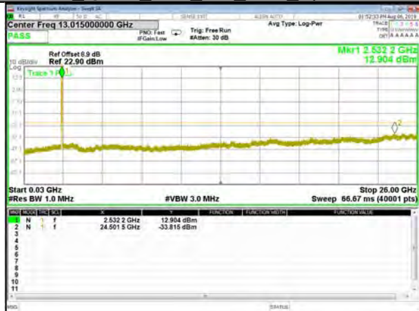
B7_QPSK_15M_High_CDT_Spurious
