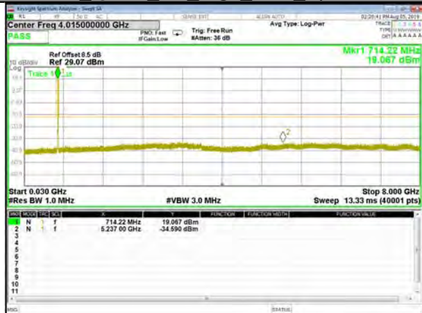
B12_QPSK_3M_High_CDT_Spurious
