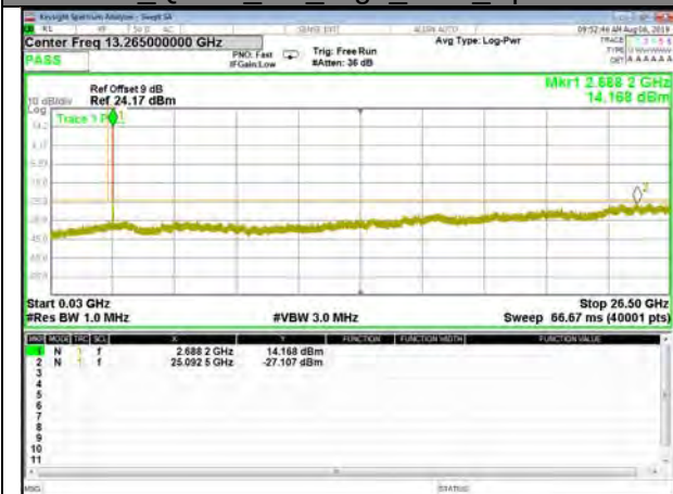
B41_QPSK_5M_High_CDT_Spurious
