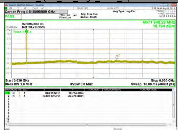
B5_Q16_3M_High_CDT_Spurious
