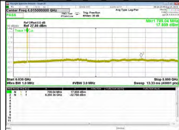
B17_QPSK_5M_High_CDT_Spurious
