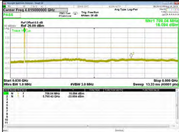
B17_Q16_10M_High_CDT_Spurious
