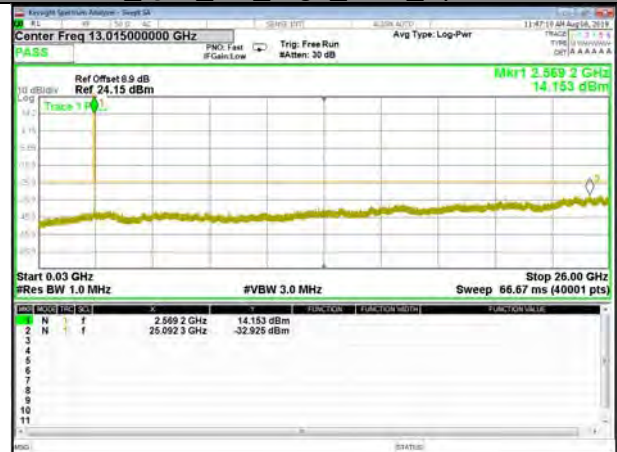
B7_Q16_5M_High_CDT_Spurious
