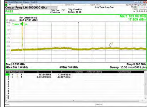
B12_QPSK_5M_Mid_CDT_Spurious
