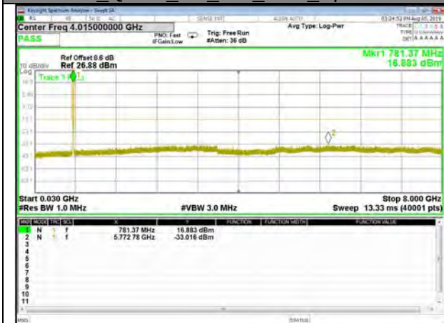
B13_QPSK_5M_High_CDT_Spurious
