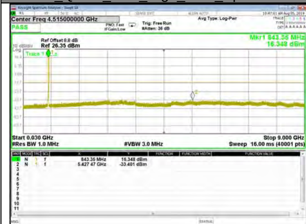
B5_QPSK_10M_High_CDT_Spurious
