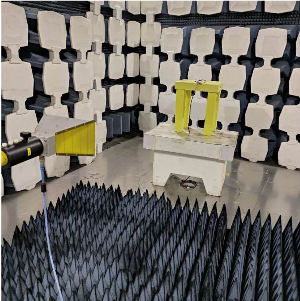
(3) Radiated spurious emission Test Setup-3(Above 1GHz)
