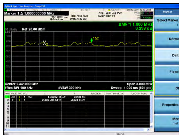
8-DPSK
