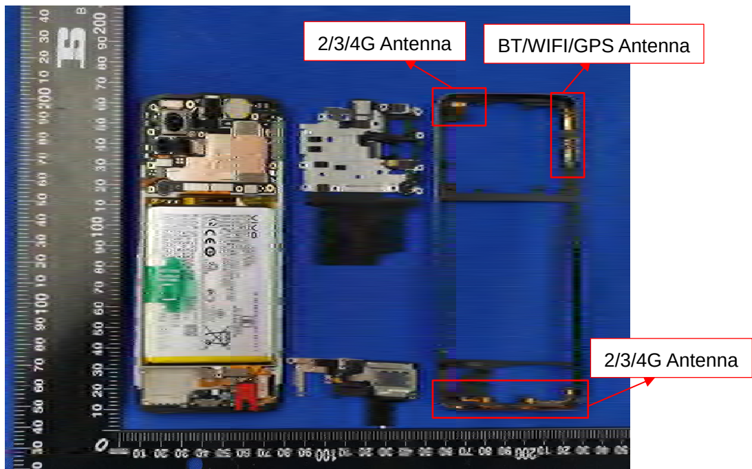
EUT UNCOVER VIEW
