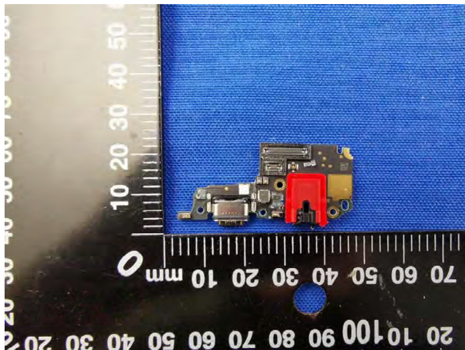
SUB BOARD BACK VIEW
