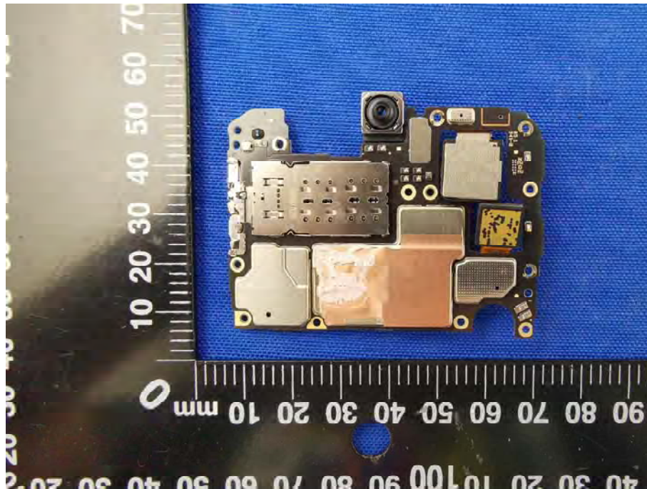
MAIN BOARD BACK VIEW (WITH SHIELDING)
