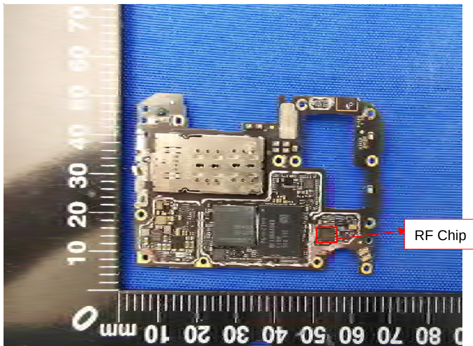
MAIN BOARD BACK VIEW (WITHOUT SHIELDING)
