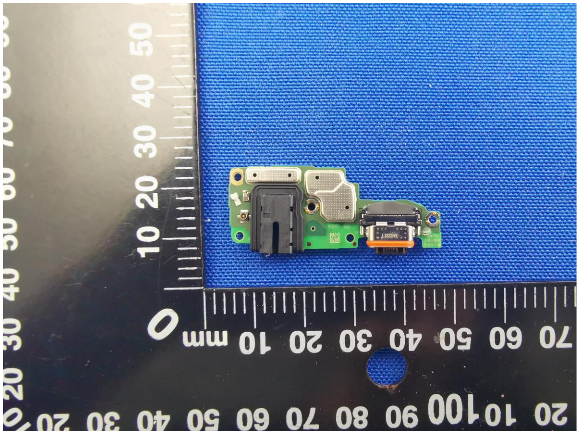
SUB BOARD TOP VIEW (WITH SHIELDING)
