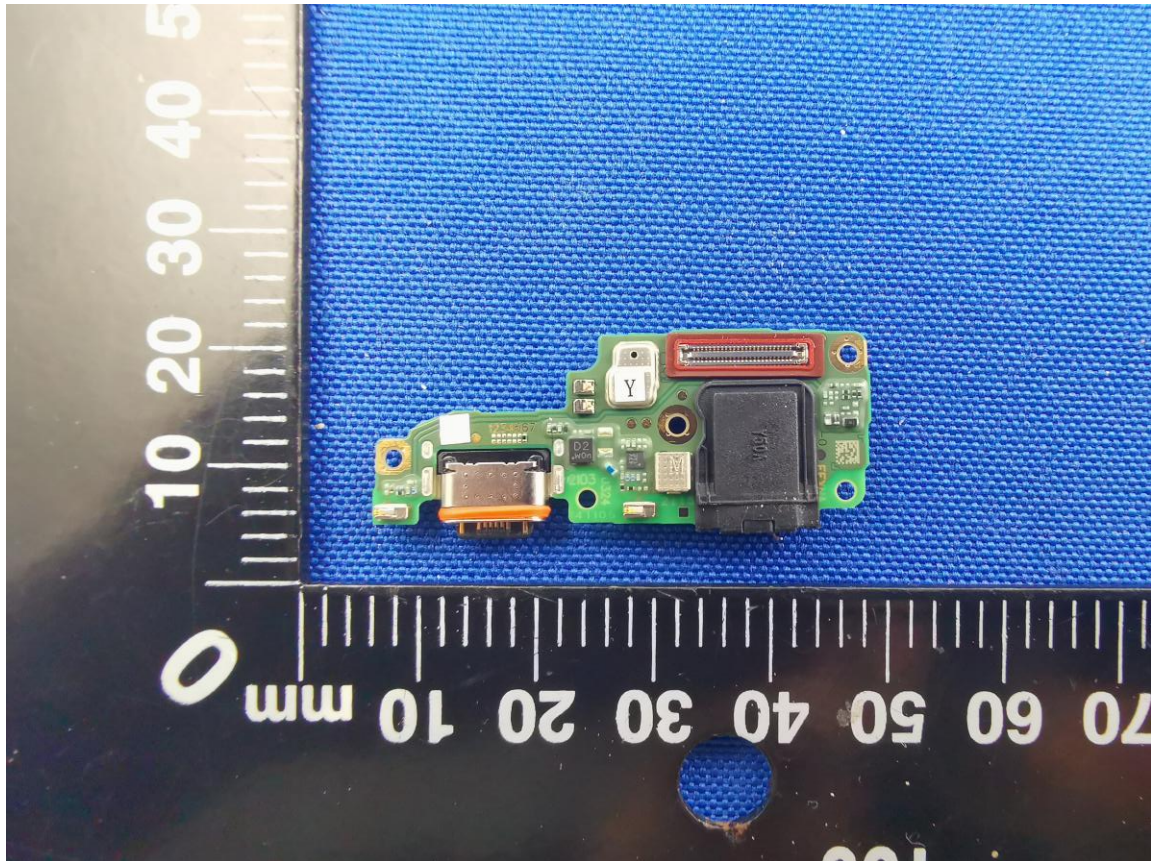
SUB BOARD BACK SIDE VIEW (WITH SHIELDING)
