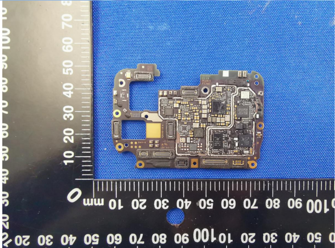
MAIN BOARD TOP VIEW (WITHOUT SHIELDING)
