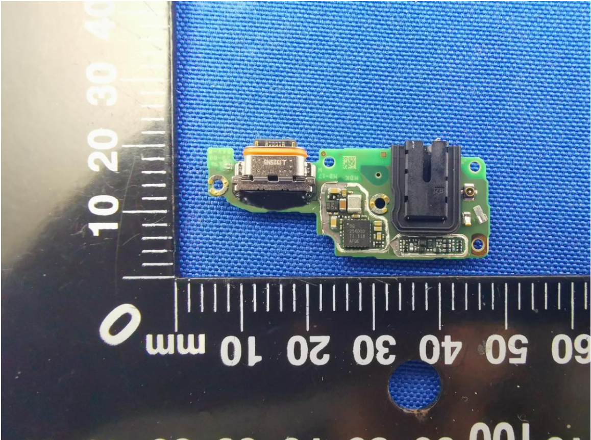
SUB BOARD TOP VIEW (WITHOUT SHIELDING)
