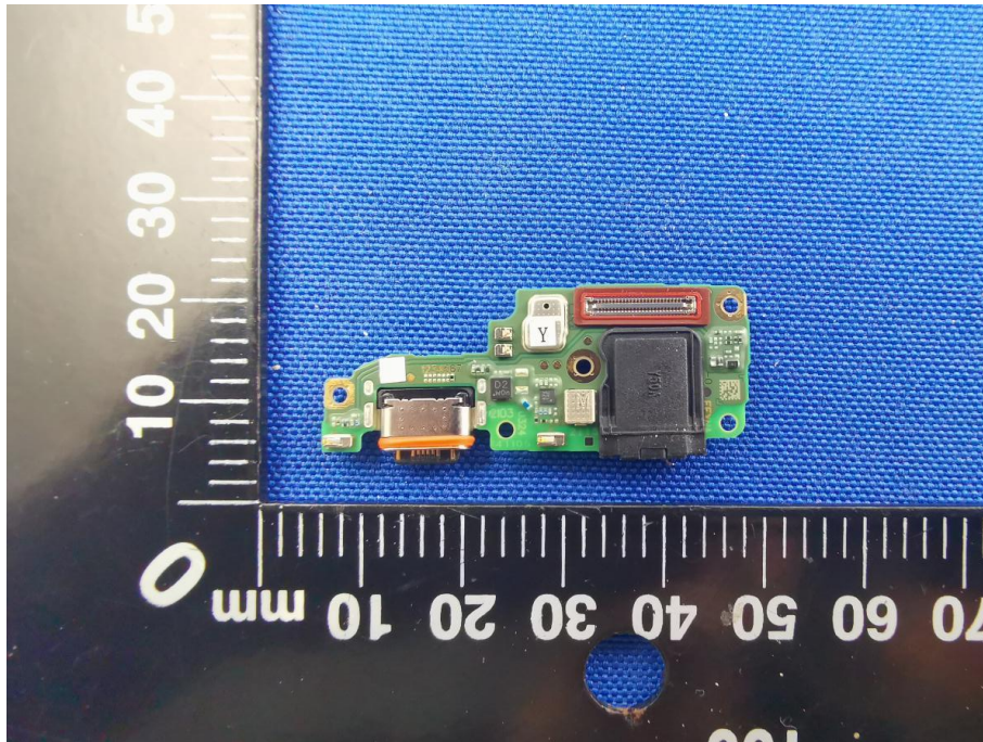
SUB BOARD BACK SIDE VIEW (WITH SHIELDING)
