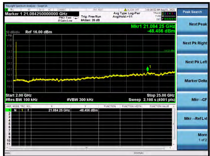
802.11n-20 CHANNEL 6, SPURIOUS 2 GHz ~ 25 GHz
