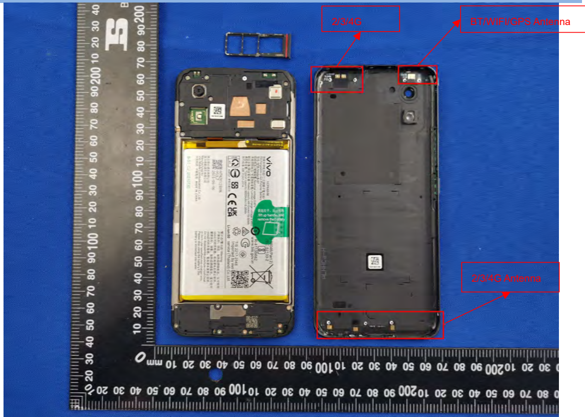
EUT UNCOVER VIEW
