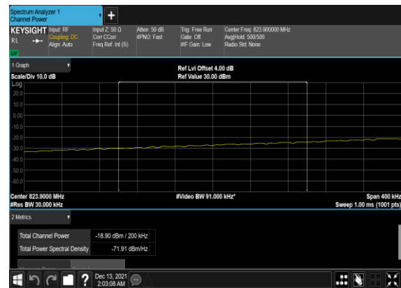
B7_N5(20M)_DFT-s- OFDM_BPSK_Edge_1RB_Left_Low_CH_CHP_PA SS
