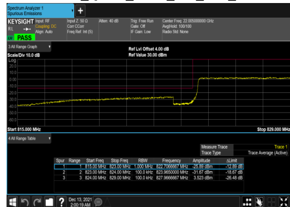
B7_N5(10M)_DFT-s- OFDM_QPSK_Outer_Full_Low_CH
