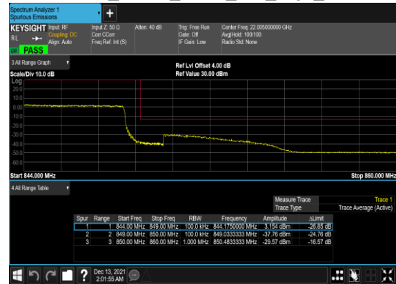
B7_N5(10M)_DFT-s- OFDM_QPSK_Outer_Full_High_CH
