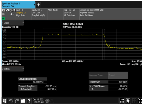
B7_N5(15M)_DFT-s-OFDM_PI_2- BPSK_Outer_Full_Mid_CH
