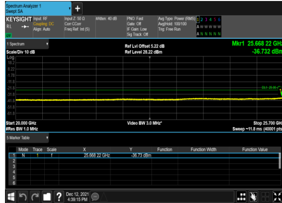
OFDM_BPSK_Edge_1RB_Left_Low_CH
