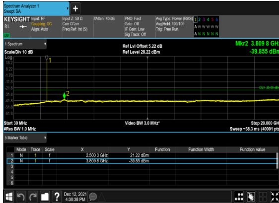
OFDM_BPSK_Edge_1RB_Left_Low_CH
