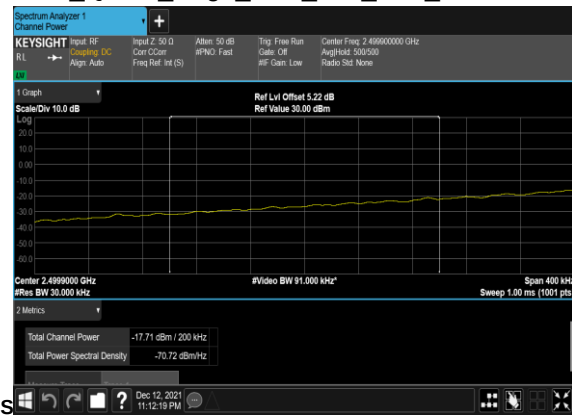
N7(10M)_DFT-s- OFDM_QPSK_Edge_1RB_Left_Low_CH_CHP_PAS
