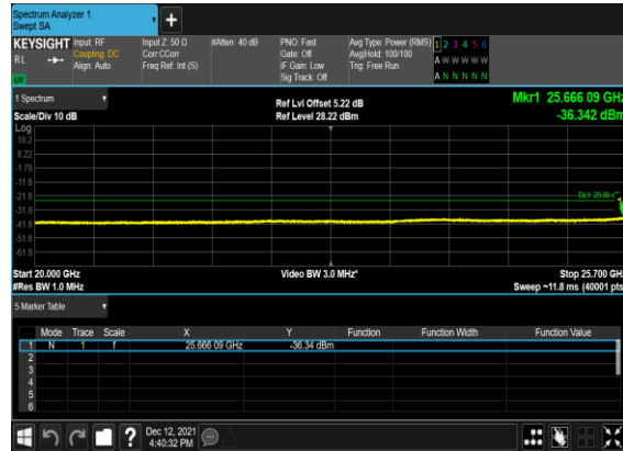
OFDM_QPSK_Edge_1RB_Left_Low_CH
