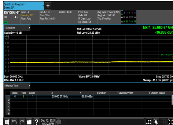
OFDM_QPSK_Edge_1RB_Left_Mid_CH
