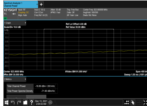
B7_N5(20M)_DFT-s- OFDM_QPSK_Edge_1RB_Left_Low_CH_CHP_PA SS
