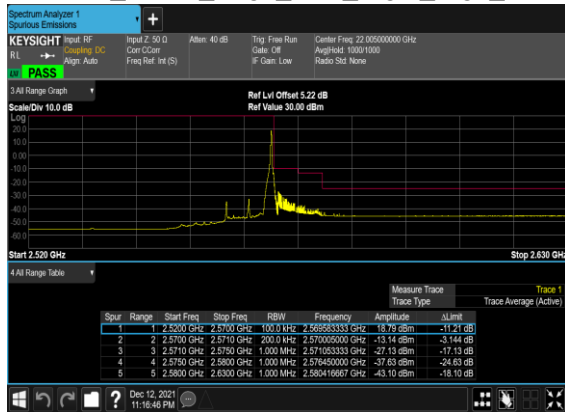
N7(10M)_DFT-s- OFDM_QPSK_Edge_1RB_Right_High_CH
