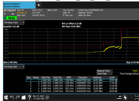
N7(10M)_DFT-s- OFDM_BPSK_Outer_Full_Low_CH
