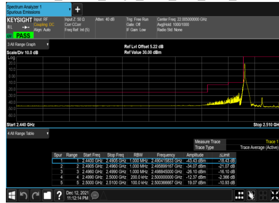
N7(10M)_DFT-s- OFDM_QPSK_Edge_1RB_Left_Low_CH
