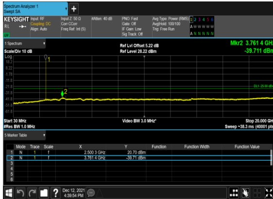
OFDM_QPSK_Edge_1RB_Left_Low_CH
