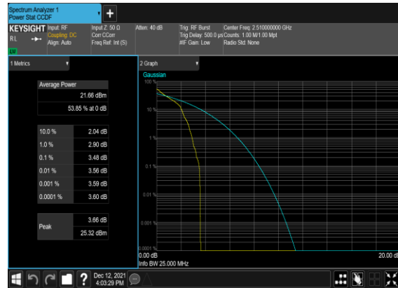
N7(20M)_DFT-s-OFDM_PI_2- BPSK_Edge_1RB_Left_Low_CH
