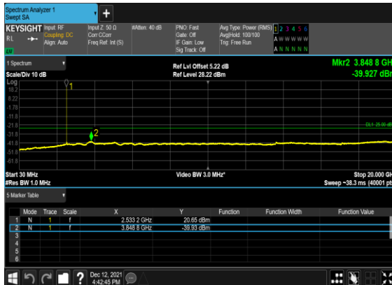
OFDM_QPSK_Edge_1RB_Left_Mid_CH
