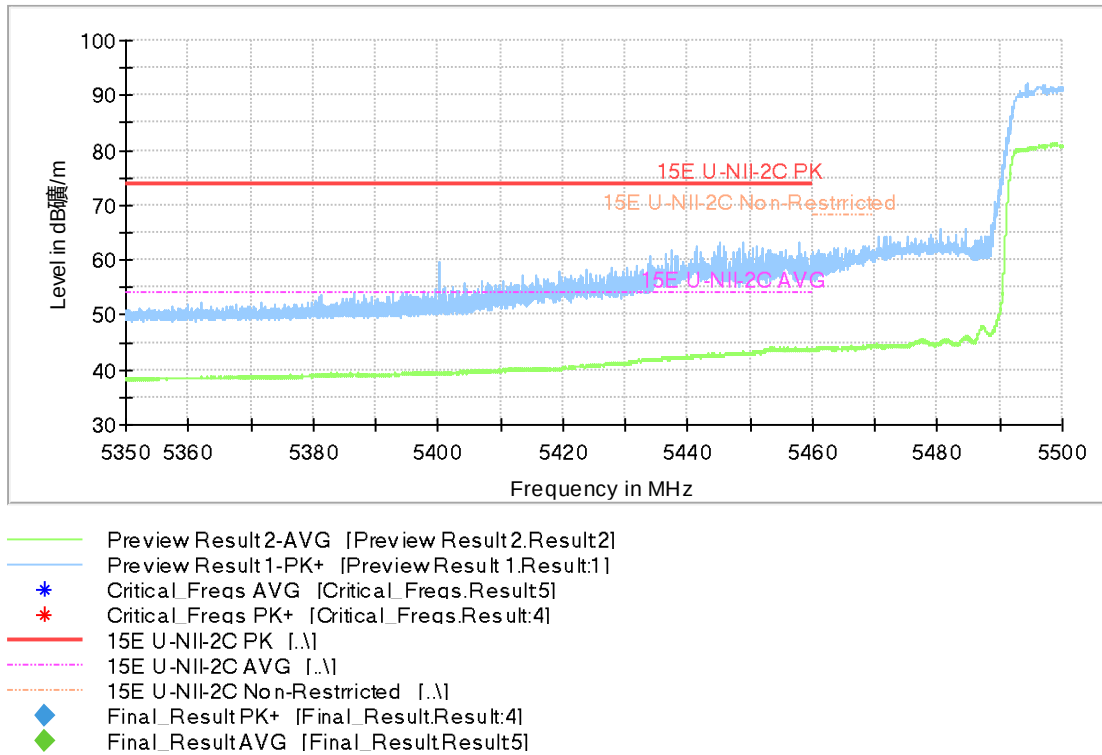
Fig.56 Band Edges (802.11ac-HT80, 5530MHz)
