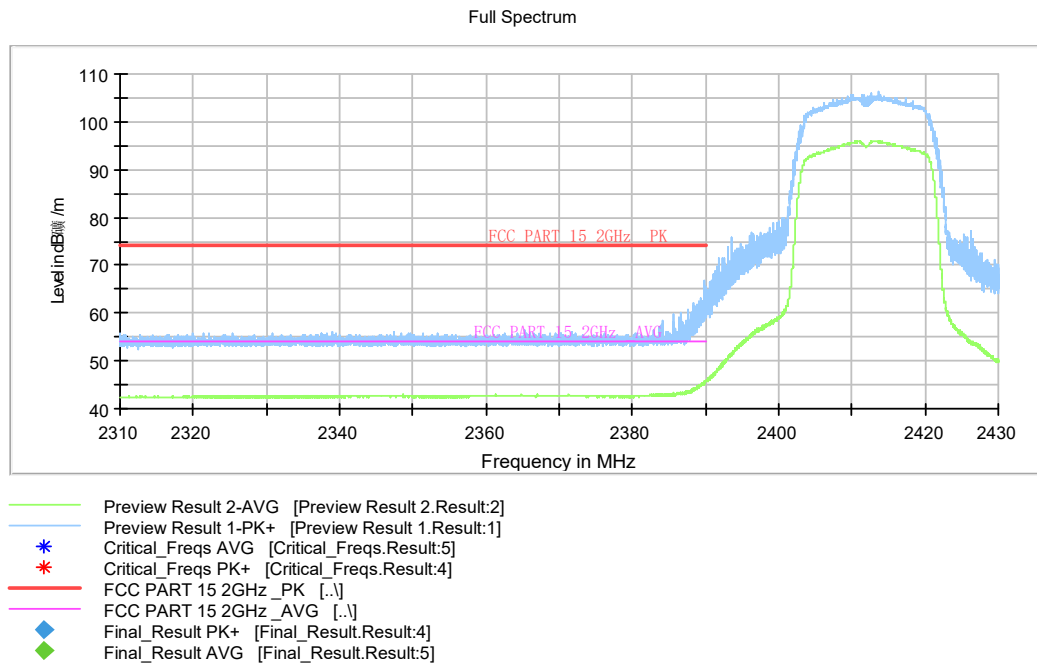
Fig.A.5.2.5 Radiated band Edges (802.11n-HT20, Ch 1)
