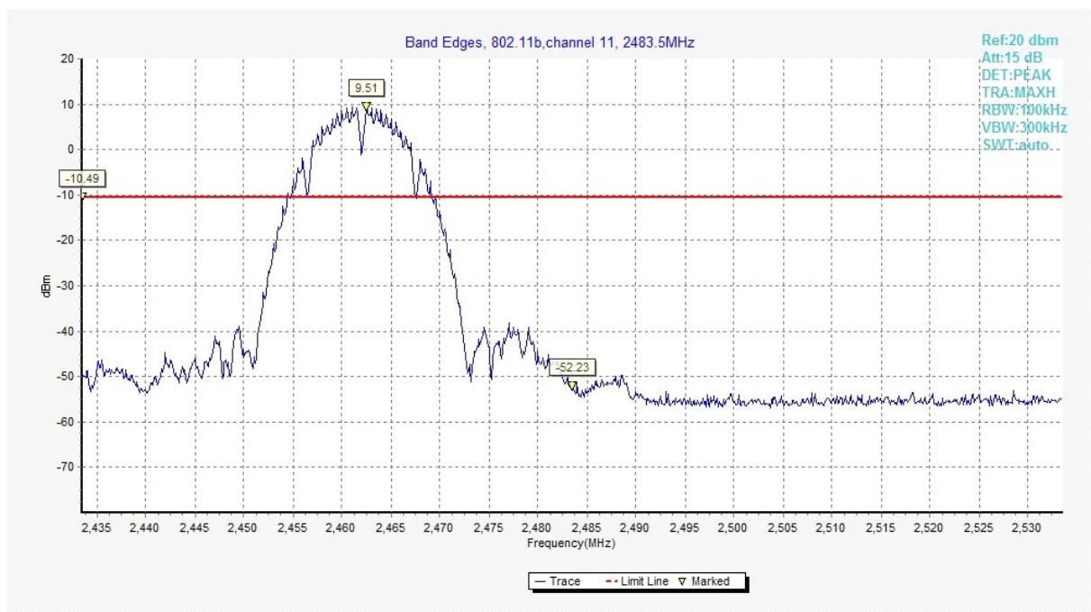
Fig.A.5.1.2 Band Edges (802.11b, Ch 11)
