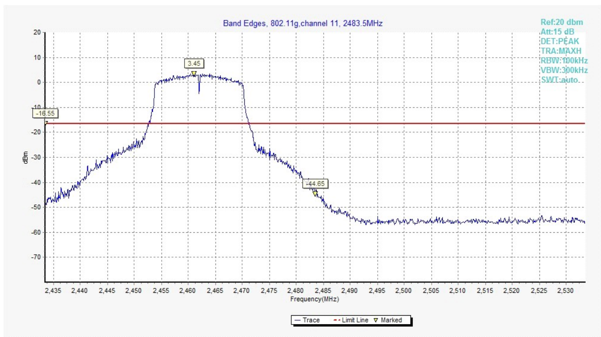
Fig.A.5.1.4 Band Edges (802.11g, Ch 11)
