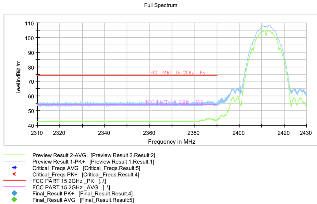
Fig.A.5.2.1 Radiated band Edges (802.11b, Ch 1)
