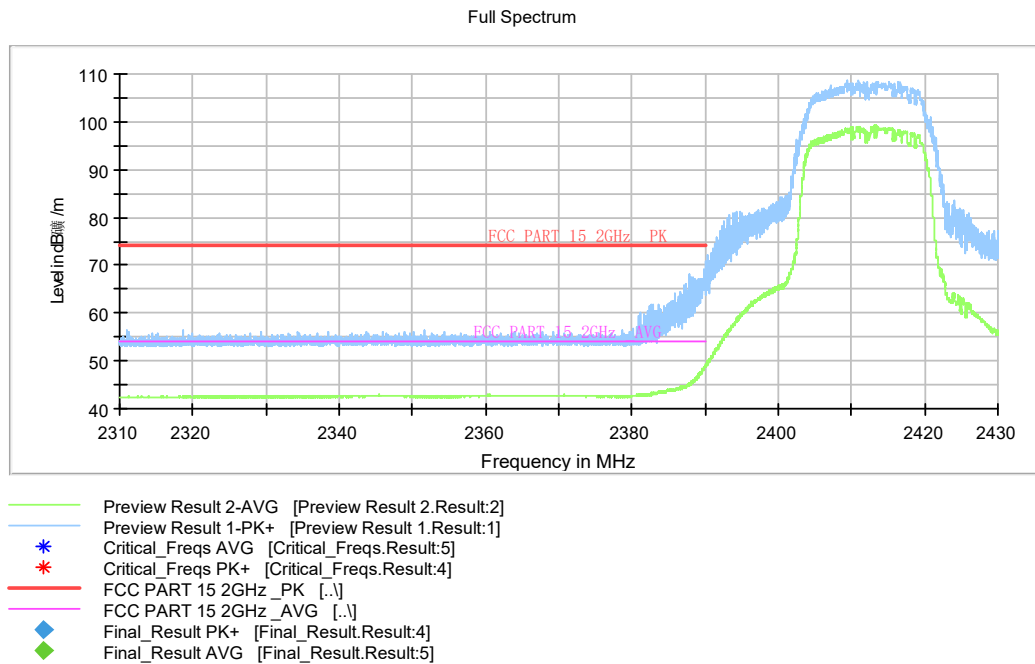
Fig.A.5.2.3 Radiated band Edges (802.11g, Ch 1)
