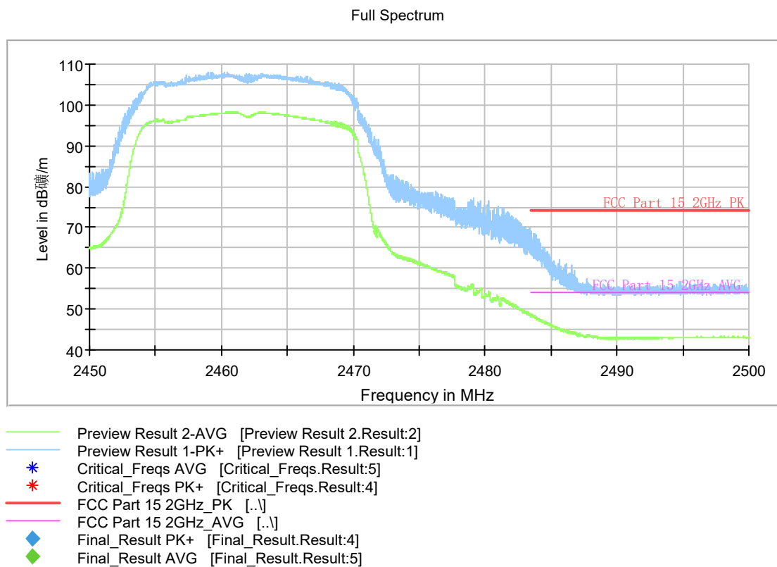
Fig.A.5.2.4 Radiated band Edges (802.11g, Ch 11)
