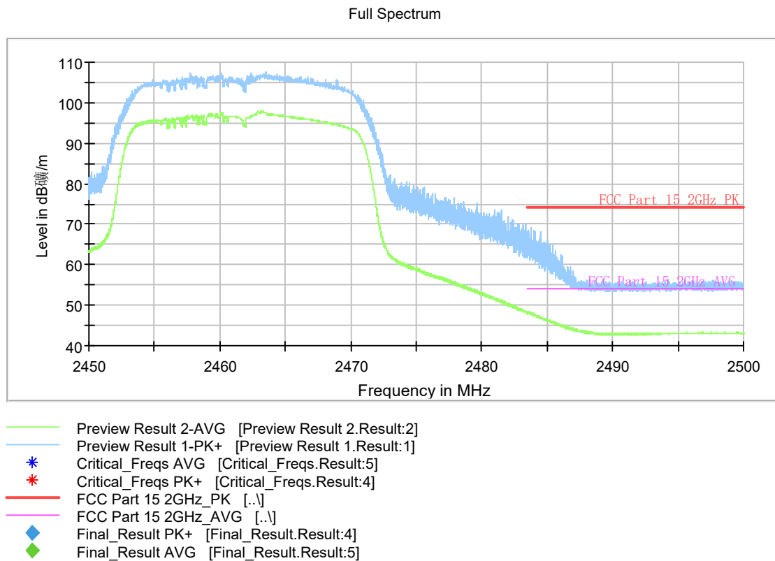
Fig.A.5.2.6 Radiated band Edges (802.11n-HT20, Ch 11)
