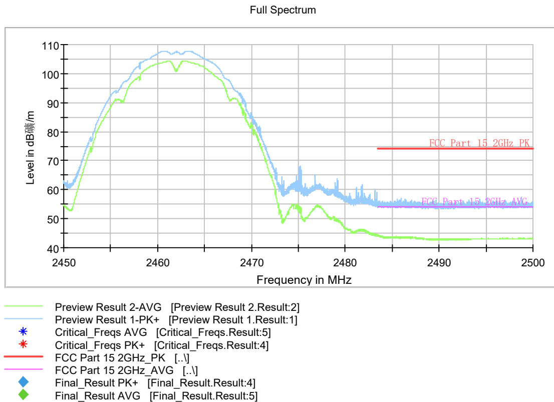
Fig.A.5.2.2 Radiated band Edges (802.11b, Ch 11)
