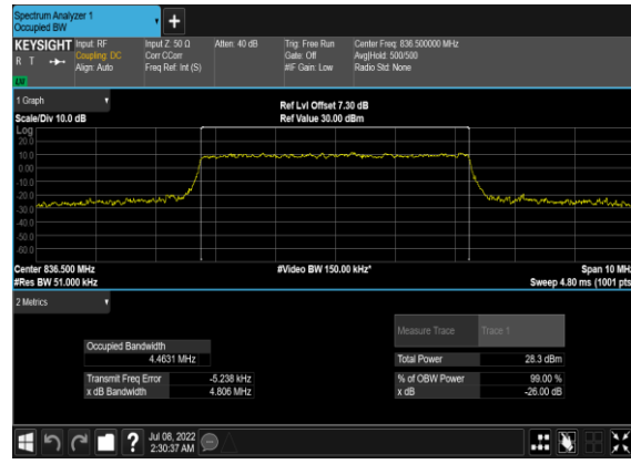
N5(5M)_CP-OFDM_16 QAM_Outer_Full_Mid_CH
