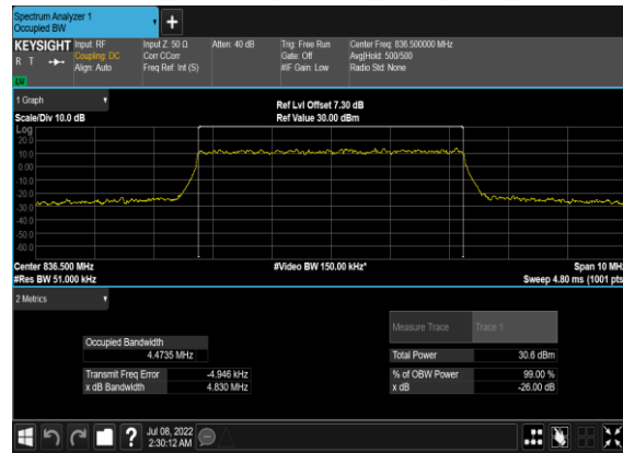
N5(5M)_DFT-s- OFDM_QPSK_Outer_Full_Mid_CH
