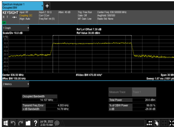
N5(15M)_CP- OFDM_QPSK_Outer_Full_Mid_CH
