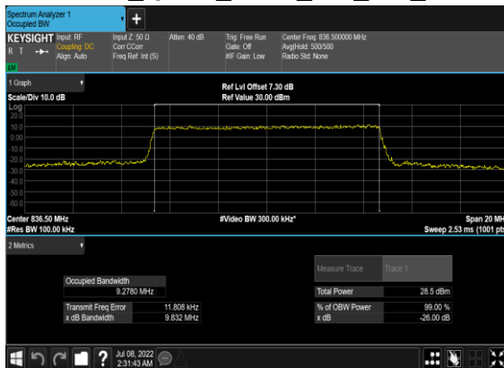
N5(10M)_CP-OFDM_QPSK_Outer_Full_Mid_CH
