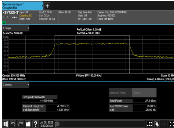
N5(5M)_CP-OFDM_- QPSK_Outer_Full_Mid_CH
