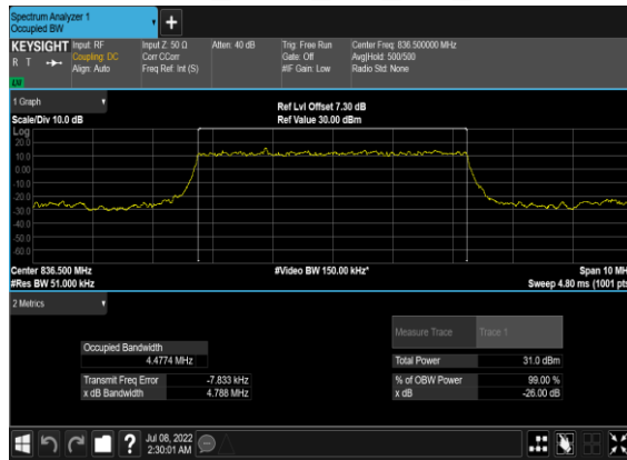
N5(5M)_DFT-s-OFDM_PI_2- BPSK_Outer_Full_Mid_CH
