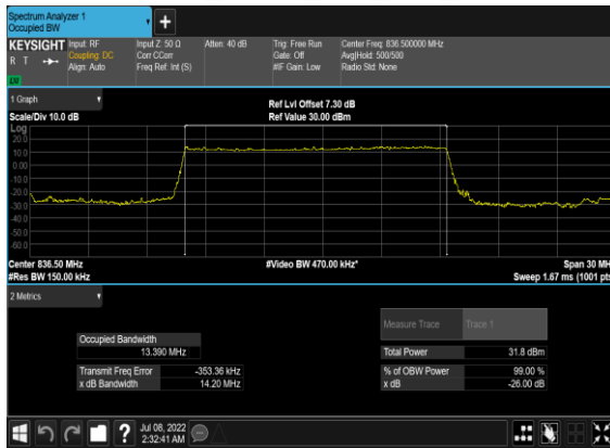
N5(15M)_DFT-s-OFDM_PI_2- BPSK_Outer_Full_Mid_CH
