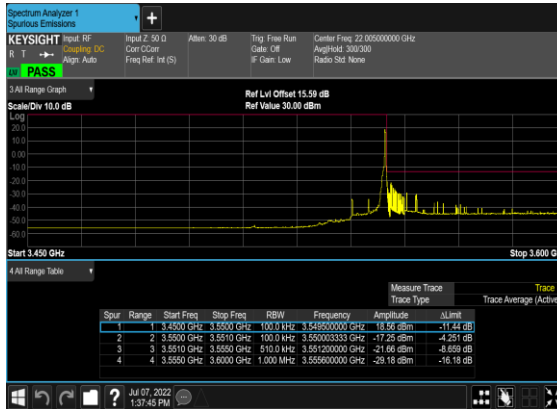
N78(10M)_DFT-s- OFDM_BPSK_Edge_1RB_Right_High_CH
