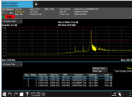
N78(20M)_DFT-s- OFDM_QPSK_Edge_1RB_Right_High_CH
