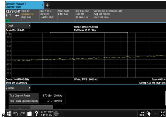
N78(20M)_DFT-s- OFDM_QPSK_Edge_1RB_Left_Low_CH_chp_pas
