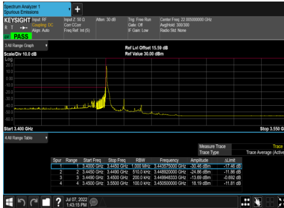
N78(20M)_DFT-s- OFDM_QPSK_Edge_1RB_Left_Low_CH
