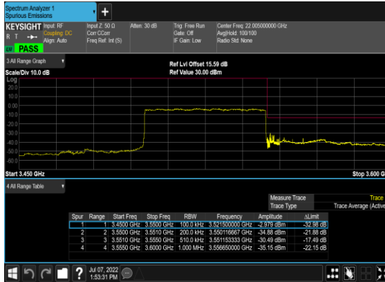
N78(50M)_DFT-s- OFDM_BPSK_Outer_Full_High_CH
