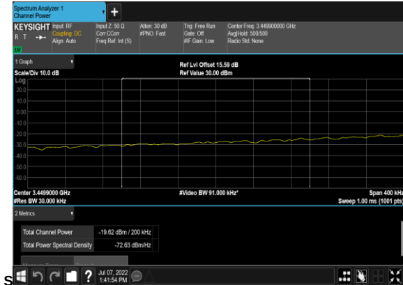
N78(20M)_DFT-s- OFDM_BPSK_Edge_1RB_Left_Low_CH_chp_pas
