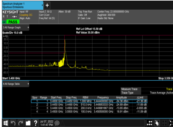
N78(20M)_DFT-s- OFDM_BPSK_Edge_1RB_Left_Low_CH
