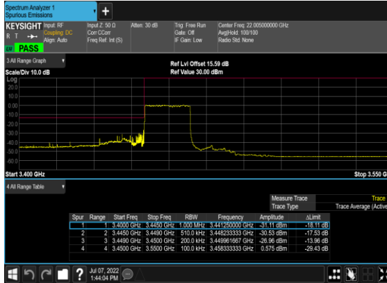
N78(20M)_DFT-s- OFDM_BPSK_Outer_Full_Low_CH
