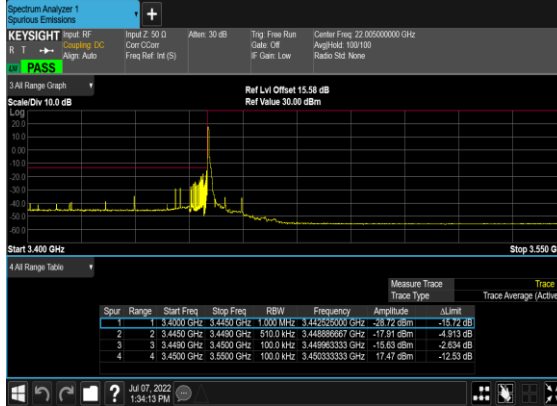
N78(10M)_DFT-s- OFDM_BPSK_Edge_1RB_Left_Low_CH
