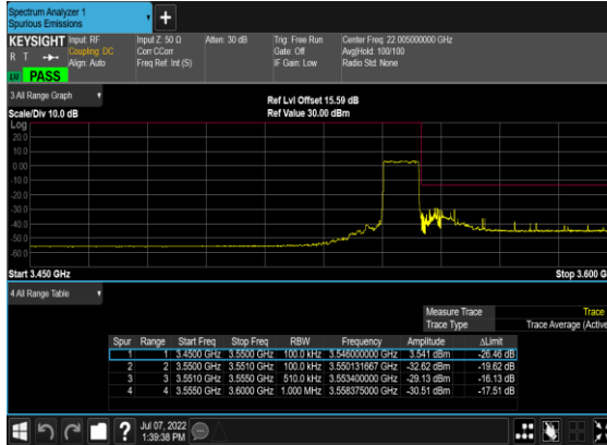
N78(10M)_DFT-s- OFDM_BPSK_Outer_Full_High_CH
