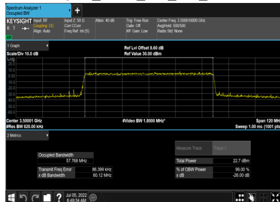
N78(60M)_CP-OFDM_256 QAM_Outer_Full_Mid_CH
