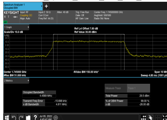
N66(5M)_DFT-s- OFDM_QPSK_Outer_Full_Mid_CH
