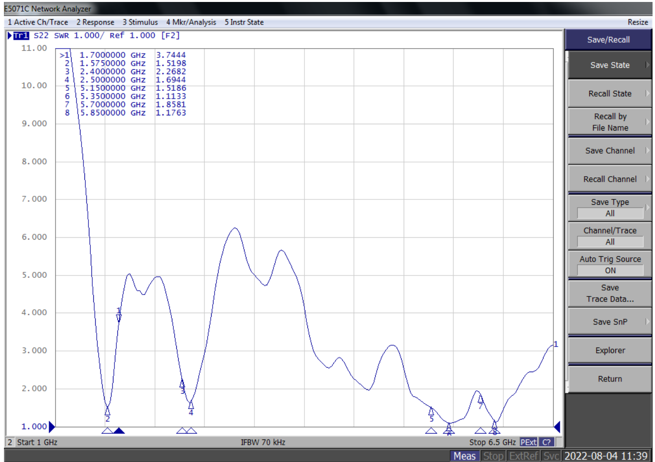
ANT22# VSWR
