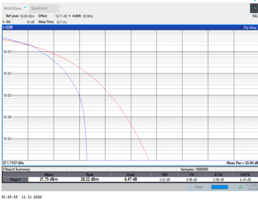
Band66-1.4MHz-16QAM-131979-6RB#0
