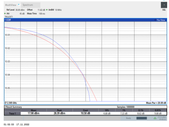
Band41-15MHz-64QAM-40640-75RB#0
