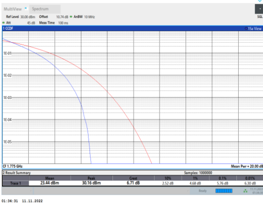
Band66-10MHz-QPSK-132622-50RB#0
