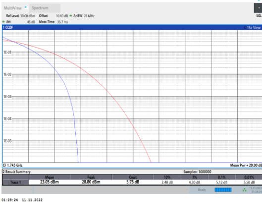
Band66-3MHz-QPSK-132322-15RB#0
