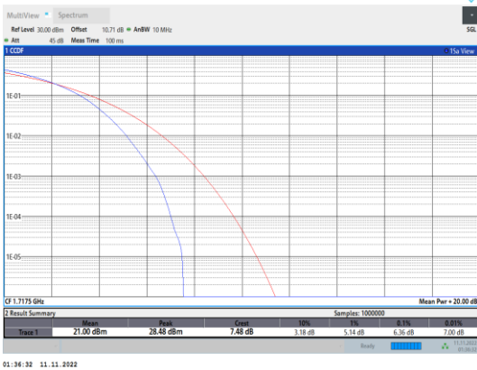
Band66-15MHz-16QAM-132047-75RB#0
