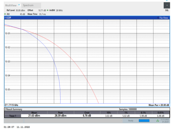
Band66-3MHz-16QAM-131987-15RB#0
