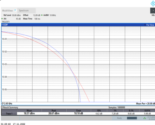
Band41-10MHz-64QAM-41190-50RB#0
