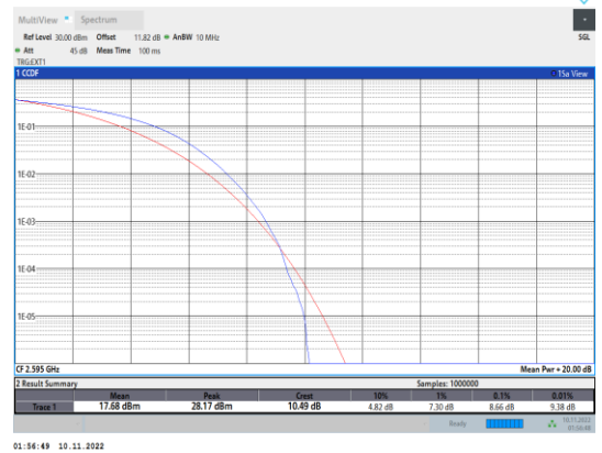
Band41-20MHz-16QAM-40640-100RB#0
