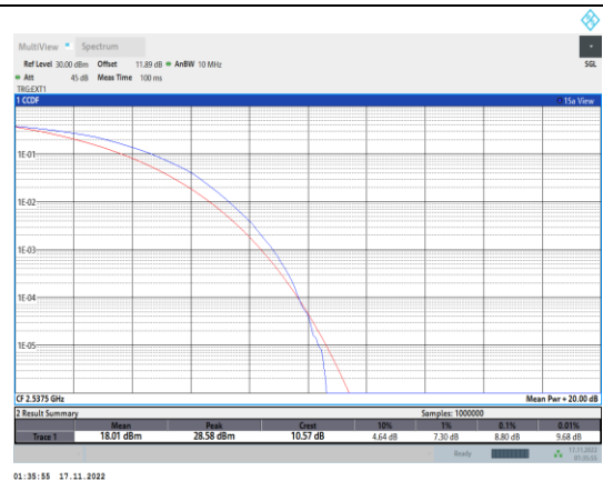
Band41-5MHz-64QAM-40065-25RB#0
