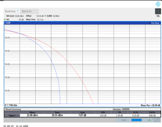
Band66-3MHz-16QAM-132657-15RB#0
