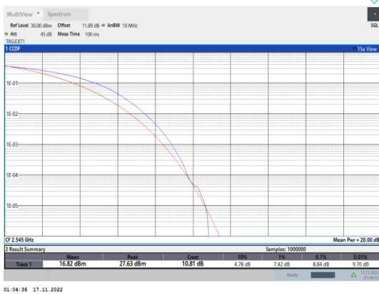
Band41-20MHz-64QAM-40140-100RB#0
