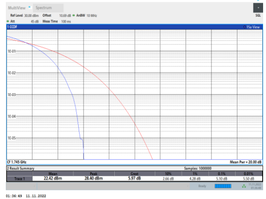
Band66-15MHz-QPSK-132322-75RB#0
