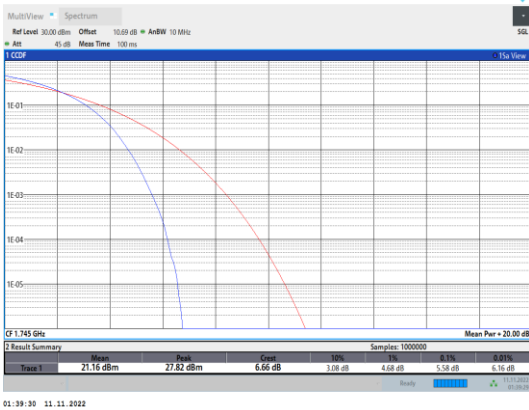
Band66-20MHz-QPSK-132322-100RB#0
