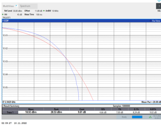
Band41-15MHz-16QAM-40115-75RB#0
