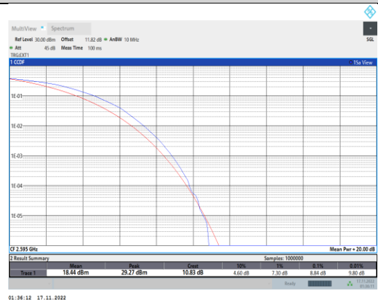
Band41-5MHz-64QAM-40640-25RB#0
