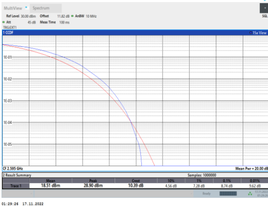
Band41-10MHz-64QAM-40640-50RB#0
