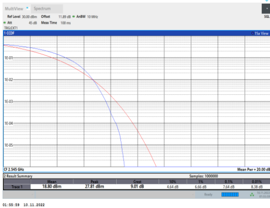
Band41-20MHz-QPSK-40140-100RB#0
