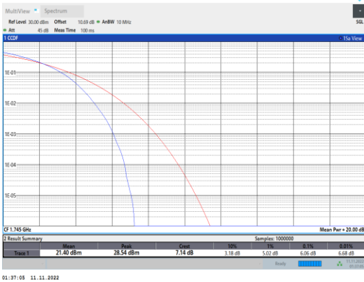
Band66-15MHz-16QAM-132322-75RB#0
