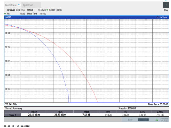
Band66-15MHz-64QAM-132322-75RB#0
