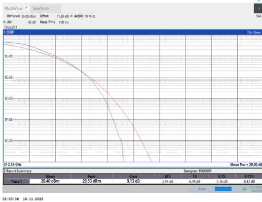
Band41-10MHz-QPSK-40090-50RB#0
