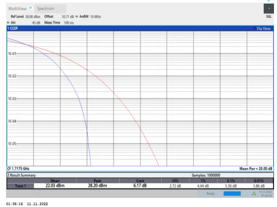
Band66-15MHz-QPSK-132047-75RB#0
