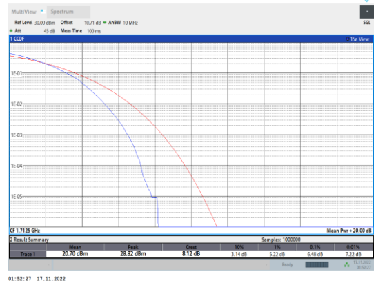
Band66-5MHz-64QAM-131997-25RB#0
