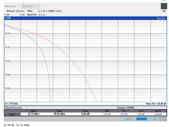
Band66-1.4MHz-QPSK-131979-6RB#0
