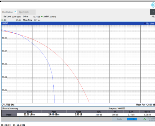
Band66-1.4MHz-16QAM-132665-6RB#0
