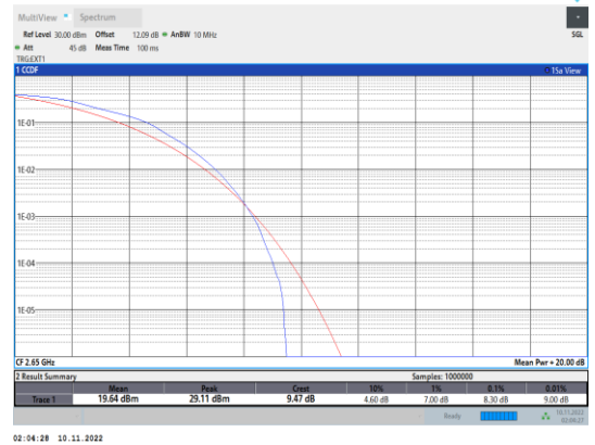
Band41-10MHz-16QAM-41190-50RB#0
