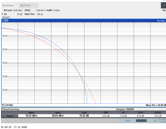
Band41-10MHz-64QAM-40090-50RB#0
