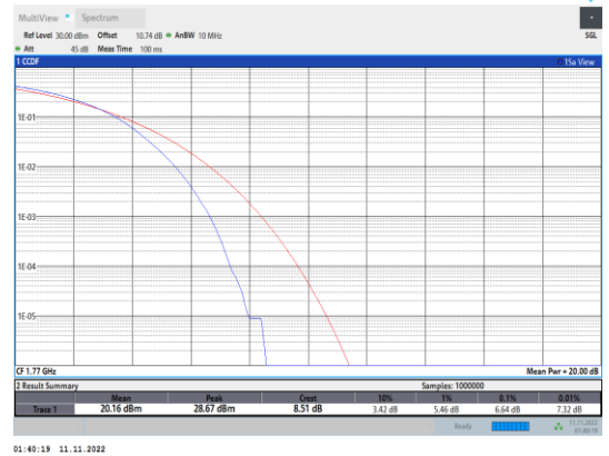
Band66-20MHz-16QAM-132572-100RB#0
