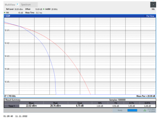
Band66-3MHz-16QAM-132322-15RB#0
