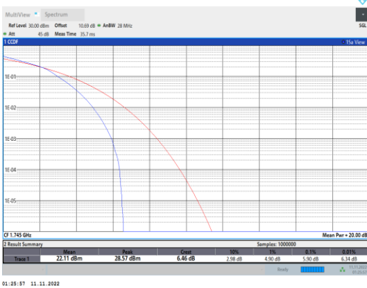
Band66-1.4MHz-16QAM-132322-6RB#0
