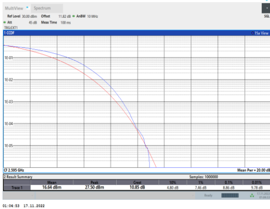
Band41-20MHz-64QAM-40640-100RB#0
