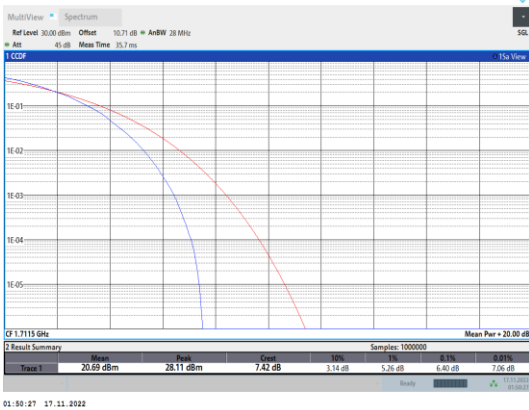
Band66-3MHz-64QAM-131987-15RB#0
