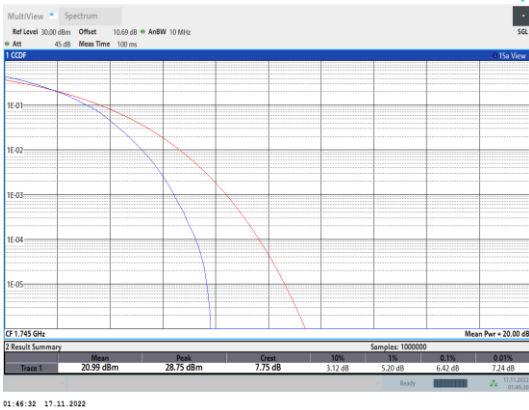
Band66-10MHz-64QAM-132322-50RB#0
