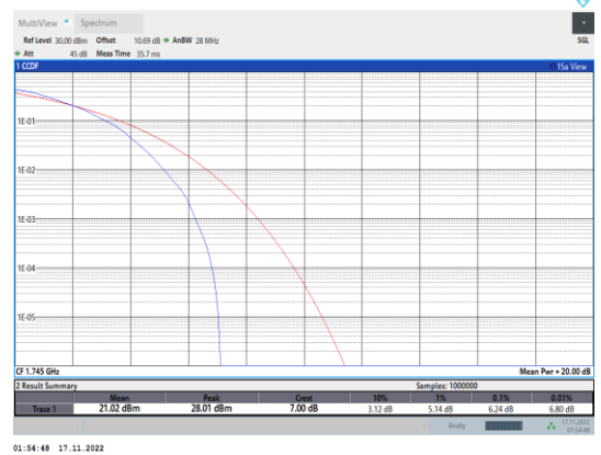
Band66-1.4MHz-64QAM-132322-6RB#0
