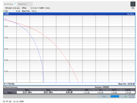
Band66-15MHz-QPSK-132597-75RB#0
