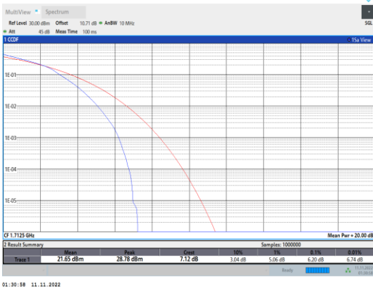
Band66-5MHz-16QAM-131997-25RB#0
