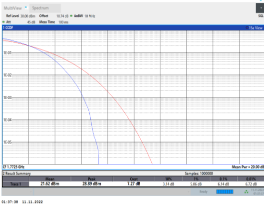
Band66-15MHz-16QAM-132597-75RB#0
