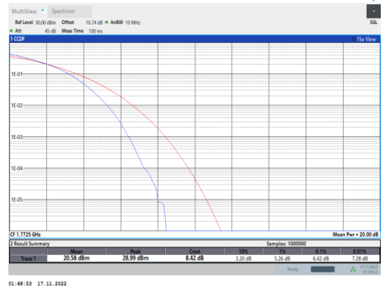
Band66-15MHz-64QAM-132597-75RB#0
