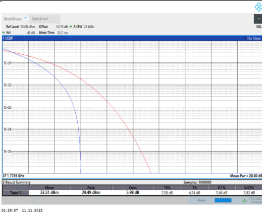
Band66-3MHz-QPSK-132657-15RB#0
