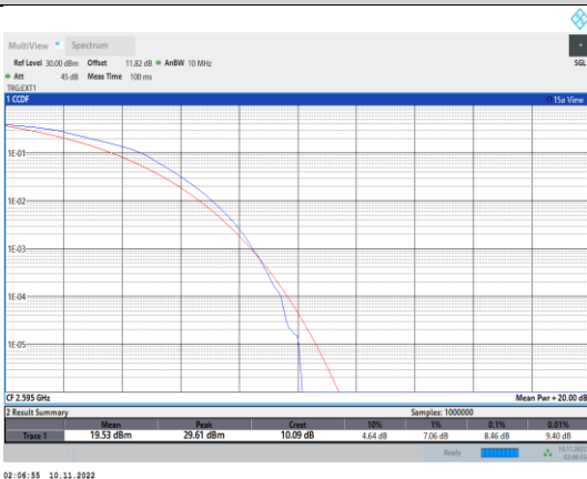
Band41-5MHz-16QAM-40640-25RB#0
