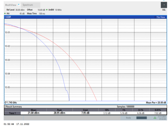
Band66-5MHz-64QAM-132322-25RB#0
