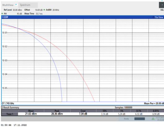
Band66-3MHz-64QAM-132322-15RB#0
