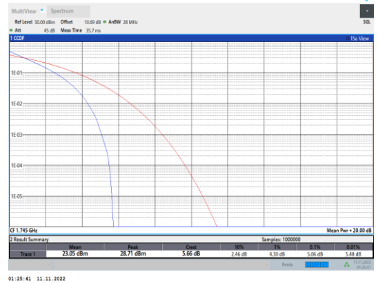
Band66-1.4MHz-QPSK-132322-6RB#0
