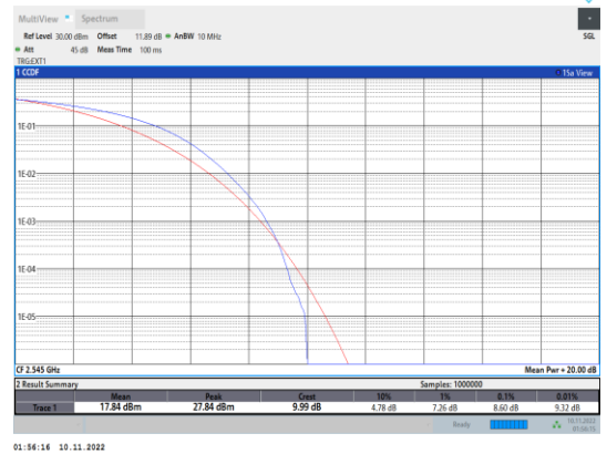
Band41-20MHz-16QAM-40140-100RB#0
