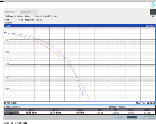
Band41-5MHz-64QAM-41215-25RB#0
