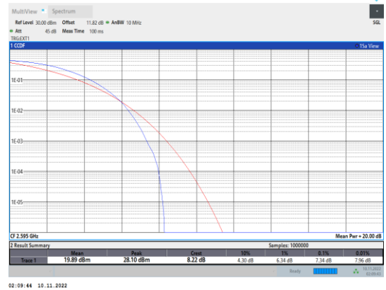
Band41-15MHz-QPSK-40640-75RB#0
