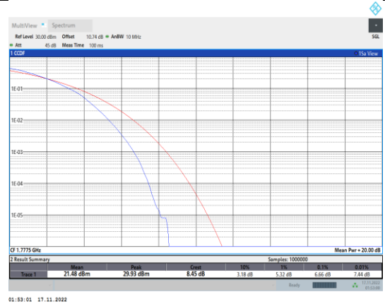
Band66-5MHz-64QAM-132647-25RB#0
