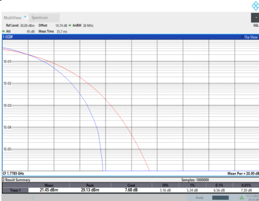
Band66-3MHz-64QAM-132657-15RB#0
