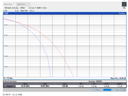
Band66-10MHz-16QAM-132622-50RB#0
