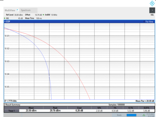
Band66-5MHz-QPSK-132647-25RB#0
