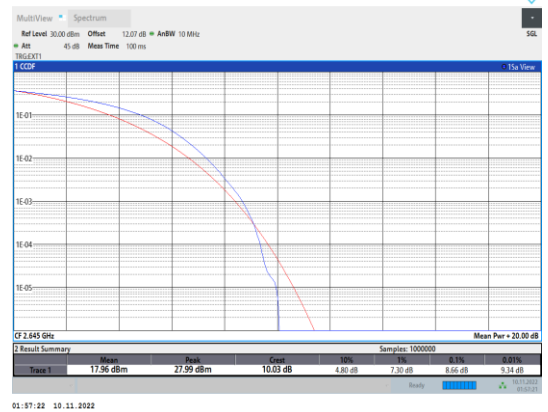
Band41-20MHz-16QAM-41140-100RB#0
