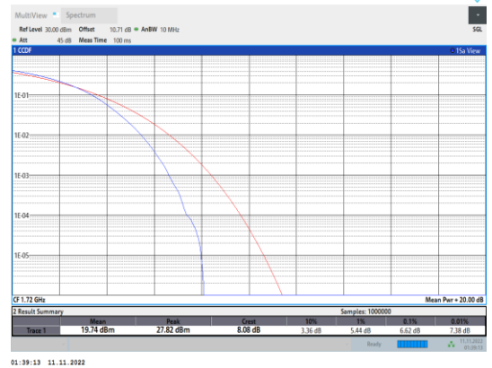
Band66-20MHz-16QAM-132072-100RB#0
