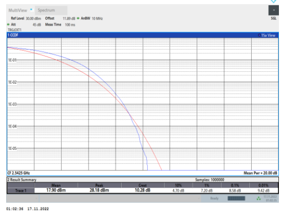
Band41-15MHz-64QAM-40115-75RB#0
