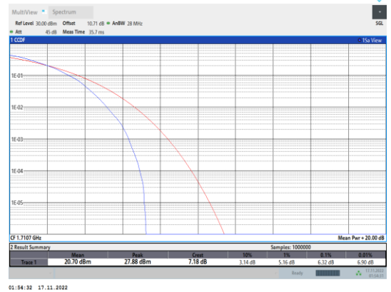
Band66-1.4MHz-64QAM-131979-6RB#0
