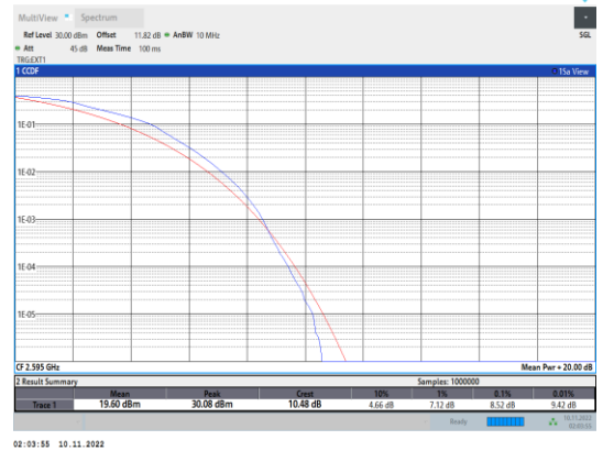
Band41-10MHz-16QAM-40640-50RB#0
