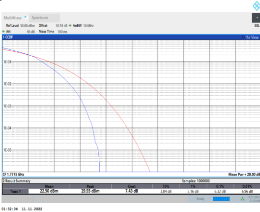
Band66-5MHz-16QAM-132647-25RB#0
