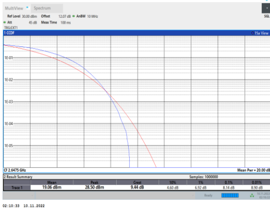
Band41-15MHz-16QAM-41165-75RB#0
