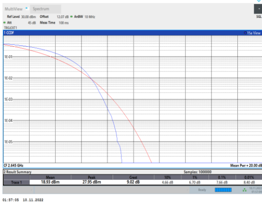
Band41-20MHz-QPSK-41140-100RB#0
