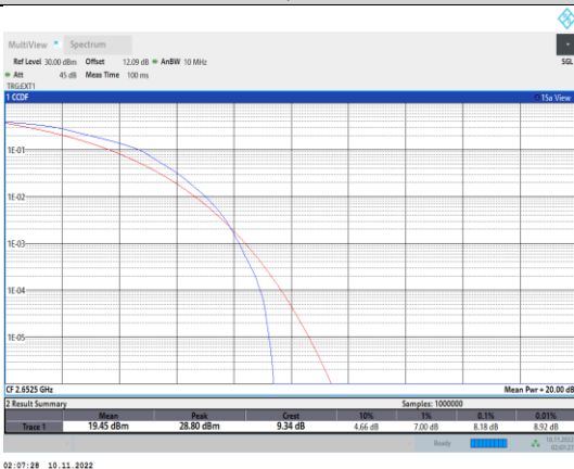
Band41-5MHz-16QAM-41215-25RB#0
