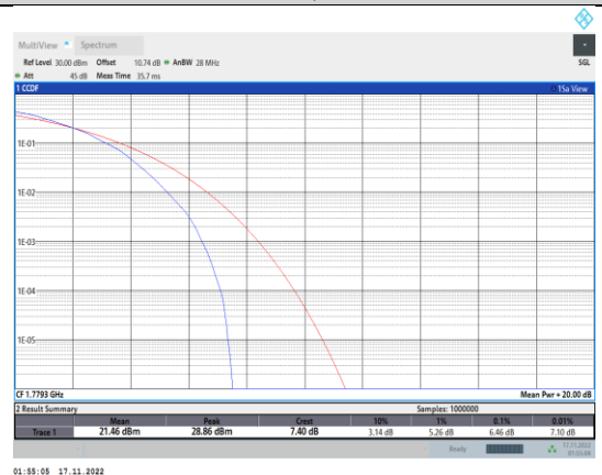
Band66-1.4MHz-64QAM-132665-6RB#0
