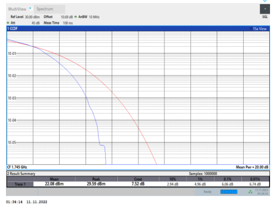
Band66-10MHz-16QAM-132322-50RB#0
