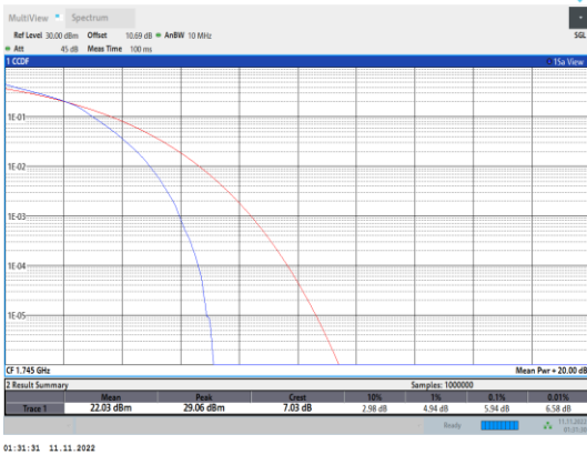
Band66-5MHz-16QAM-132322-25RB#0
