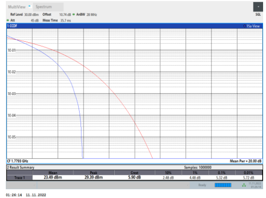
Band66-1.4MHz-QPSK-132665-6RB#0
