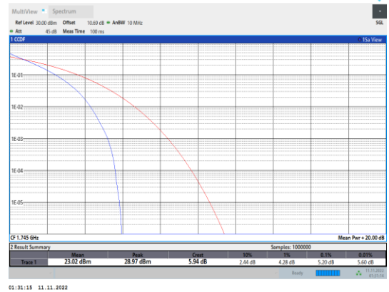
Band66-5MHz-QPSK-132322-25RB#0
