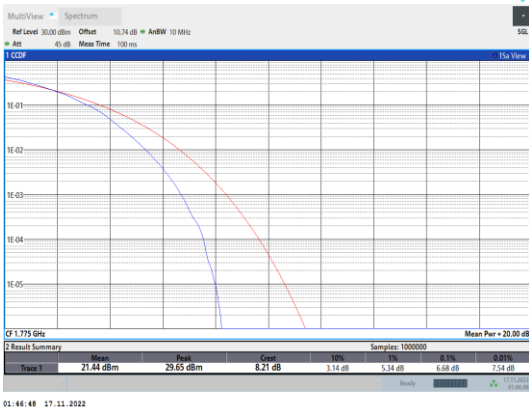
Band66-10MHz-64QAM-132622-50RB#0
