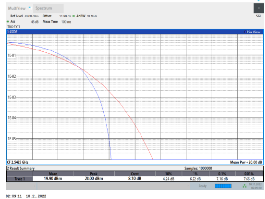
Band41-15MHz-QPSK-40115-75RB#0
