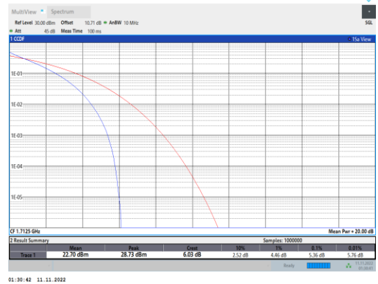
Band66-5MHz-QPSK-131997-25RB#0
