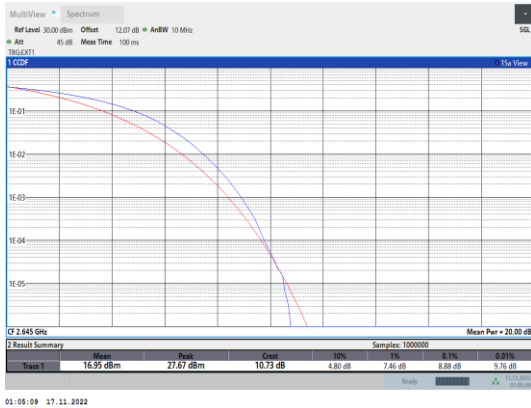
Band41-20MHz-64QAM-41140-100RB#0
