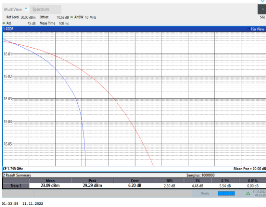
Band66-10MHz-QPSK-132322-50RB#0
