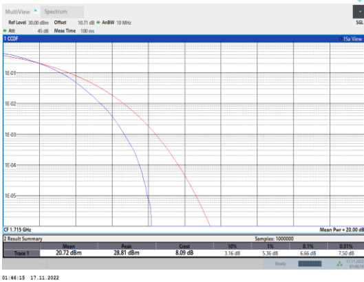
Band66-10MHz-64QAM-132022-50RB#0
