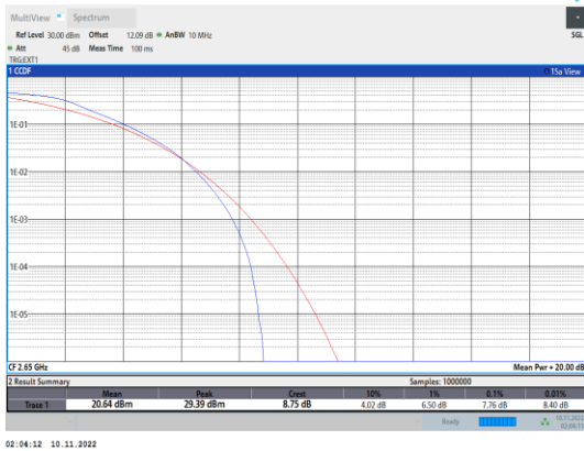
Band41-10MHz-QPSK-41190-50RB#0
