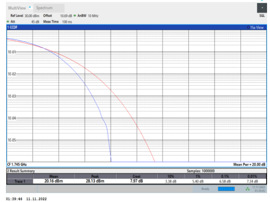
Band66-20MHz-16QAM-132322-100RB#0
