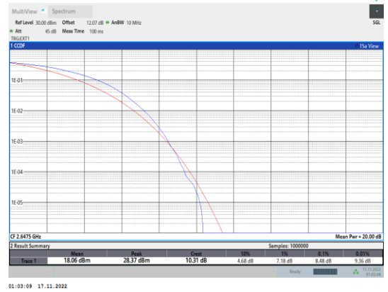
Band41-15MHz-64QAM-41165-75RB#0
