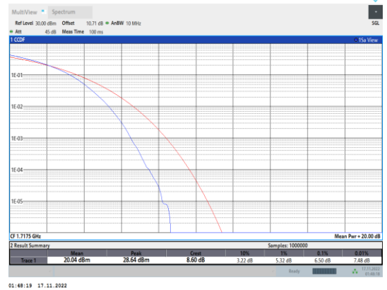
Band66-15MHz-64QAM-132047-75RB#0
