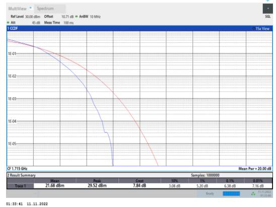
Band66-10MHz-16QAM-132022-50RB#0
