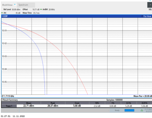
Band66-3MHz-QPSK-131987-15RB#0
