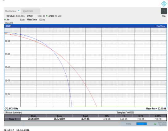
Band41-15MHz-QPSK-41165-75RB#0
