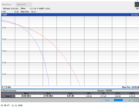
Band66-20MHz-QPSK-132072-100RB#0
