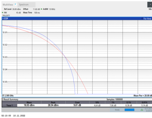
Band41-15MHz-16QAM-40640-75RB#0
