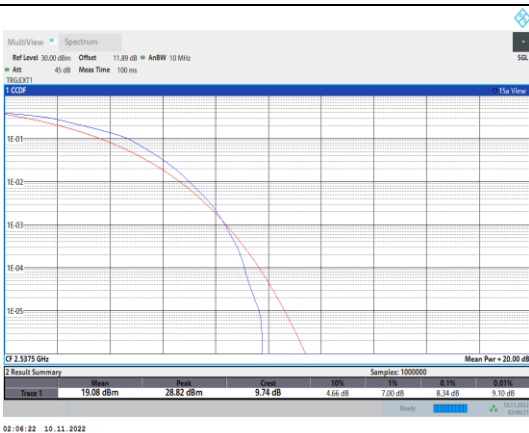
Band41-5MHz-16QAM-40065-25RB#0
