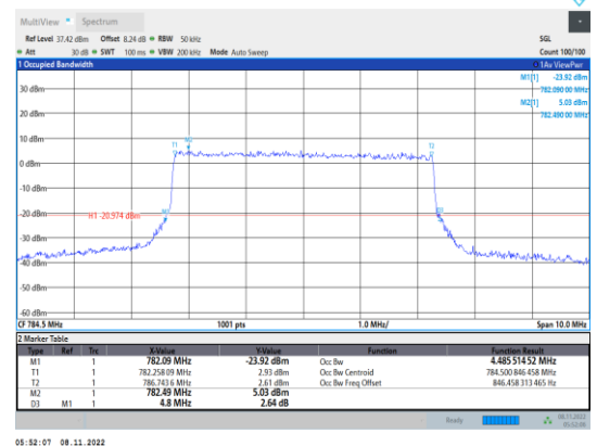
Band13-5MHz-16QAM-23255-25RB#0
