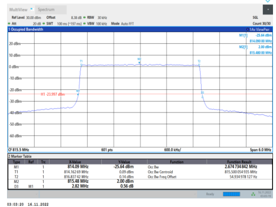
Band26-3MHz-64QAM-26705-15RB#0
