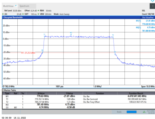
Band13-5MHz-64QAM-23230-25RB#0
