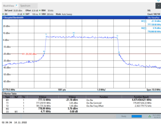
Band13-5MHz-64QAM-23205-25RB#0
