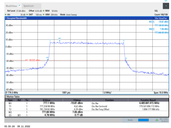
Band13-5MHz-16QAM-23205-25RB#0
