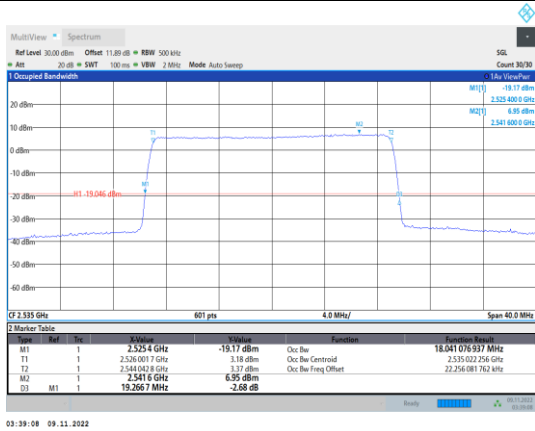
Band7-20MHz-16QAM-21100-100RB#0
