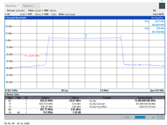
Band26-15MHz-64QAM-26865-75RB#0
