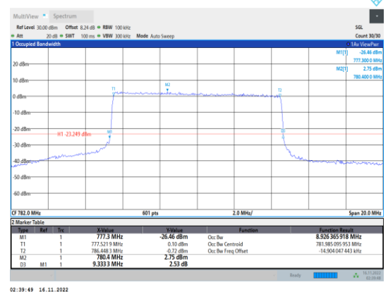
Band13-10MHz-64QAM-23230-50RB#0
