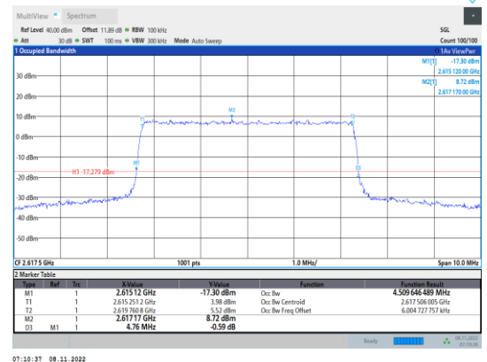
Band38-5MHz-16QAM-38225-25RB#0
