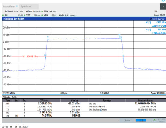
Band7-15MHz-64QAM-21100-75RB#0
