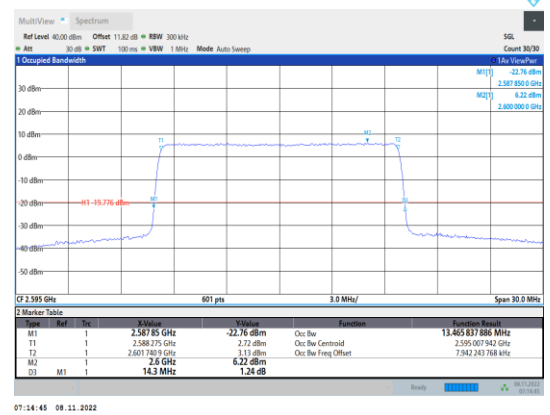
Band38-15MHz-16QAM-38000-75RB#0
