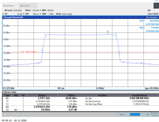
Band38-10MHz-16QAM-37800-50RB#0
