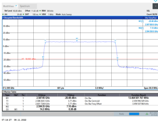
Band38-15MHz-QPSK-38000-75RB#0
