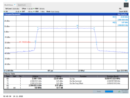
Band38-10MHz-64QAM-38000-50RB#0
