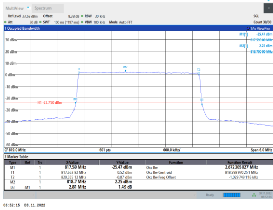
Band26-3MHz-16QAM-26740-15RB#0
