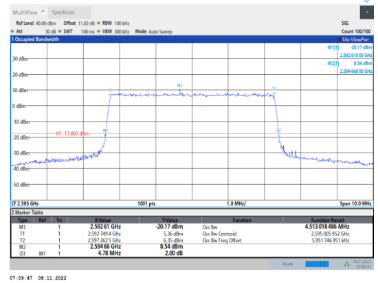
Band38-5MHz-16QAM-38000-25RB#0
