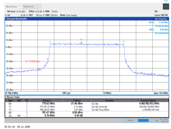
Band13-5MHz-16QAM-23230-25RB#0
