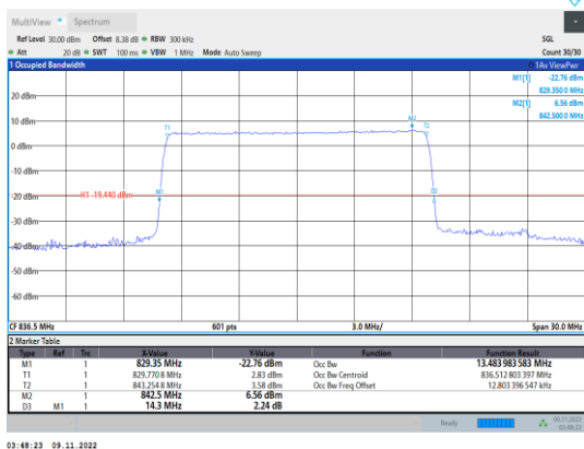
Band26-15MHz-QPSK-26915-75RB#0
