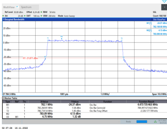
Band13-5MHz-64QAM-23255-25RB#0
