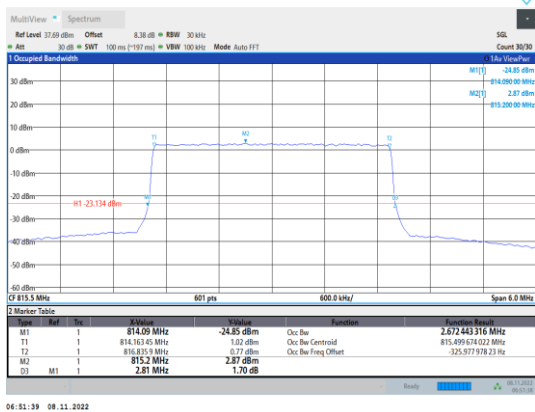
Band26-3MHz-16QAM-26705-15RB#0
