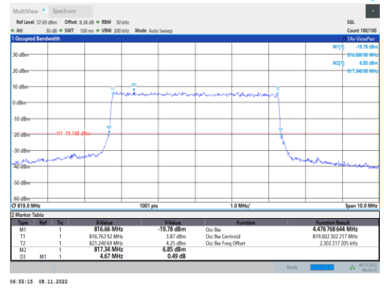
Band26-5MHz-16QAM-26740-25RB#0
