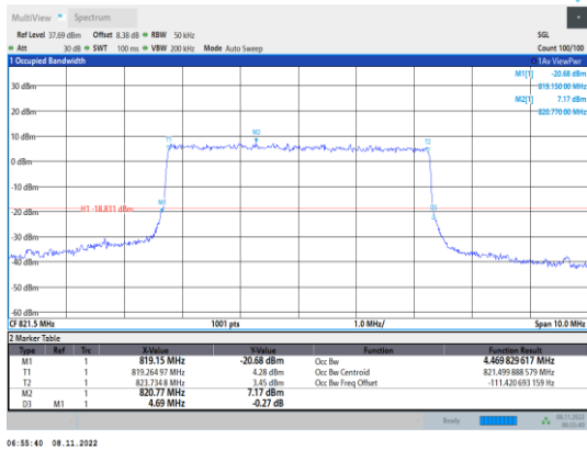
Band26-5MHz-QPSK-26765-25RB#0
