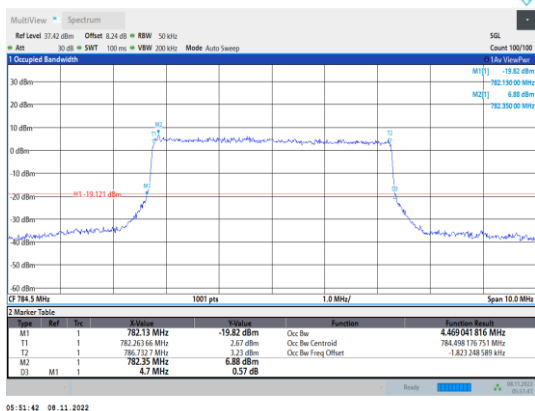
Band13-5MHz-QPSK-23255-25RB#0
