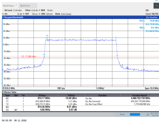
Band26-5MHz-QPSK-26715-25RB#0
