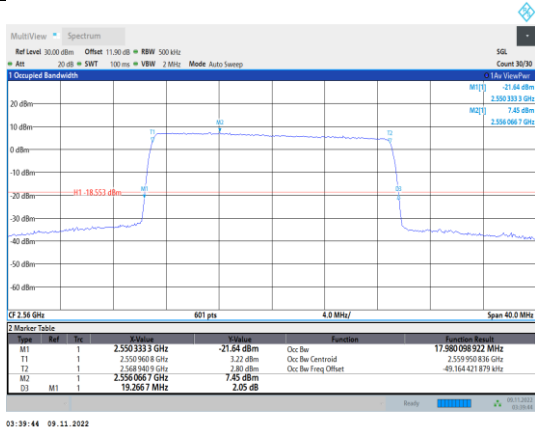
Band7-20MHz-16QAM-21350-100RB#0
