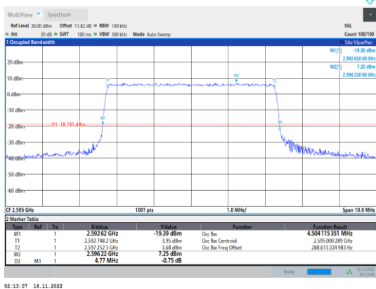
Band38-5MHz-64QAM-38000-25RB#0
