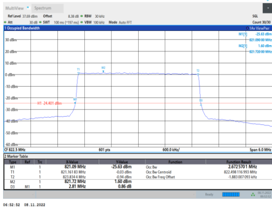
Band26-3MHz-16QAM-26775-15RB#0
