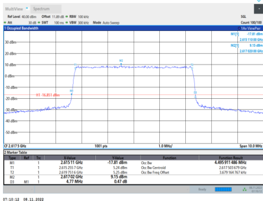
Band38-5MHz-QPSK-38225-25RB#0
