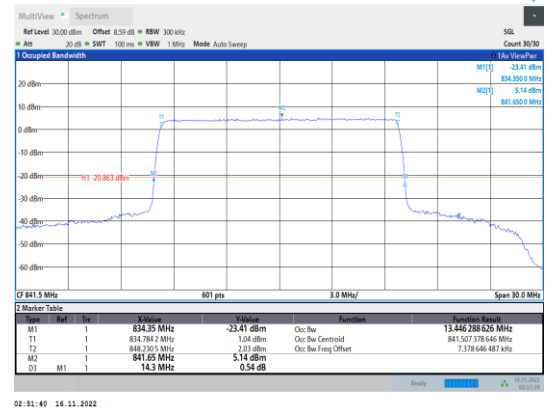
Band26-15MHz-64QAM-26965-75RB#0
