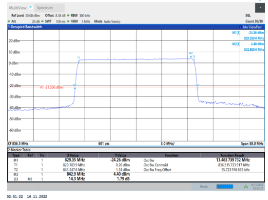
Band26-15MHz-64QAM-26915-75RB#0
