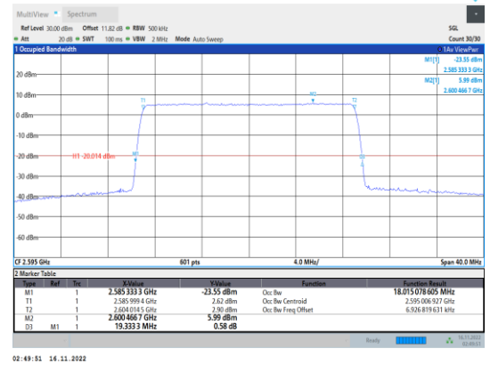
Band38-20MHz-64QAM-38000-100RB#0
