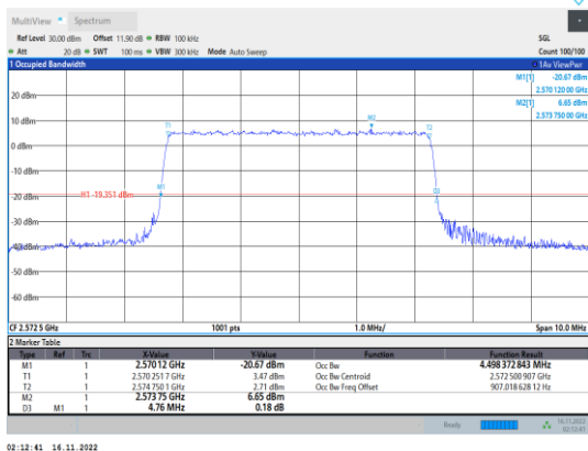
Band38-5MHz-64QAM-37775-25RB#0
