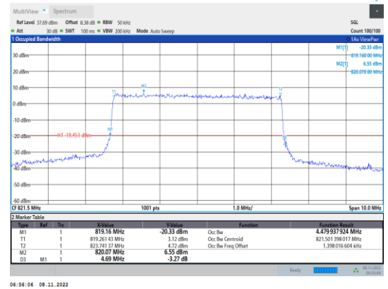
Band26-5MHz-16QAM-26765-25RB#0
