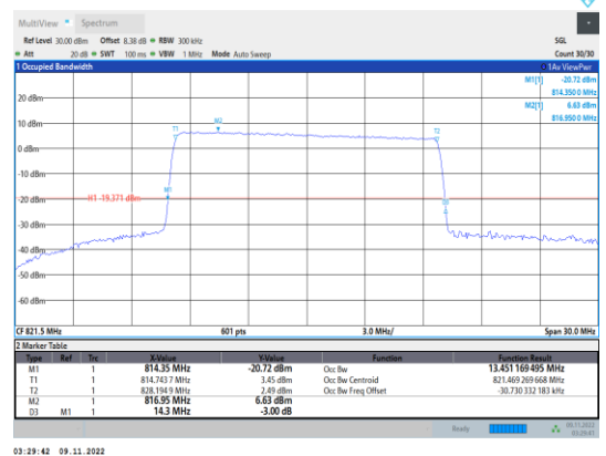
Band26-15MHz-16QAM-26765-75RB#0
