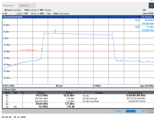
Band26-15MHz-QPSK-26765-75RB#0
