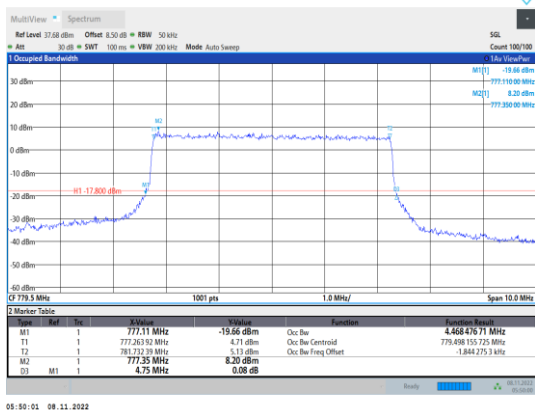
Band13-5MHz-QPSK-23205-25RB#0
