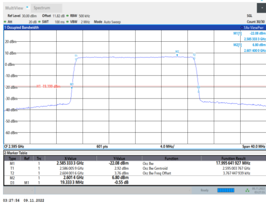
Band38-20MHz-16QAM-38000-100RB#0
