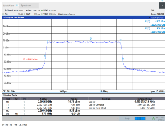
Band38-5MHz-QPSK-38000-25RB#0
