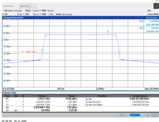
Band38-10MHz-16QAM-38200-50RB#0
