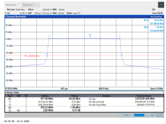
Band26-3MHz-64QAM-26740-15RB#0
