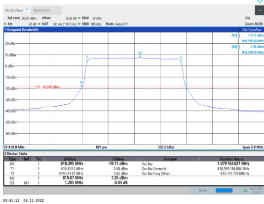
Band26-1.4MHz-QPSK-26740-6RB#0
