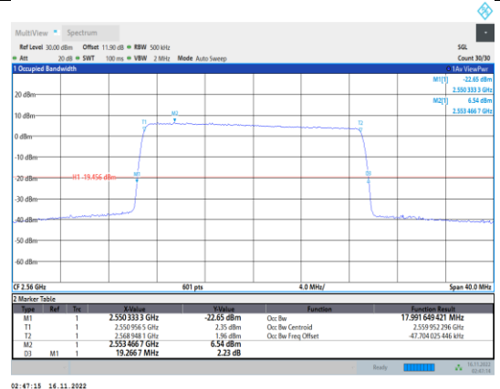
Band7-20MHz-64QAM-21350-100RB#0
