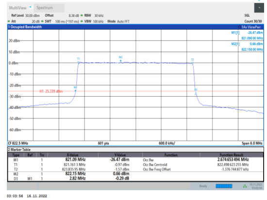
Band26-3MHz-64QAM-26775-15RB#0
