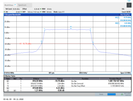
Band26-1.4MHz-16QAM-26740-6RB#0
