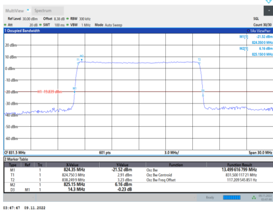
Band26-15MHz-QPSK-26865-75RB#0
