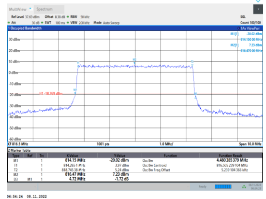
Band26-5MHz-16QAM-26715-25RB#0
