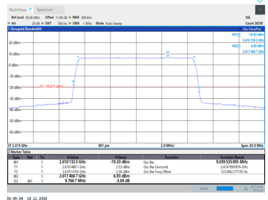
Band38-10MHz-64QAM-38200-50RB#0
