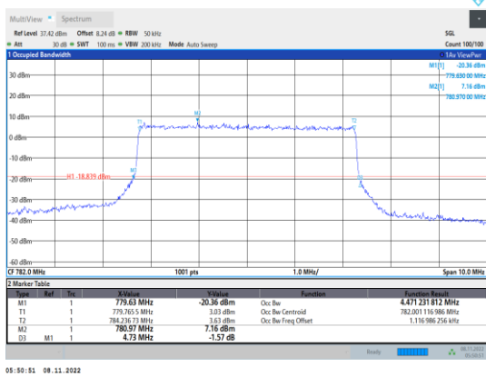
Band13-5MHz-QPSK-23230-25RB#0
