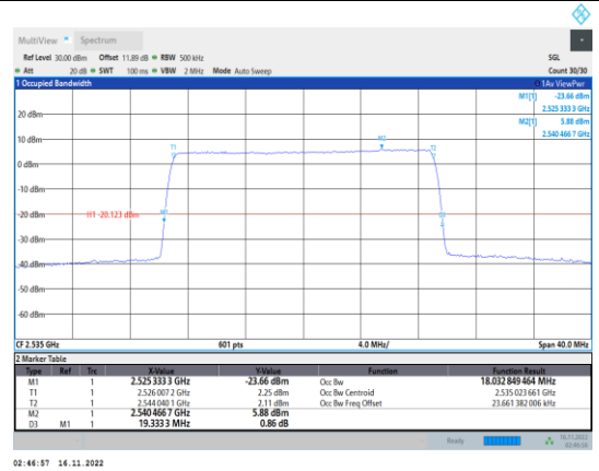
Band7-20MHz-64QAM-21100-100RB#0
