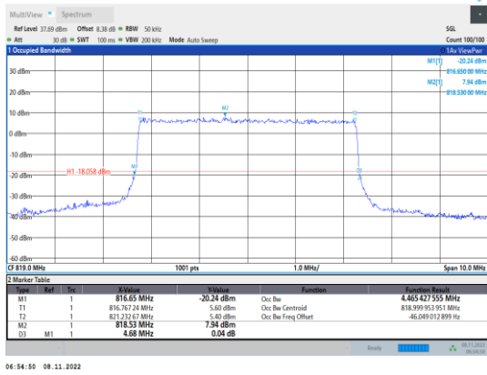
Band26-5MHz-QPSK-26740-25RB#0
