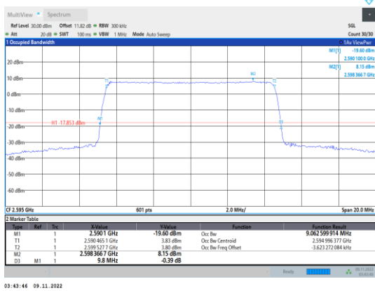
Band38-10MHz-16QAM-38000-50RB#0
