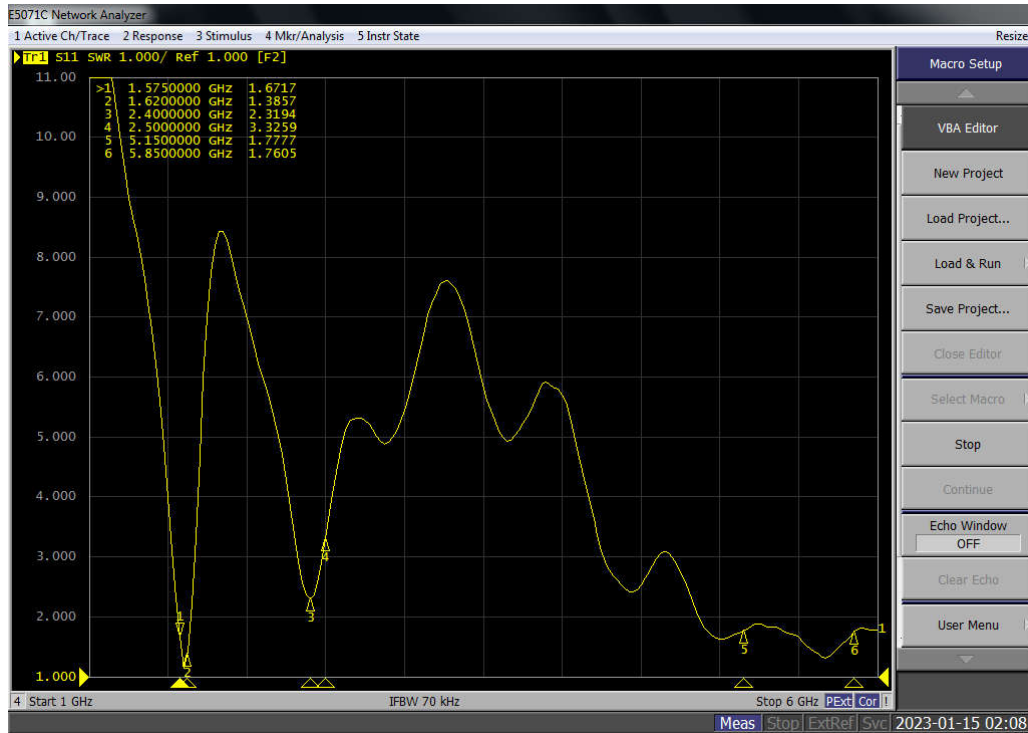
Picture one: VSWR
