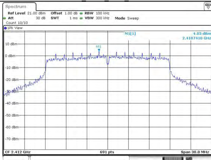
11n20SISO_Ant22_2412_0~Reference
