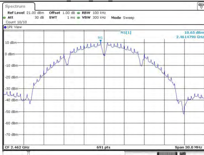
11b_Ant22_2462_0~Reference
