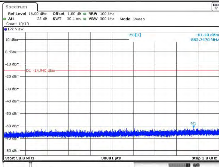
11n20SISO_Ant22_2462_30~1000
