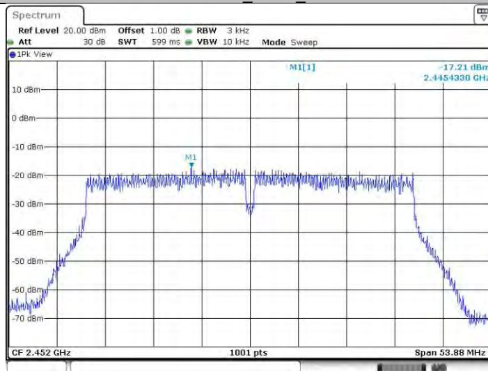
11n40SISO_Ant22_2452
