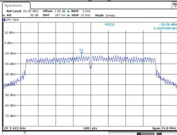
11n20SISO_Ant22_2412
