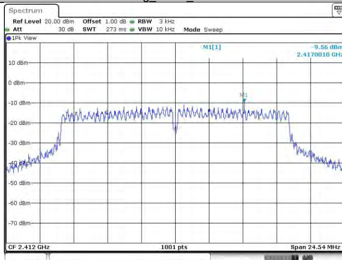
11g_Ant22_2412
