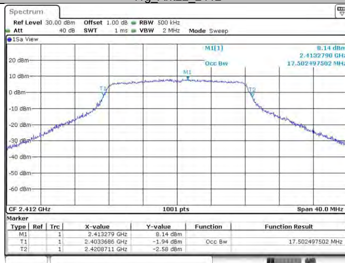
11g_Ant22_2412
