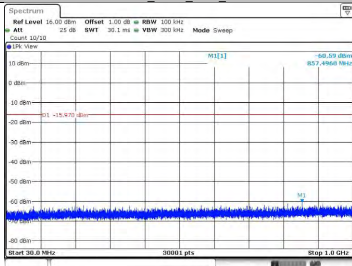
11n20SISO_Ant22_2412_30~1000
