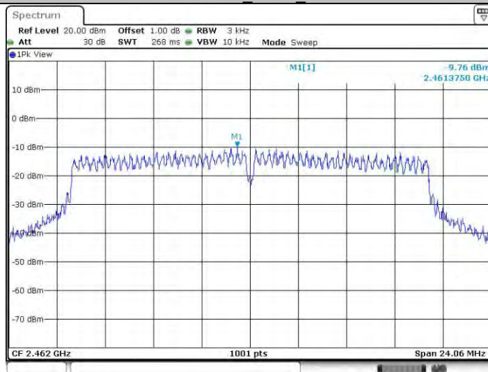
11n20SISO_Ant22_2462
