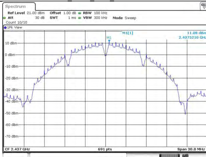
11b_Ant22_2437_0~Reference
