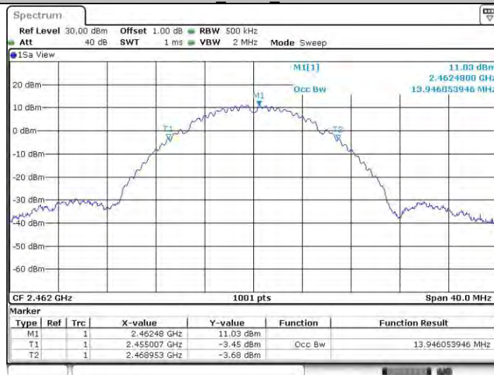
11b_Ant22_2462
