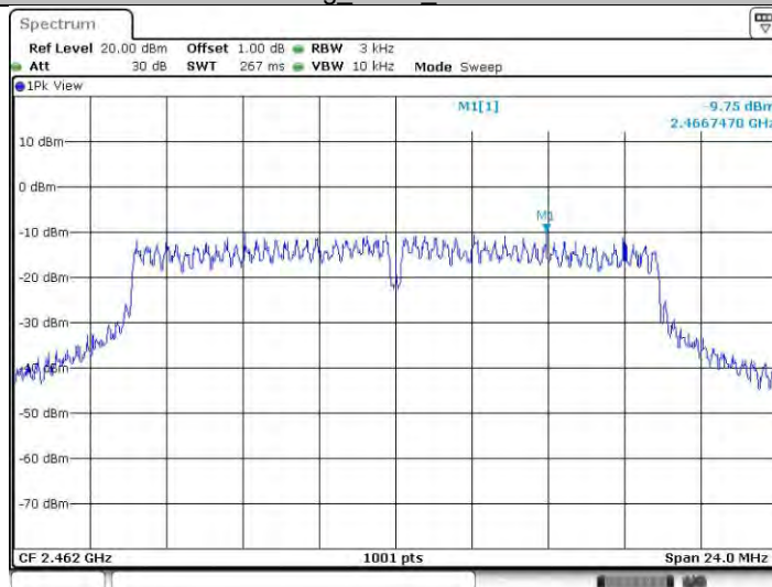
11g_Ant22_2462
