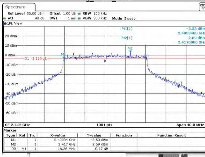
11g_Ant22_2412
