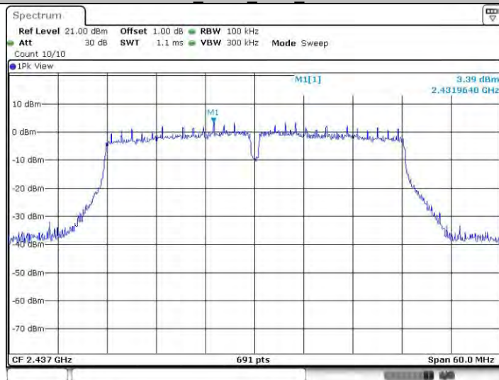
11n40SISO_Ant22_2437_0~Reference
