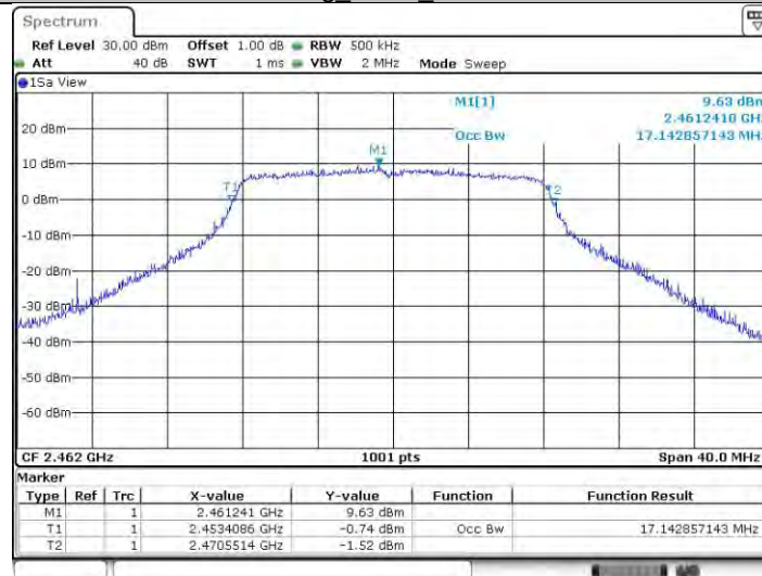
11g_Ant22_2462
