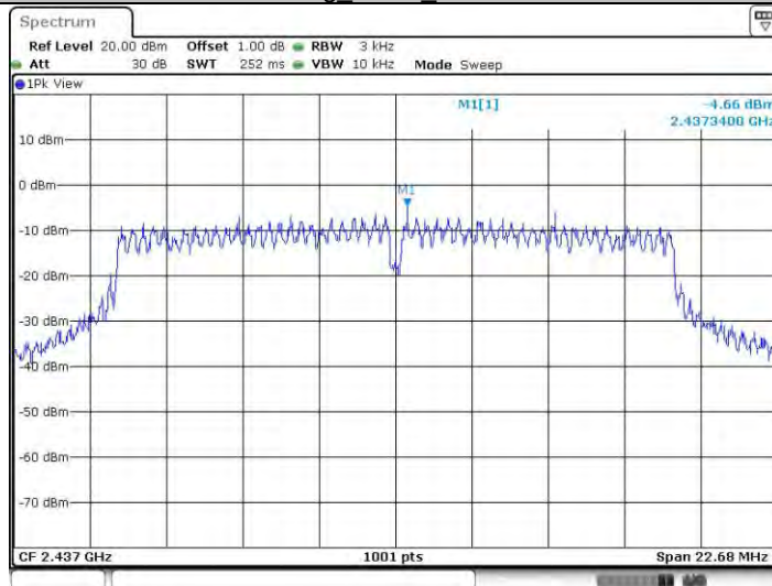
11g_Ant22_2437
