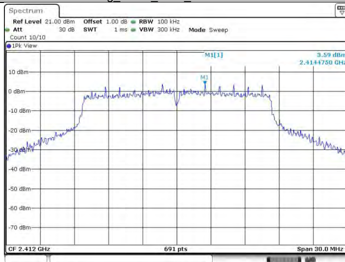
11g_Ant22_2412_0~Reference
