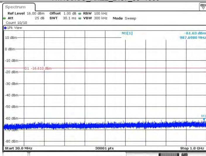
11n40SISO_Ant22_2437_30~1000
