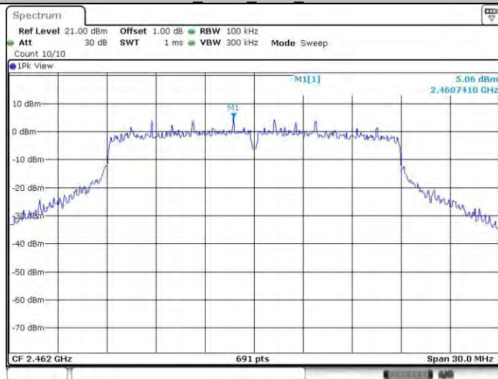
11n20SISO_Ant22_2462_0~Reference
