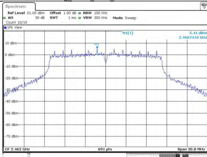
11g_Ant22_2462_0~Reference
