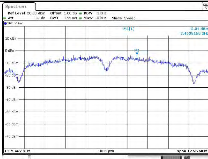
11b_Ant22_2462
