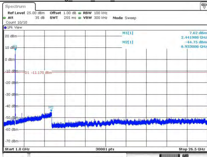
11g_Ant22_2437_1000~26500
