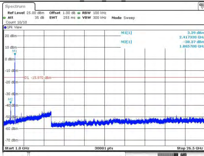
11n20SISO_Ant22_2412_1000~26500
