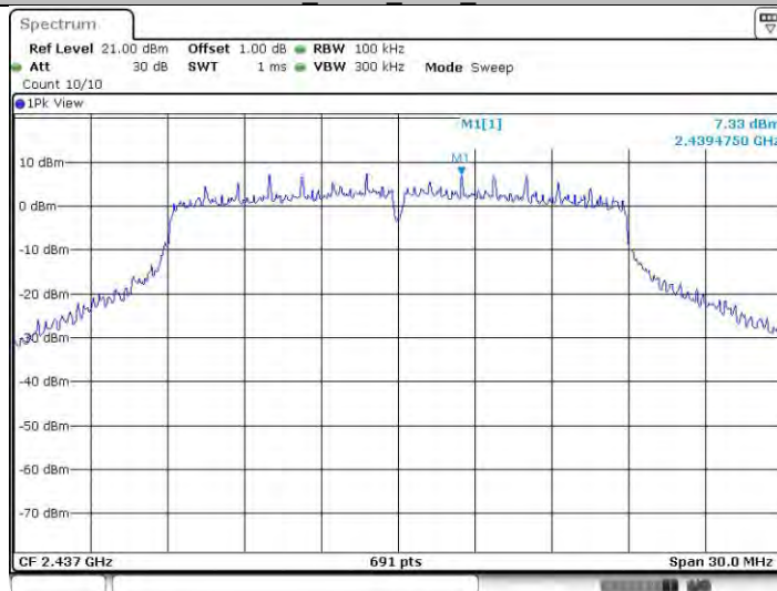
11n20SISO_Ant22_2437_0~Reference
