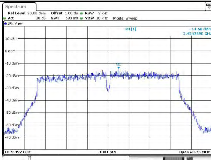
11n40SISO_Ant22_2422
