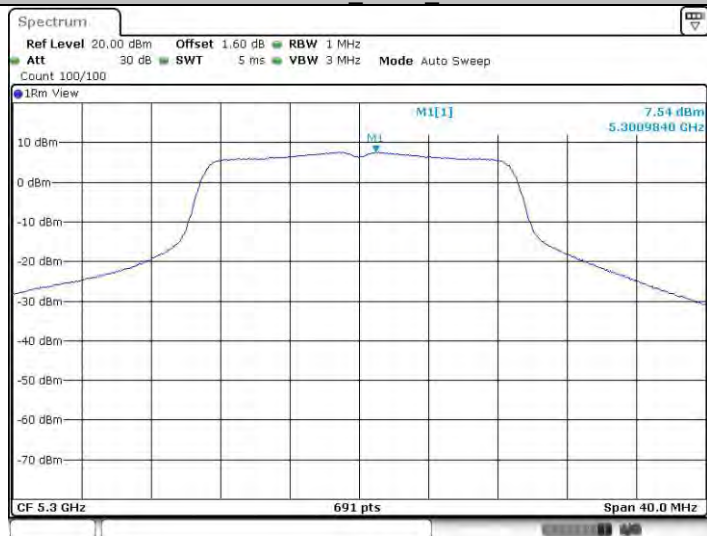
11n20SISO_Ant22_5300
