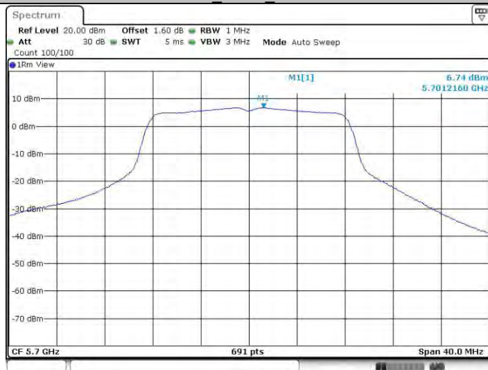
11a_Ant22_5700
