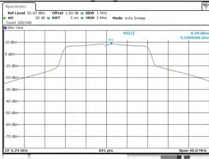
11a_Ant22_5240
