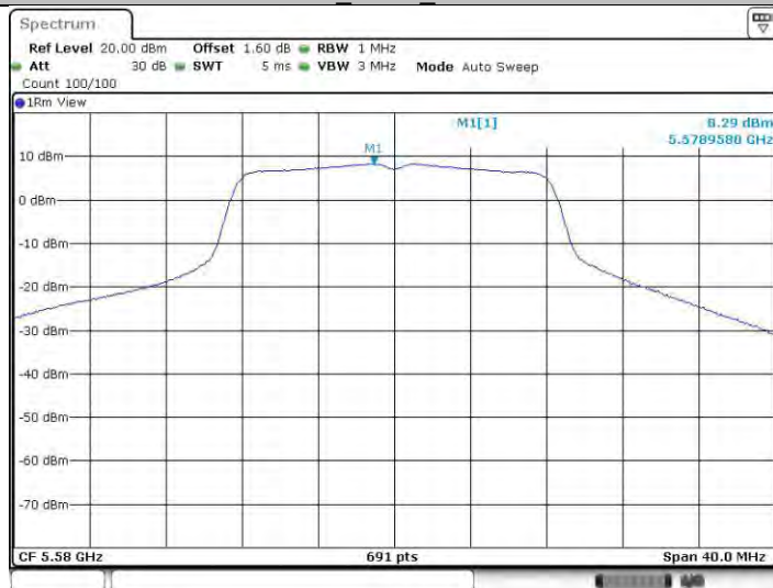
11a_Ant22_5580
