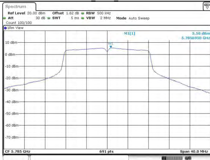
11a_Ant22_5785
