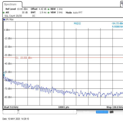
GSM850-190-5-0.009~0.15MHz-0.01
