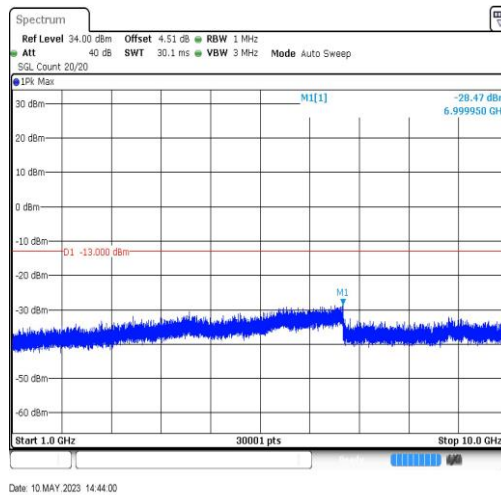
EGPRS850-128-8-1000~10000MHz-6999.95
