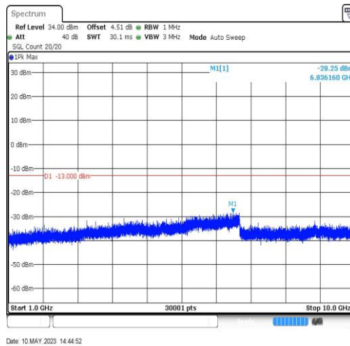
EGPRS850-251-8-1000~10000MHz-6836.16
