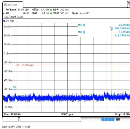
EGPRS850-128-8-30~1000MHz-118.27
