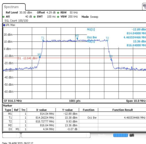
Band26-5MHz-16QAM-26715-25RB#0-4.466
