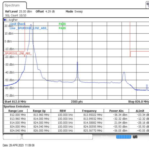
Band26-10MHz-QPSK-26740-1RB#0
