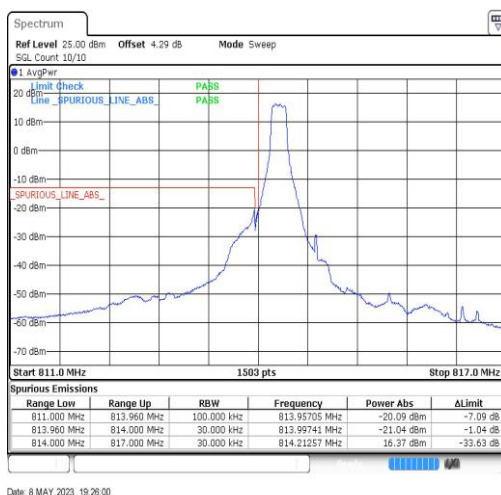
Band26-1.4MHz-QPSK-26697-1RB#0
