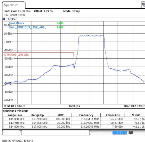
Band26-1.4MHz-QPSK-26697-6RB#0
