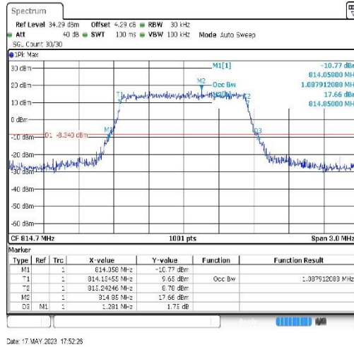
Band26-1.4MHz-QPSK-26697-6RB#0-2.97
