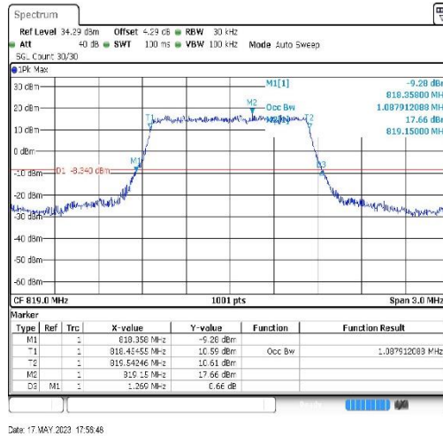
Band26-1.4MHz-QPSK-26740-6RB#0-2.973
