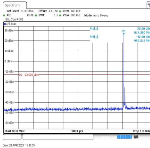
Band26-10MHz-QPSK-26740-1RB#0-Range3:30~1000MHz
