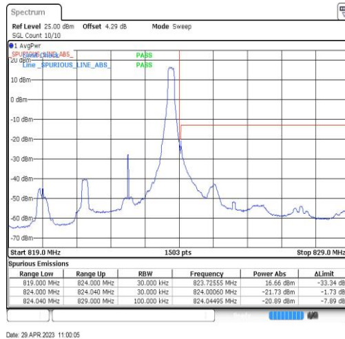
Band26-3MHz-QPSK-26775-1RB#14
