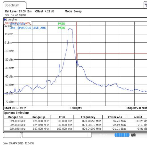
Band26-1.4MHz-QPSK-26783-1RB#5
