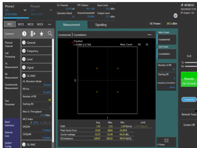
Band26-10MHz-QPSK-26740-50RB#0
