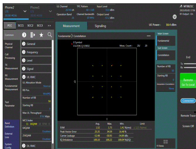
Band26-10MHz-16QAM-26740-50RB#0
