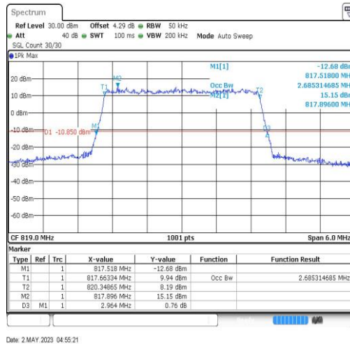
Band26-3MHz-64QAM-26740-15RB#0-2.685
