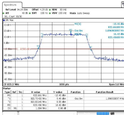
Band26-1.4MHz-16QAM-26740-6RB#0-2.97
