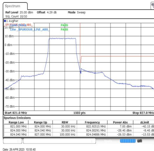
Band26-1.4MHz-QPSK-26783-6RB#0
