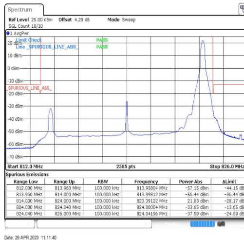
Band26-10MHz-QPSK-26740-1RB#49
