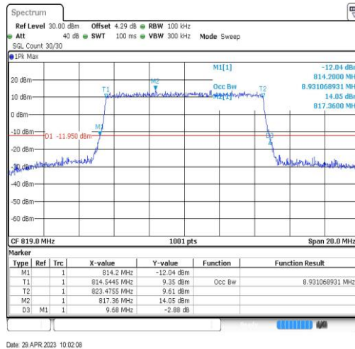
Band26-10MHz-16QAM-26740-50RB#0-8.931
