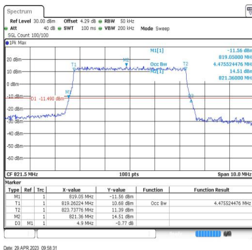
Band26-5MHz-QPSK-26765-25RB#0-4.476
