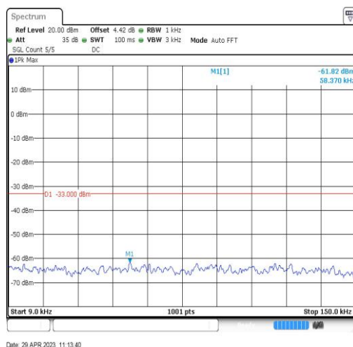
Band26-10MHz-QPSK-26740-1RB#0-Range1:0.009~0.15MHz
