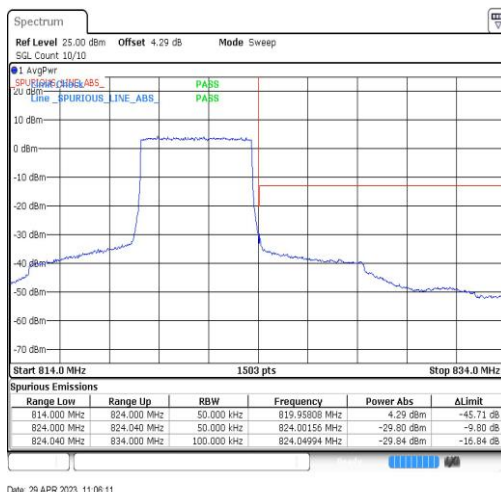
Band26-5MHz-QPSK-26765-25RB#0
