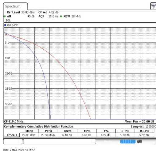
Band26-10MHz-QPSK-26740-50RB#0
