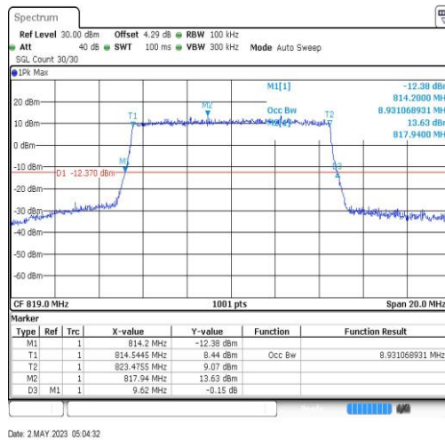
Band26-10MHz-64QAM-26740-50RB#0-8.931
