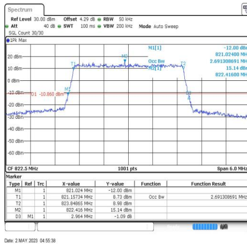
Band26-3MHz-64QAM-26775-15RB#0-2.691
