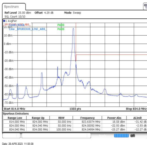
Band26-5MHz-QPSK-26765-1RB#24
