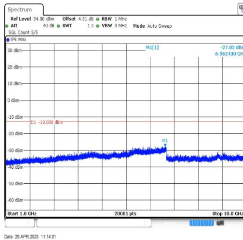
Band26-10MHz-QPSK-26740-1RB#0-Range4:1000~10000MHz
