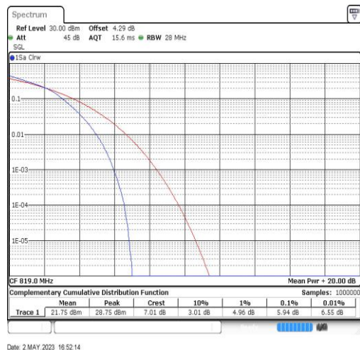
Band26-10MHz-16QAM-26740-50RB#0
