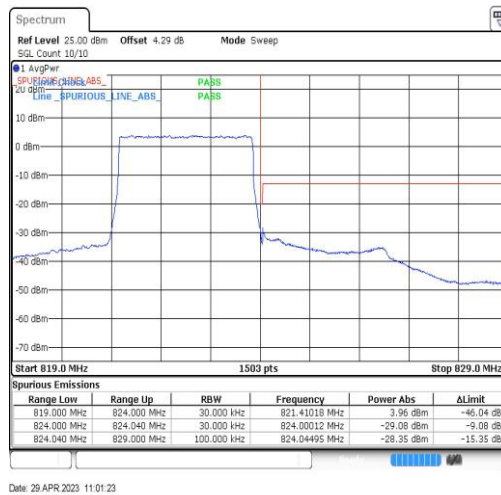
Band26-3MHz-QPSK-26775-15RB#0
