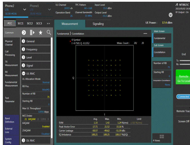
Band26-15MHz-64QAM-26915-75RB#0
