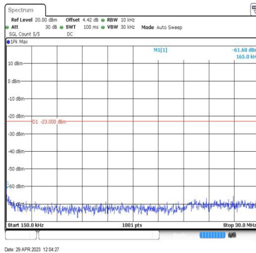
Band26-15MHz-QPSK-26965-1RB#0-Range2:0.15~30MHz
