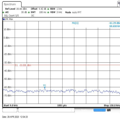
Band26-15MHz-QPSK-26965-1RB#0-Range1:0.009~0.15MHz
