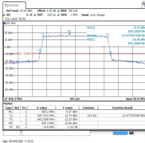
Band26-15MHz-16QAM-26915-75RB#0-13.478
