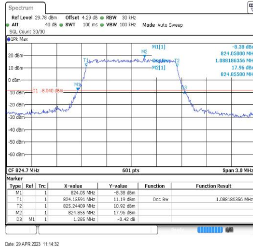
Band26-1.4MHz-QPSK-26797-6RB#0-1.088
