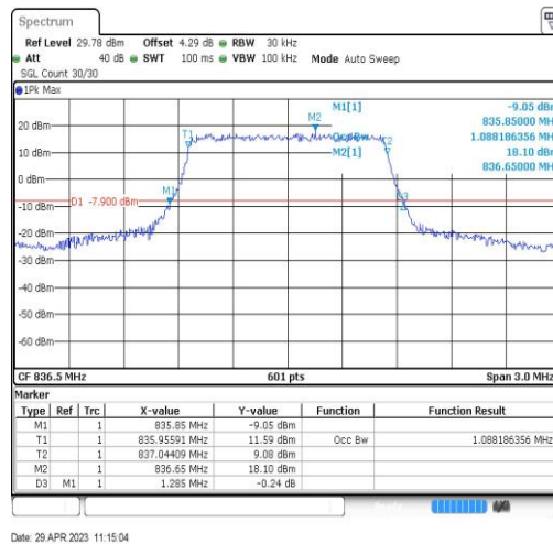
Band26-1.4MHz-QPSK-26915-6RB#0-1.088
