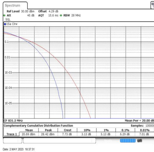
Band26-15MHz-64QAM-26865-75RB#0
