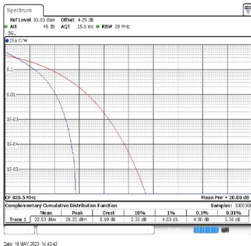
Band26-15MHz-QPSK-26915-75RB#0
