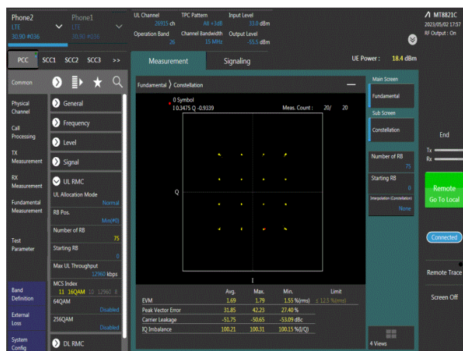
Band26-15MHz-16QAM-26915-75RB#0
