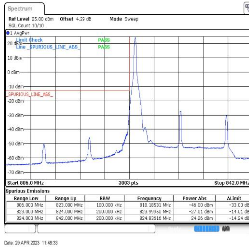
Band26-15MHz-QPSK-26865-1RB#0
