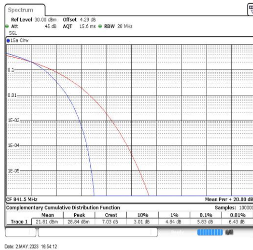
Band26-15MHz-16QAM-26965-75RB#0
