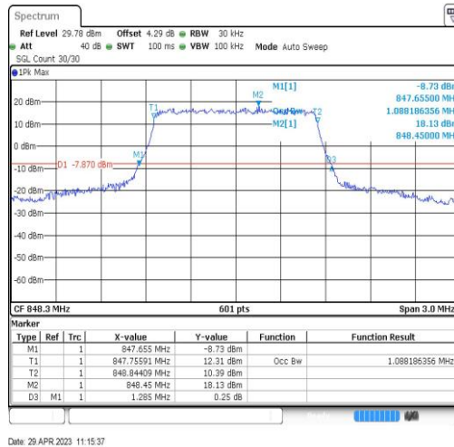
Band26-1.4MHz-QPSK-27033-6RB#0-1.088
