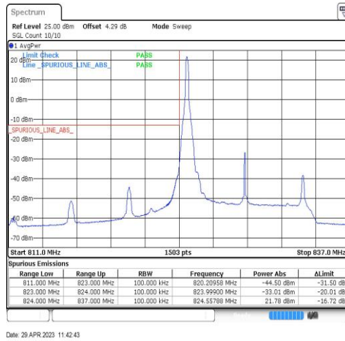
Band26-10MHz-QPSK-26840-1RB#0
