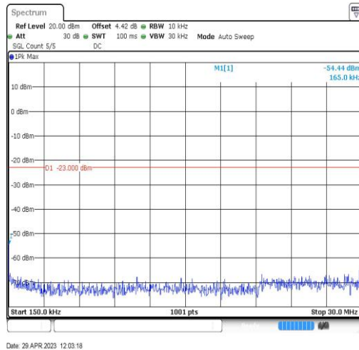
Band26-15MHz-QPSK-26865-1RB#0-Range2:0.15~30MHz
