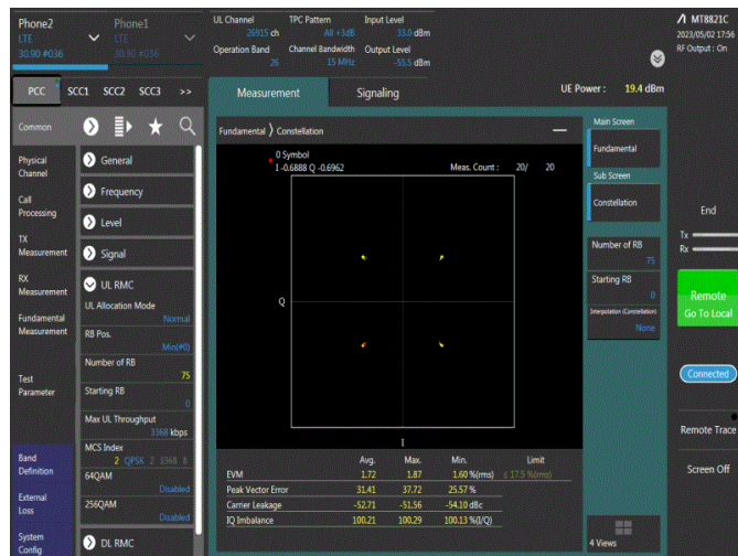
Band26-15MHz-QPSK-26915-75RB#0
