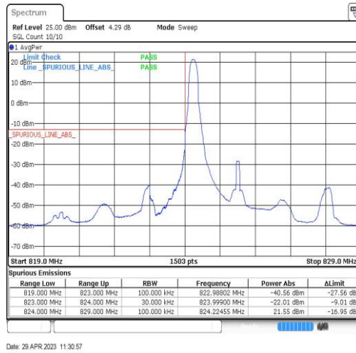
Band26-3MHz-QPSK-26805-1RB#0
