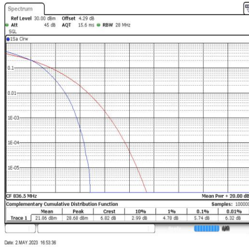
Band26-15MHz-16QAM-26915-75RB#0
