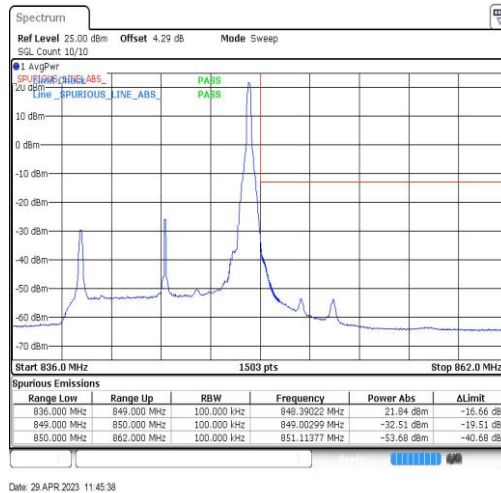
Band26-10MHz-QPSK-26990-1RB#49
