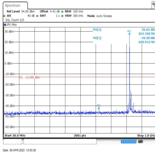
Band26-15MHz-QPSK-26865-1RB#0-Range3:30~1000MHz
