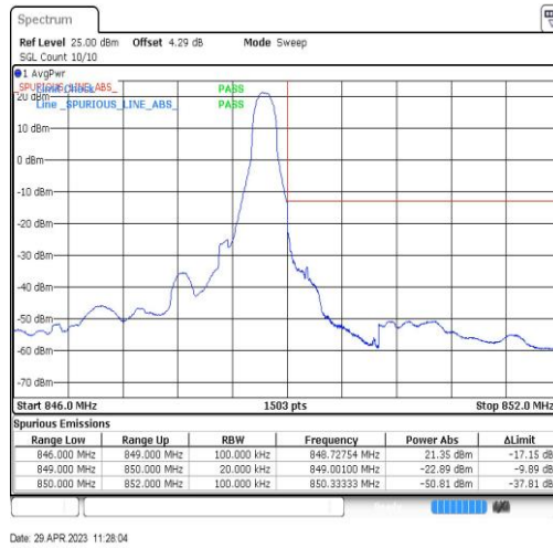
Band26-1.4MHz-QPSK-27033-1RB#5
