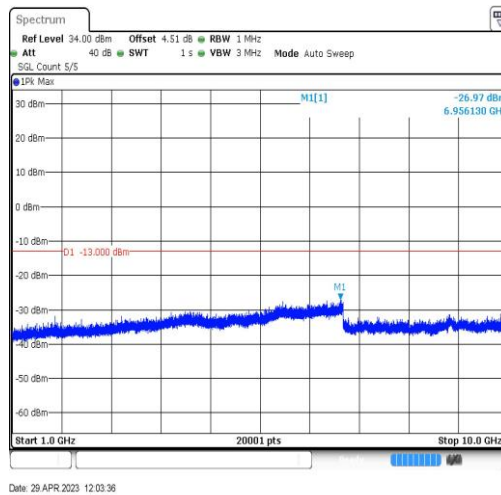
Band26-15MHz-QPSK-26865-1RB#0-Range4:1000~10000MHz
