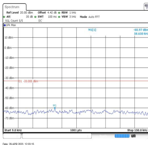
Band26-15MHz-QPSK-26865-1RB#0-Range1:0.009~0.15MHz
