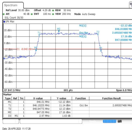
Band26-3MHz-QPSK-27025-15RB#0-2.696
