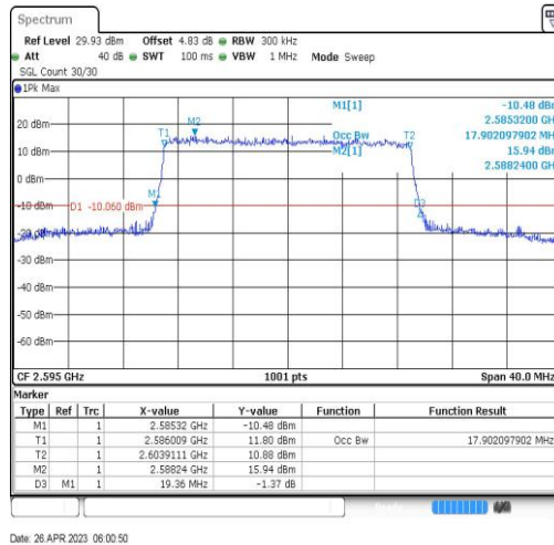
Band38-20MHz-QPSK-38000-100RB#0-17.902
