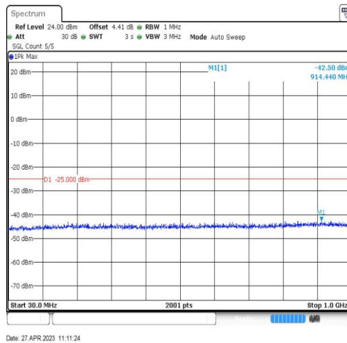
Band38-20MHz-QPSK-38000-1RB#0-Range3:30~1000MHz
