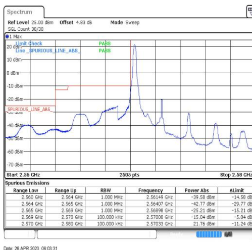
Band38-5MHz-QPSK-37775-1RB#0
