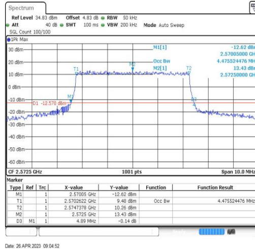
Band38-5MHz-QPSK-37775-25RB#0-4.476
