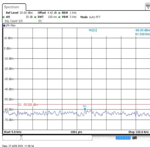
Band38-20MHz-QPSK-37850-1RB#0-Range1:0.009~0.15MHz
