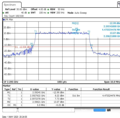
Band38-5MHz-64QAM-38000-25RB#0-4.476
