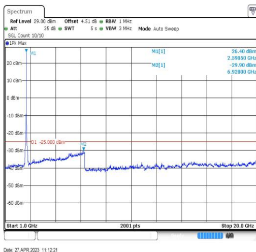
Band38-20MHz-QPSK-38000-1RB#0-Range4:1000~20000MHz
