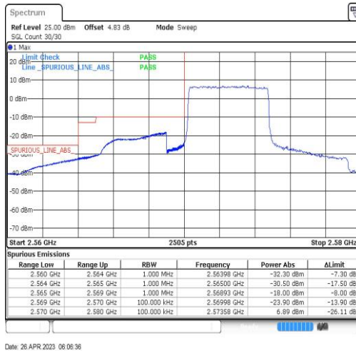
Band38-5MHz-QPSK-37775-25RB#0
