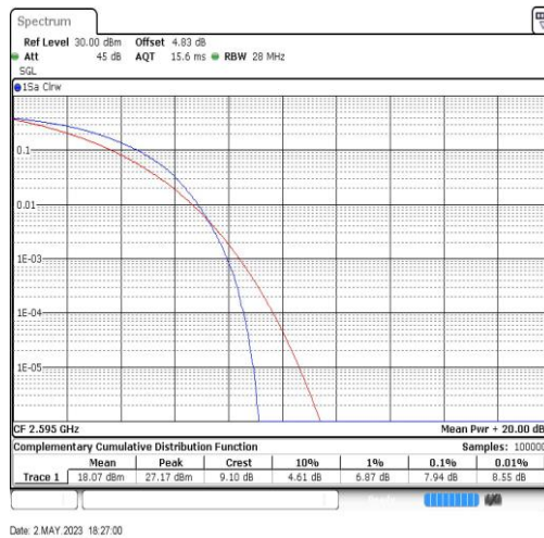
Band38-20MHz-64QAM-38000-100RB#0
