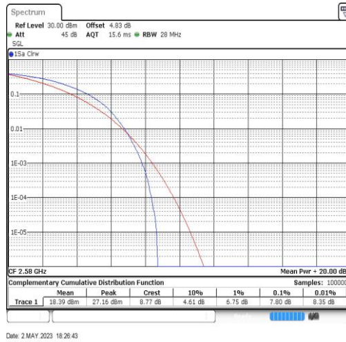
Band38-20MHz-64QAM-37850-100RB#0
