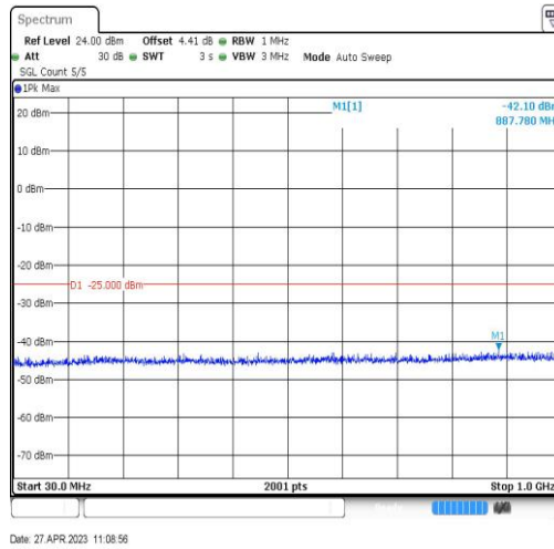
Band38-20MHz-QPSK-37850-1RB#0-Range3:30~1000MHz
