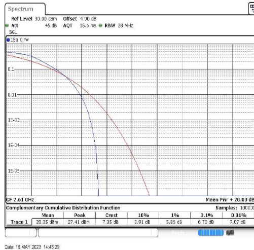
Band38-20MHz-QPSK-38150-100RB#0
