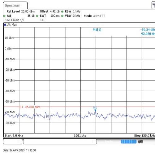
Band38-20MHz-QPSK-38150-1RB#0-Range1:0.009~0.15MHz
