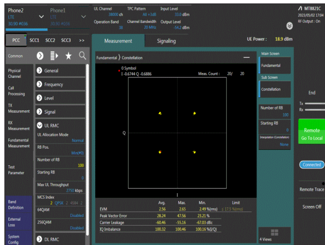
Band38-20MHz-QPSK-38000-100RB#0
