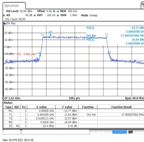
Band38-20MHz-QPSK-38150-100RB#0-17.902
