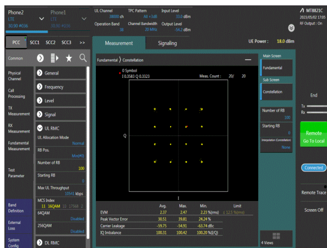
Band38-20MHz-16QAM-38000-100RB#0
