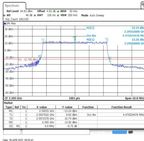
Band38-5MHz-QPSK-38000-25RB#0-4.476
