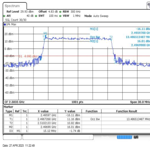
Band41-15MHz-16QAM-39725-75RB#0-13.487
