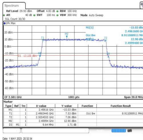
Band41-10MHz-64QAM-39700-50RB#0-8.911
