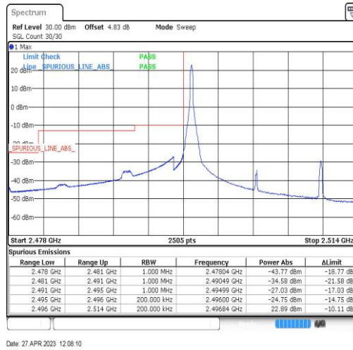
Band41-15MHz-QPSK-39725-1RB#0
