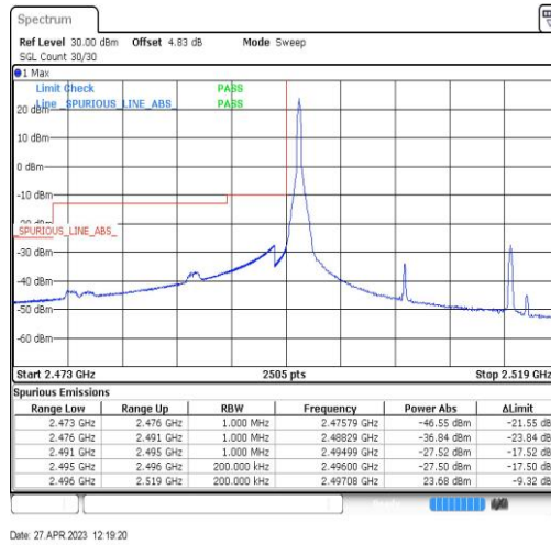
Band41-20MHz-QPSK-39750-1RB#0
