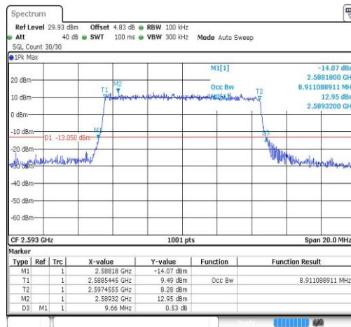
Band41-10MHz-16QAM-39700-50RB#0-8.911
