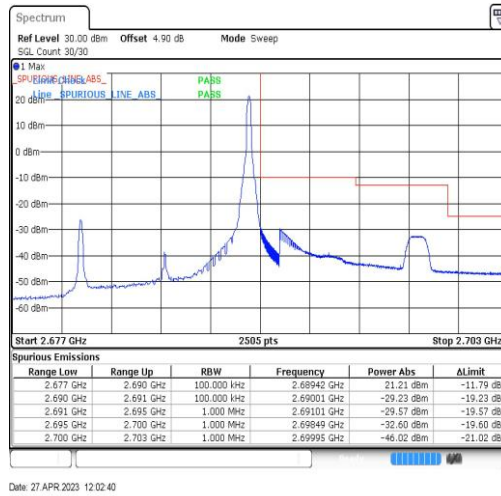
Band41-10MHz-QPSK-41540-1RB#49
