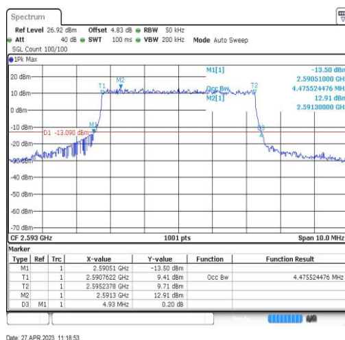
Band41-5MHz-QPSK-40620-25RB#0-4.476
