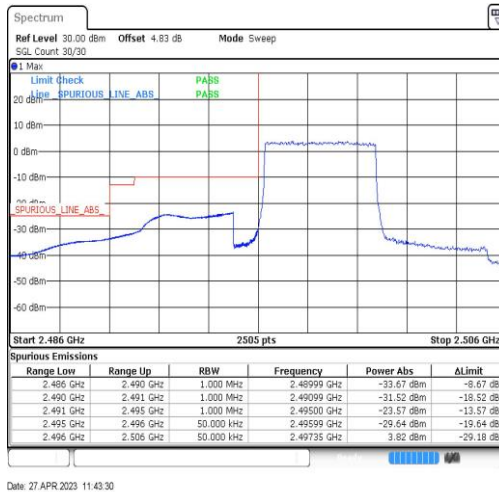
Band41-5MHz-QPSK-39675-25RB#0
