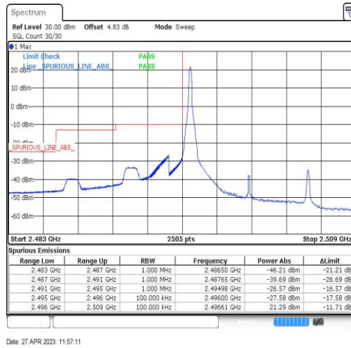
Band41-10MHz-QPSK-39700-1RB#0
