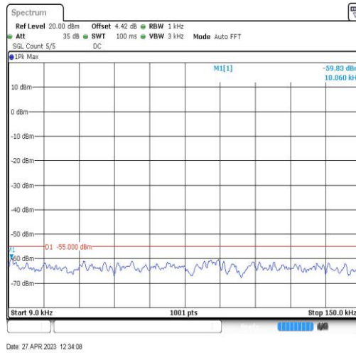
Band41-20MHz-QPSK-41490-1RB#0-Range1:0.009~0.15MHz
