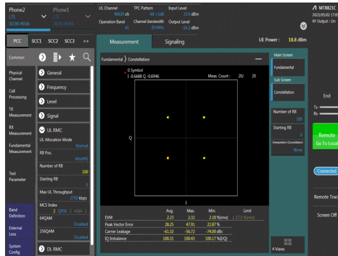
Band41-20MHz-QPSK-40620-100RB#0
