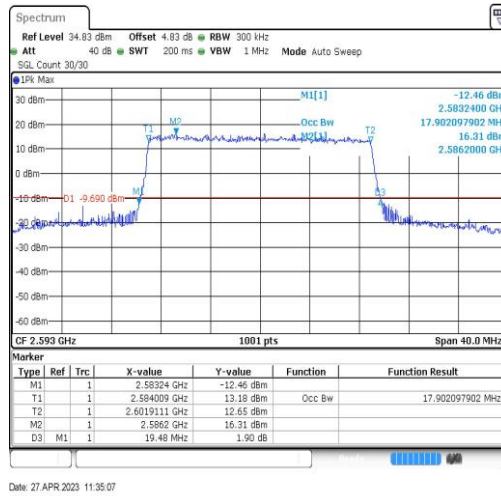
Band41-20MHz-QPSK-40620-100RB#0-17.902
