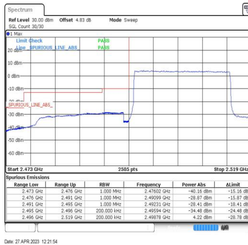
Band41-20MHz-QPSK-39750-100RB#0
