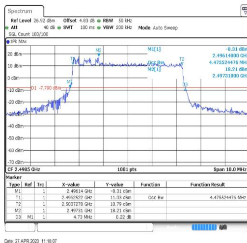
Band41-5MHz-QPSK-39675-25RB#0-4.476
