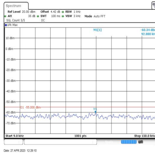
Band41-20MHz-QPSK-39750-1RB#0-Range1:0.009~0.15MHz
