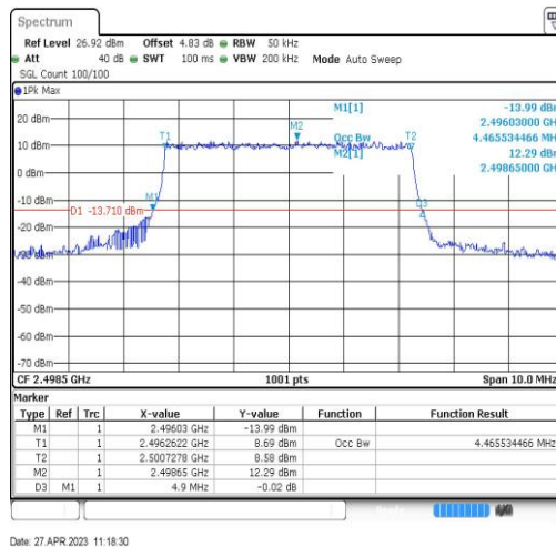
Band41-5MHz-16QAM-39675-25RB#0-4.466
