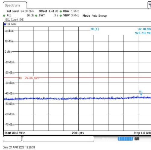
Band41-20MHz-QPSK-39750-1RB#0-Range3:30~1000MHz
