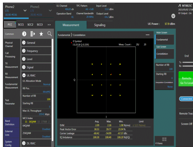
Band41-20MHz-16QAM-40620-100RB#0
