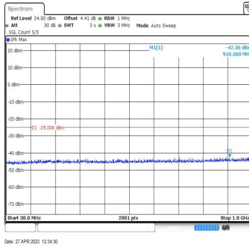
Band41-20MHz-QPSK-41490-1RB#0-Range3:30~1000MHz
