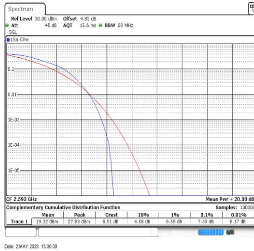
Band41-20MHz-16QAM-40620-100RB#0
