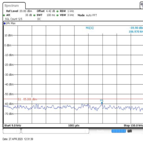
Band41-20MHz-QPSK-40620-1RB#0-Range1:0.009~0.15MHz
