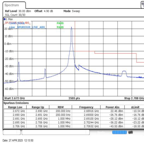
Band41-15MHz-QPSK-41515-1RB#74
