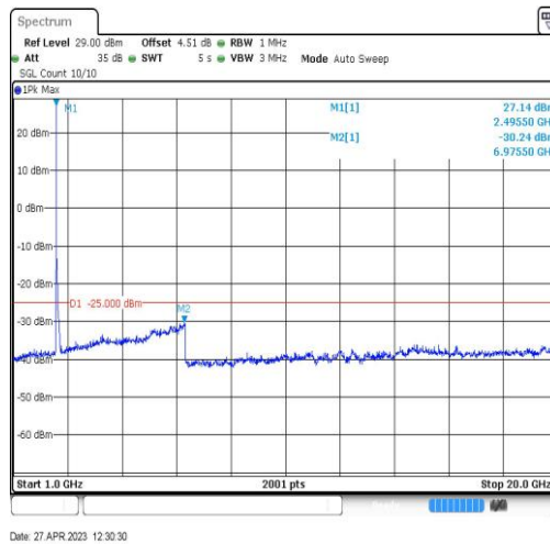
Band41-20MHz-QPSK-39750-1RB#0-Range4:1000~20000MHz
