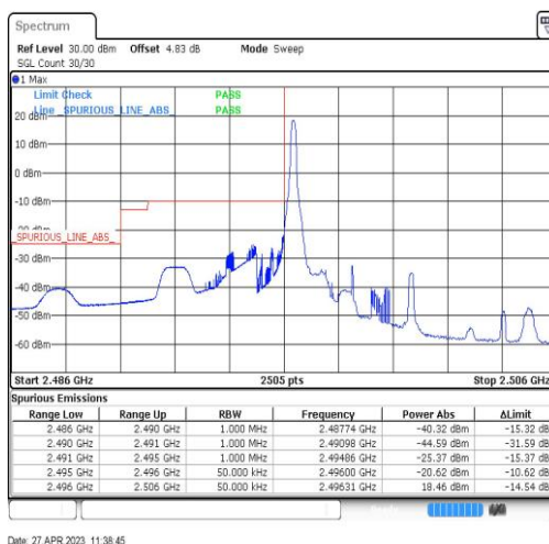
Band41-5MHz-QPSK-39675-1RB#0
