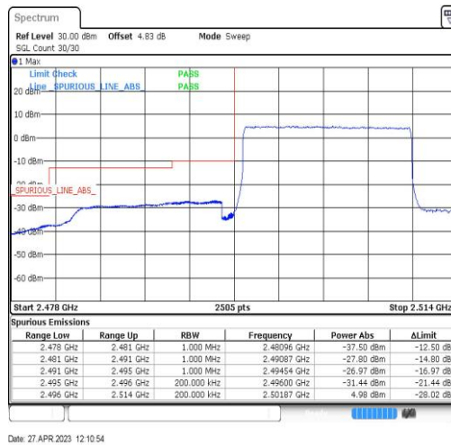
Band41-15MHz-QPSK-39725-75RB#0
