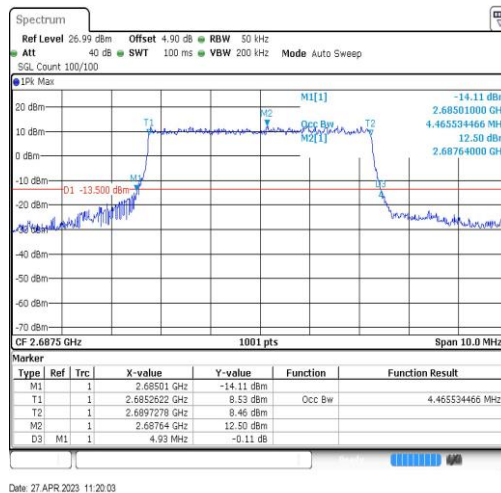
Band41-5MHz-16QAM-41565-25RB#0-4.466
