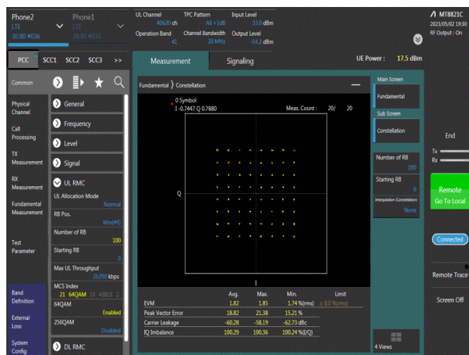
Band41-20MHz-64QAM-40620-100RB#0
