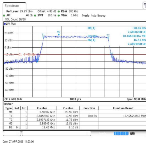
Band41-15MHz-QPSK-40620-75RB#0-13.457
