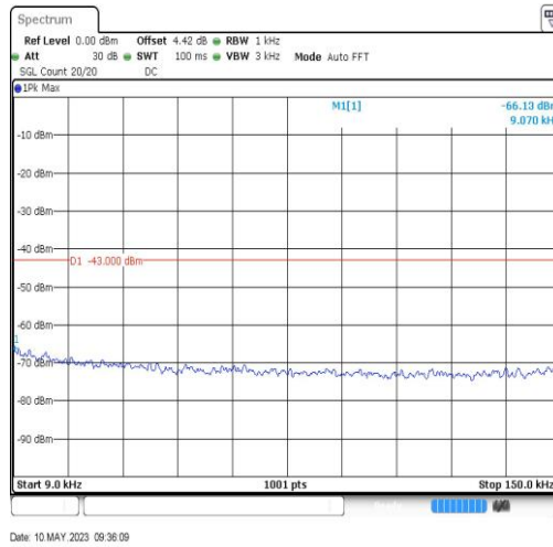
Band IV-1312-0.009~0.15MHz-0.01
