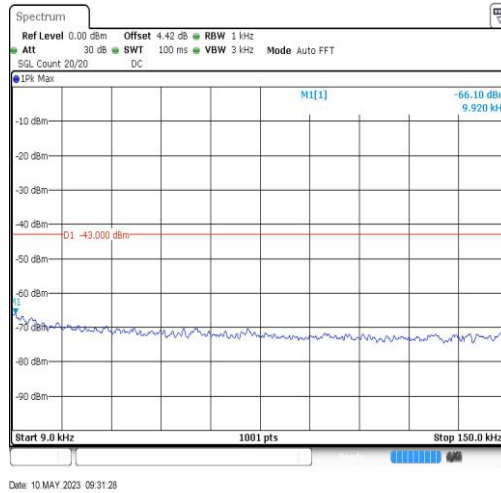
BandII-9262-0.009~0.15MHz-0.01
