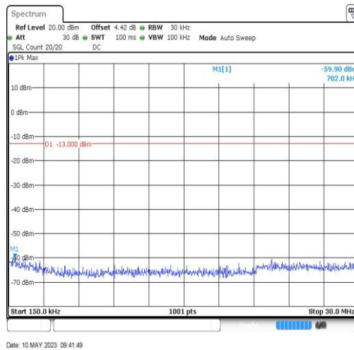
BandV-4182-0.15~30MHz-0.7
