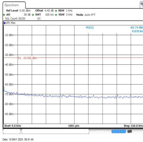
BandV-4182-0.009~0.15MHz-0.01
