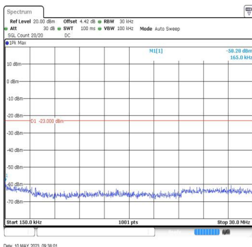
BandIV-1513-0.15~30MHz-0.17
