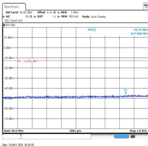
BandIV-1513-30~1000MHz-847.06
