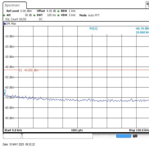
BandII-9400-0.009~0.15MHz-0.01
