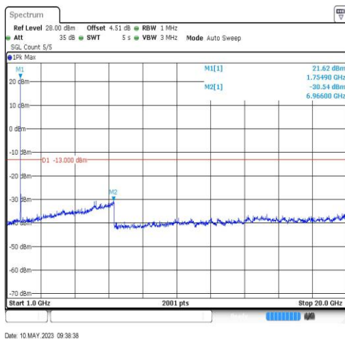
BandIV-1513-1000~20000MHz-6966
