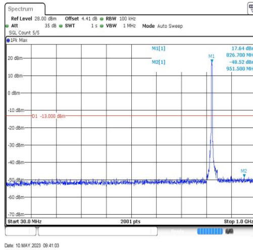
BandV-4132-30~1000MHz-951.5
