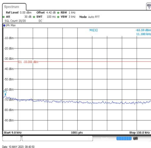
BandV-4132-0.009~0.15MHz-0.01
