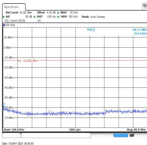
BandV-4132-0.15~30MHz-0.31
