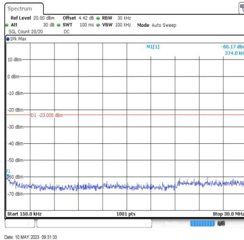
BandII-9262-0.15~30MHz-0.37
