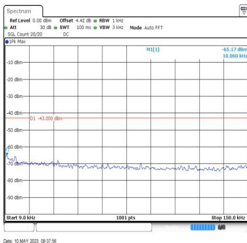
BandIV-1513-0.009~0.15MHz-0.01
