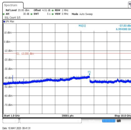
BandV-4132-1000~10000MHz-6994.38
