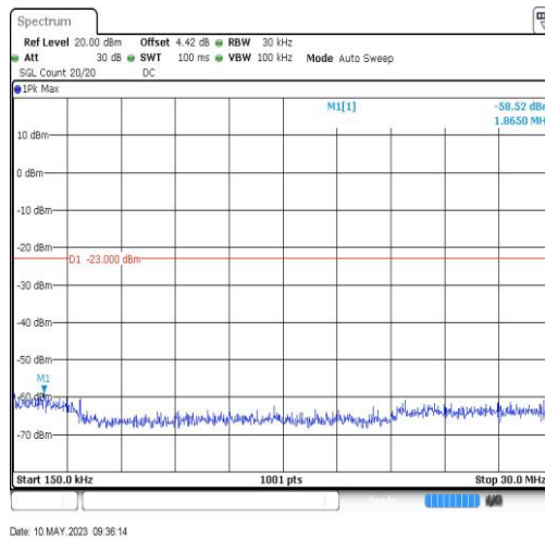
Band IV-1312-0.15~30MHz-1.87
