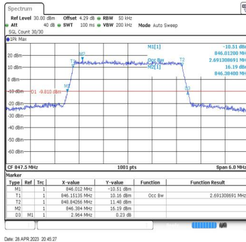
Band5-3MHz-16QAM-20635-15RB#0-2.691
