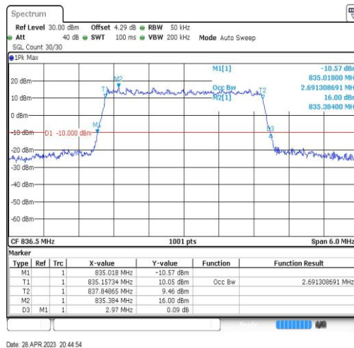
Band5-3MHz-16QAM-20525-15RB#0-2.691
