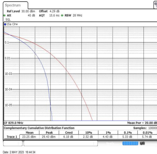
Band5-10MHz-QPSK-20450-50RB#0
