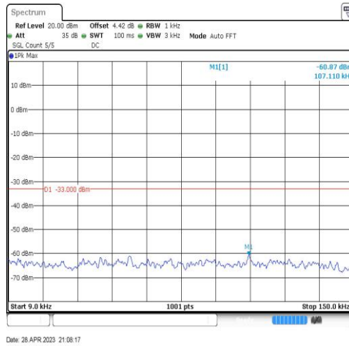
Band5-10MHz-QPSK-20600-1RB#0-Range1:0.009~0.15MHz
