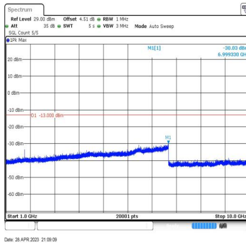
Band5-10MHz-QPSK-20600-1RB#0-Range4:1000~10000MHz
