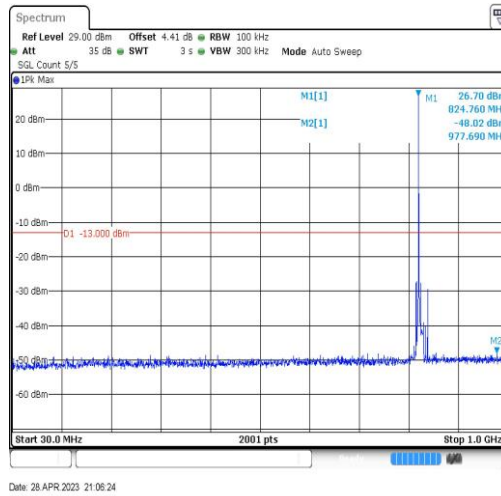
Band5-10MHz-QPSK-20450-1RB#0-Range3:30~1000MHz
