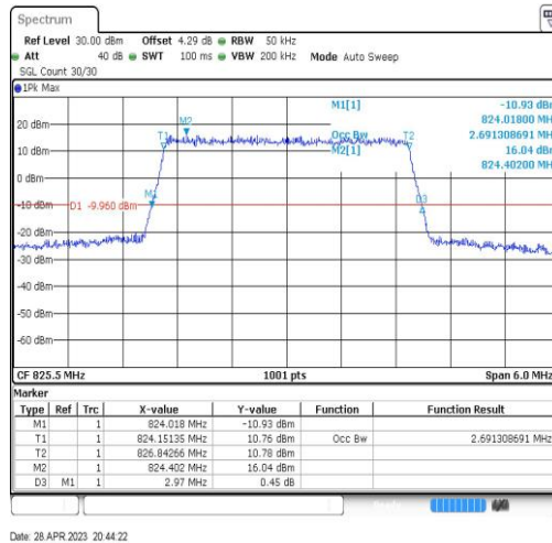
Band5-3MHz-16QAM-20415-15RB#0-2.691
