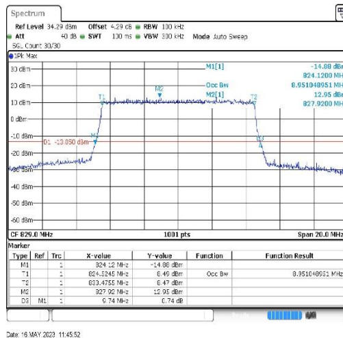
Band5-10MHz-64QAM-20450-50RB#0-8.951
