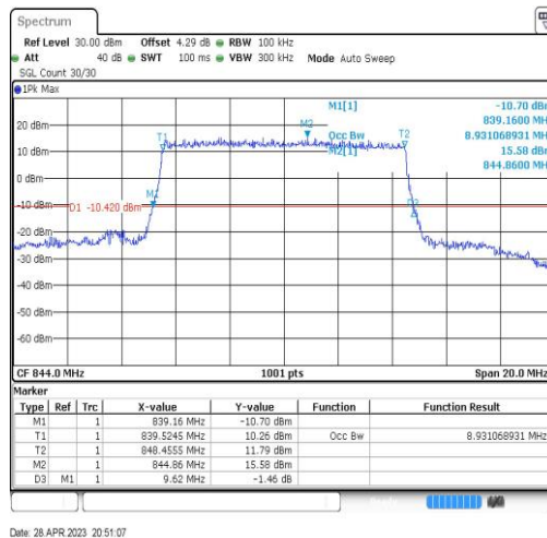
Band5-10MHz-QPSK-20600-50RB#0-8.931
