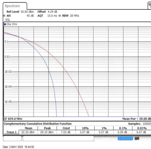
Band5-10MHz-16QAM-20450-50RB#0
