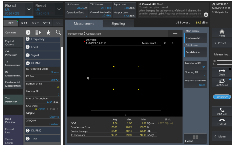
Band5-10MHz-QPSK-20525-50RB#0
