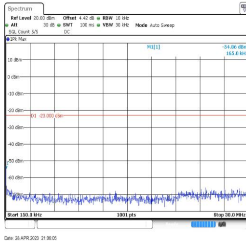
Band5-10MHz-QPSK-20450-1RB#0-Range2:0.15~30MHz
