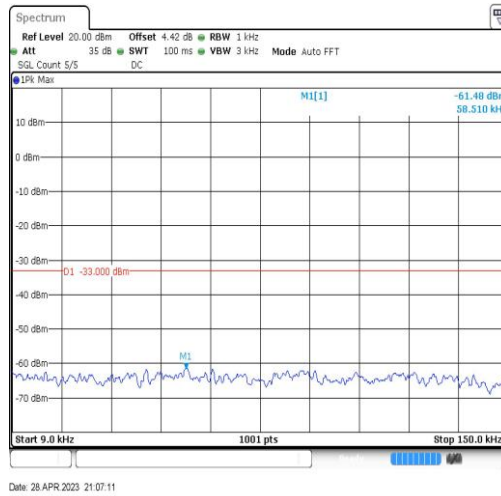
Band5-10MHz-QPSK-20525-1RB#0-Range1:0.009~0.15MHz
