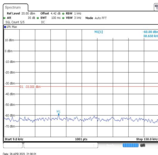
Band5-10MHz-QPSK-20450-1RB#0-Range1:0.009~0.15MHz
