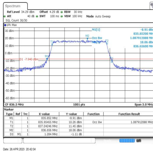
Band5-1.4MHz-QPSK-20525-6RB#0-1.088
