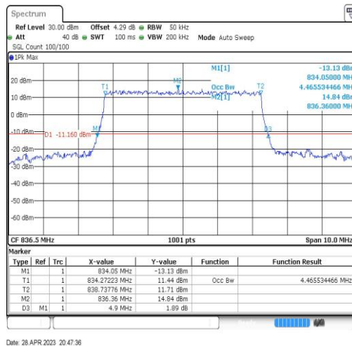
Band5-5MHz-QPSK-20525-25RB#0-4.466
