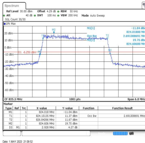
Band5-3MHz-64QAM-20415-15RB#0-2.691
