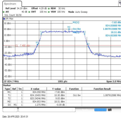
Band5-1.4MHz-QPSK-20407-6RB#0-1.088
