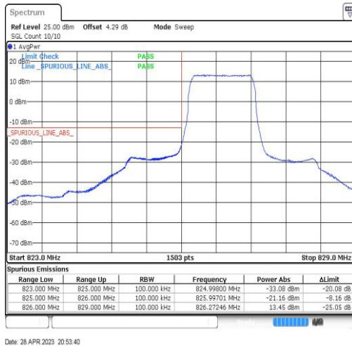
Band5-1.4MHz-QPSK-20427-6RB#0
