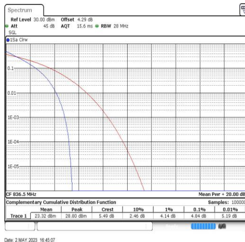
Band5-10MHz-QPSK-20525-50RB#0
