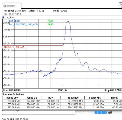
Band5-1.4MHz-QPSK-20427-1RB#0
