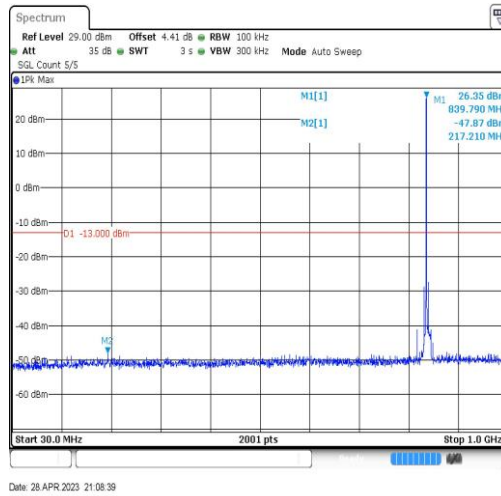
Band5-10MHz-QPSK-20600-1RB#0-Range3:30~1000MHz
