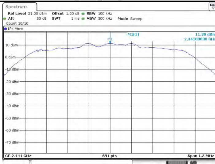
2DH5_Ant22_2441_0~Reference
