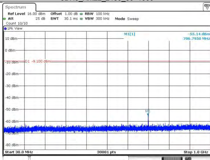
3DH5_Ant22_2480_30~1000
