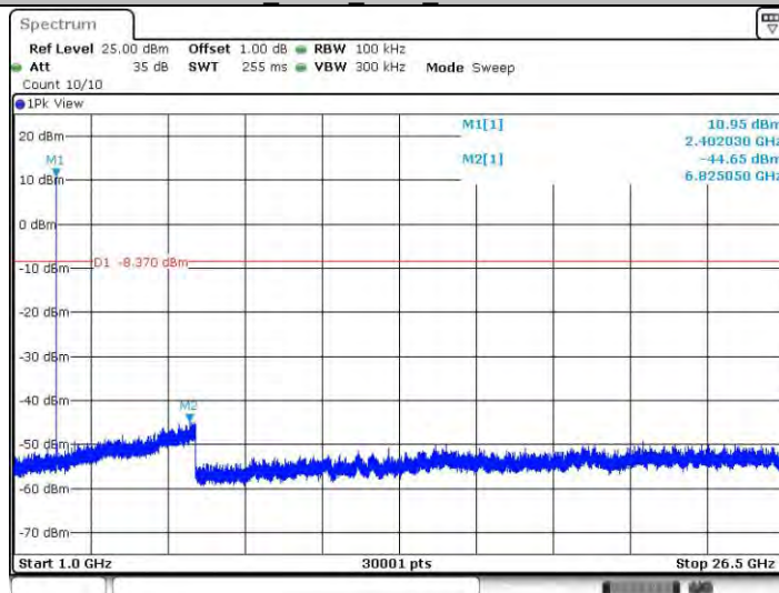
DH5_Ant22_2402_1000~26500
