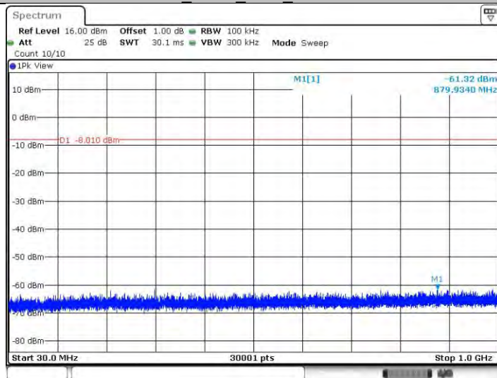
DH5_Ant22_2480_30~1000
