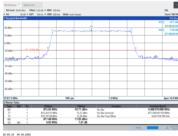
Band18(815-824)-5MHz-16QAM-23875-25RB#0
