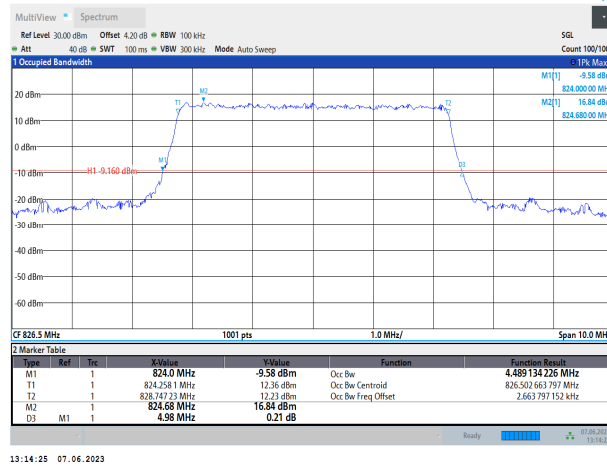
18(824-830)-5MHz-16QAM-23965-25RB#0
