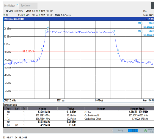
Band19-5MHz-QPSK-24075-25RB#0
