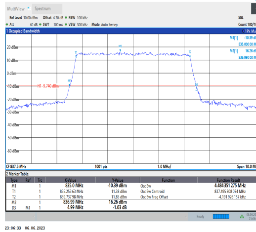
Band19-5MHz-16QAM-24075-25RB#0
