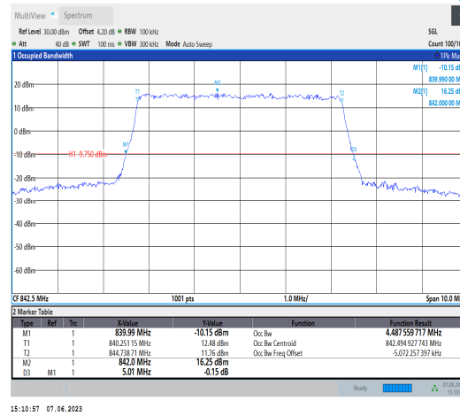
Band19-5MHz-64QAM-24125-25RB#0
