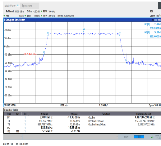
Band19-5MHz-QPSK-24025-25RB#0
