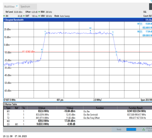
Band19-10MHz-64QAM-24075-50RB#
