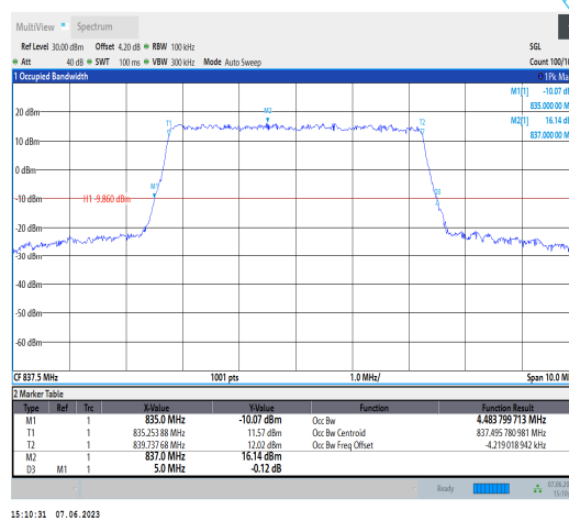
Band19-5MHz-64QAM-24075-25RB#0
