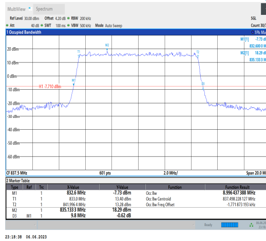
Band19-10MHz-QPSK-24075-50RB#0
