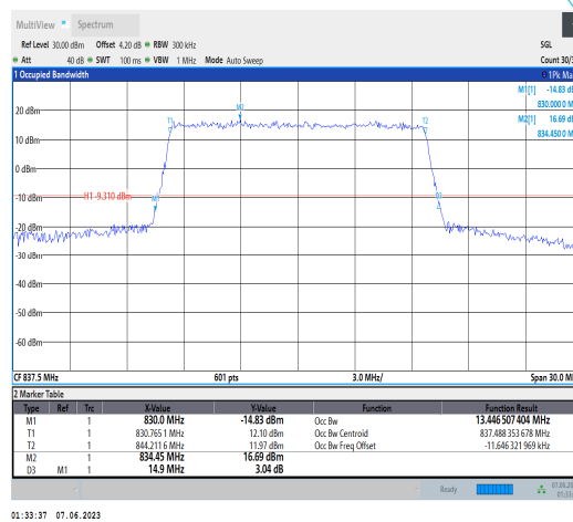
Band19-15MHz-16QAM-24075-75RB#0
