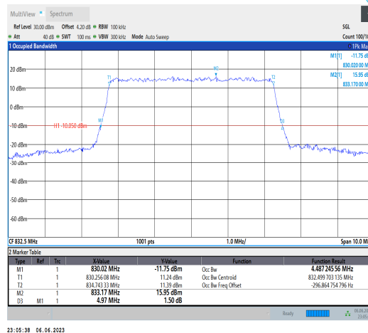
Band19-5MHz-16QAM-24025-25RB#0
