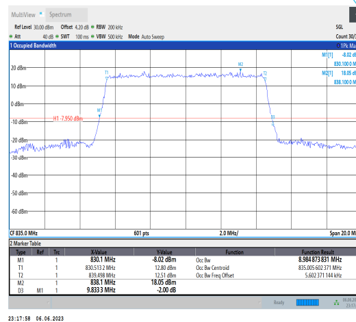
Band19-10MHz-QPSK-24050-50RB#0
