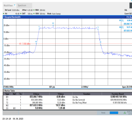
Band19-10MHz-QPSK-24100-50RB#
