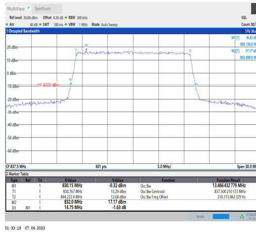
Band19-15MHz-QPSK-24075-75RB#0
