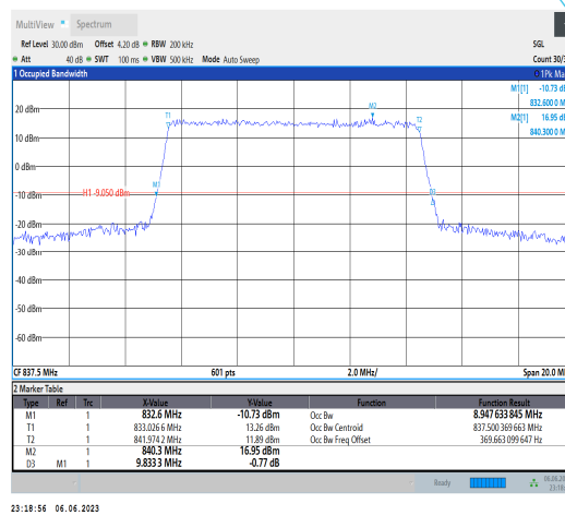
Band19-10MHz-16QAM-24075-50RB#0
