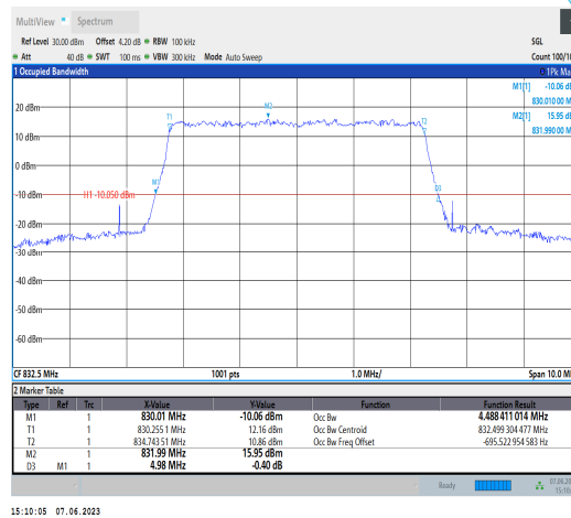
Band19-5MHz-64QAM-24025-25RB#0
