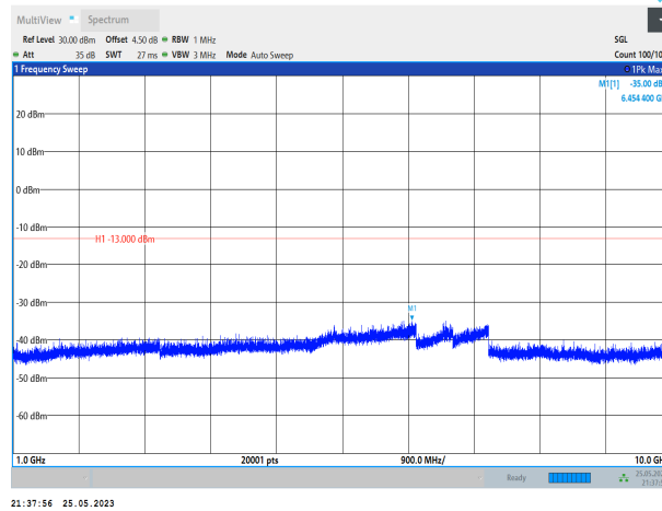
Band26-10MHz-QPSK-26740-1RB#0-Range4:1000~10000MHz
