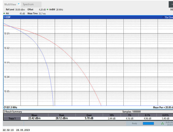
Band26-15MHz-QPSK-26915-75RB#0
