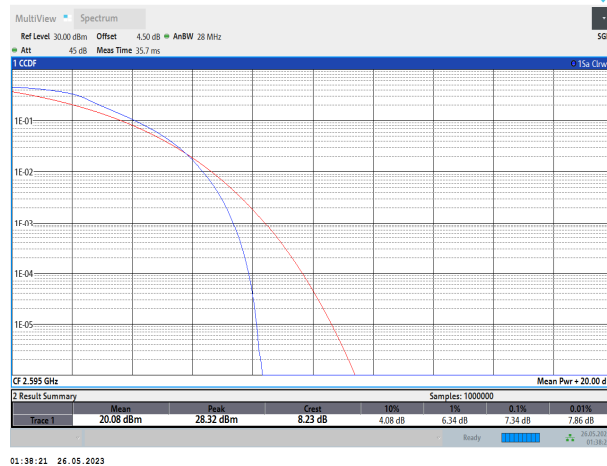
Band38-20MHz-QPSK-38000-100RB#0
