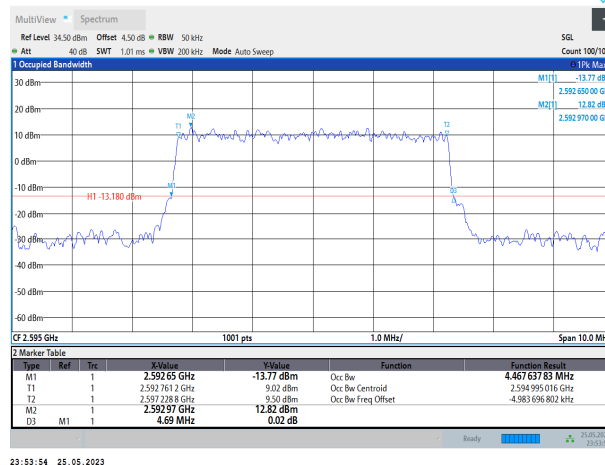
Band38-5MHz-QPSK-38000-25RB#0
