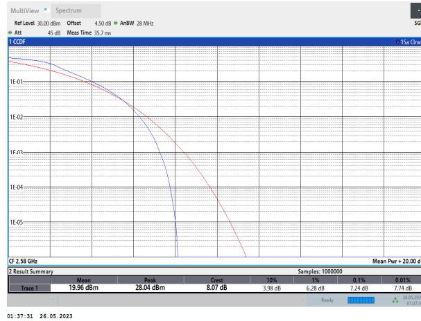
Band38-20MHz-QPSK-38000-100RB#0
