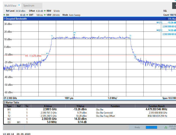
Band41-5MHz-QPSK-40620-25RB#0
