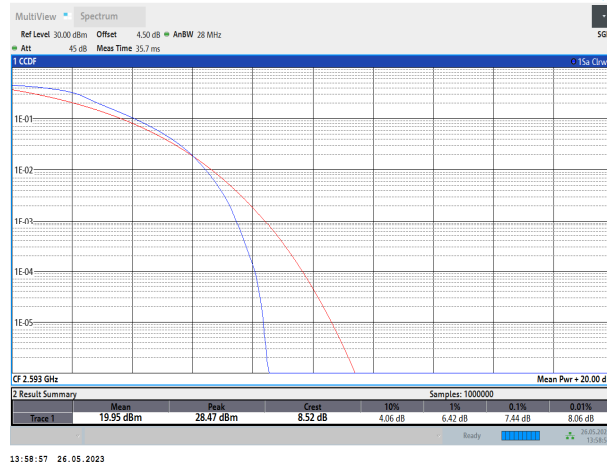
Band41-20MHz-QPSK-40620-100RB#0
