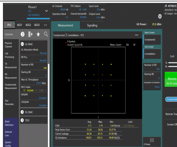
Band41-20MHz-16QAM-40620-100RB#0
