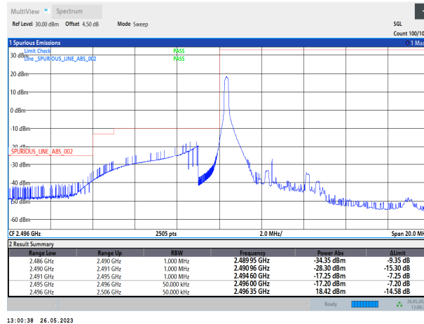
Band41-5MHz-QPSK-39675-25RB#0
