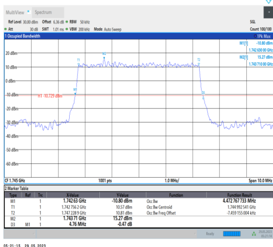
NTNV_N66_PC3_15_5_M_TID2_Ant1#1
