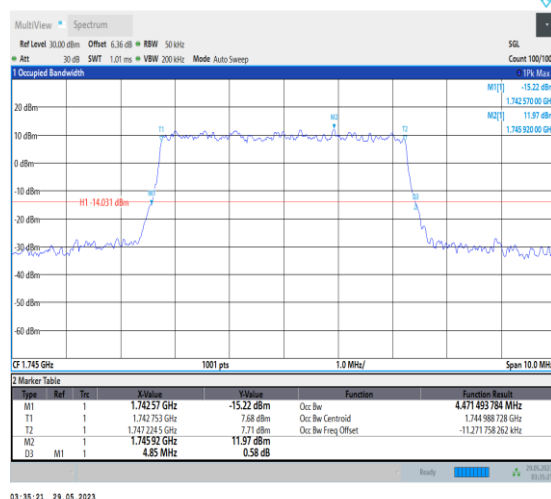
NTNV_N66_PC3_15_5_M_TID3_Ant1#1
