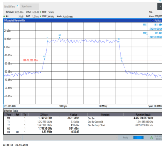
NTNV_N66_PC3_15_5_M_TID5_Ant1#1
