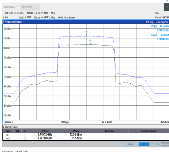
NTNV_N66_PC3_15_40_M_TID1_#1
