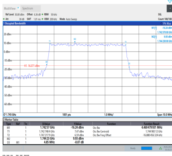
NTNV_N66_PC3_15_5_M_TID6_Ant1#1
