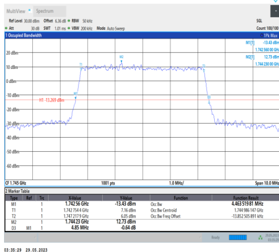
NTNV_N66_PC3_15_5_M_TID4_Ant1#1
