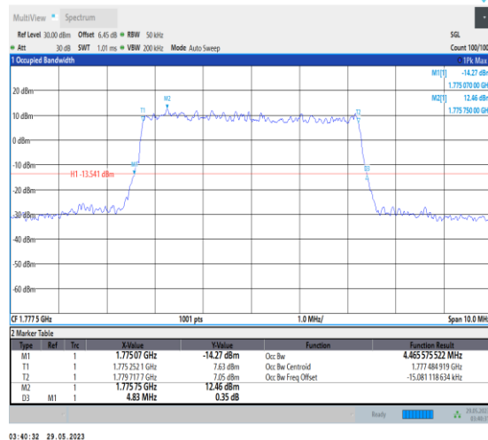
NTNV_N66_PC3_15_5_H_TID4_Ant1#1
