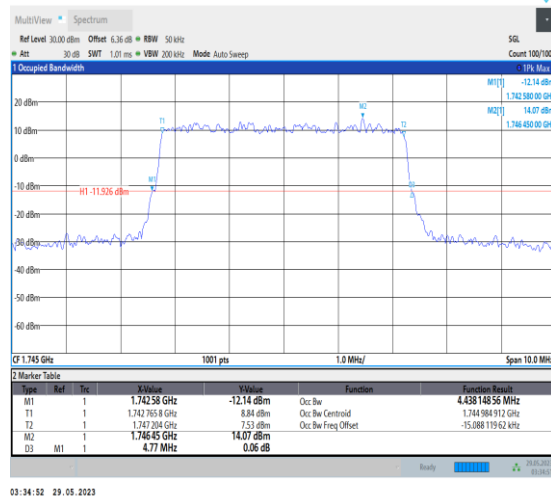
NTNV_N66_PC3_15_5_M_TID1_Ant1#1
