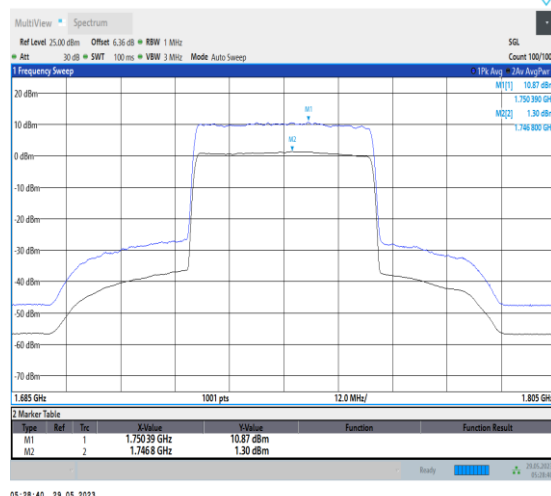
NTNV_N66_PC3_15_40_M_TID2_#1
