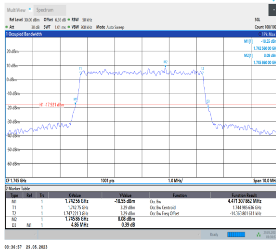
NTNV_N66_PC3_15_5_M_TID9_Ant1#1
