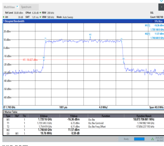
NTNV_N66_PC3_15_20_M_TID8_Ant1#1
