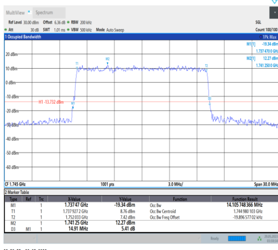
NTNV_N66_PC3_15_15_M_TID8_Ant1#1
