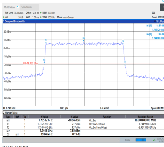
NTNV_N66_PC3_15_20_M_TID9_Ant1#1
