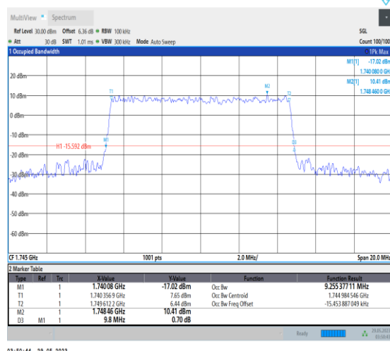
NTNV_N66_PC3_15_10_M_TID8_Ant1#1
