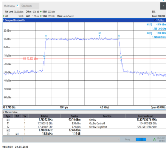
NTNV_N66_PC3_15_20_M_TID4_Ant1#1
