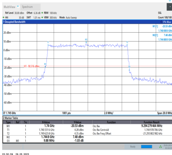
NTNV_N66_PC3_15_10_M_TID9_Ant1#1
