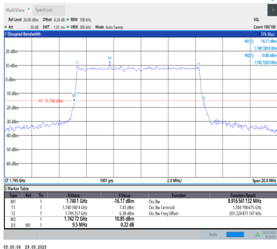
NTNV_N66_PC3_15_10_M_TID5_Ant1#1
