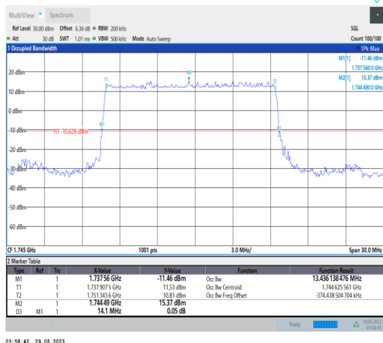
NTNV_N66_PC3_15_15_M_TID2_Ant1#1
