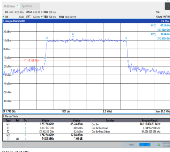
NTNV_N66_PC3_15_15_M_TID6_Ant1#1
