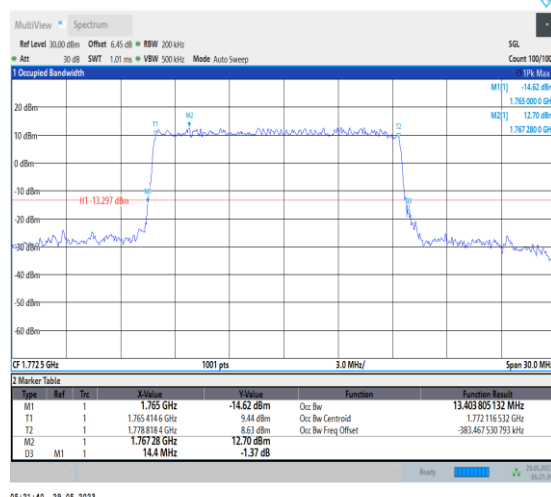
NTNV_N66_PC3_15_15_H_TID4_Ant1#1
