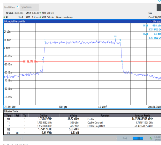
NTNV_N66_PC3_15_15_M_TID9_Ant1#1
