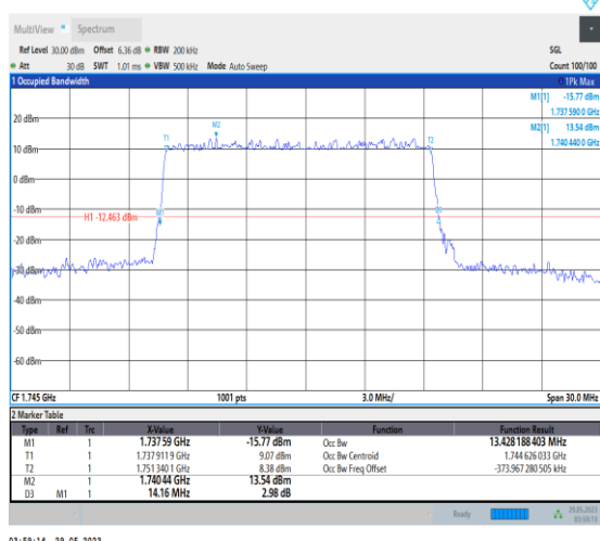
NTNV_N66_PC3_15_15_M_TID4_Ant1#1
