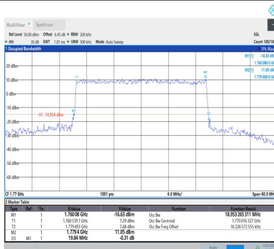
NTNV_N66_PC3_15_20_H_TID4_Ant1#1
