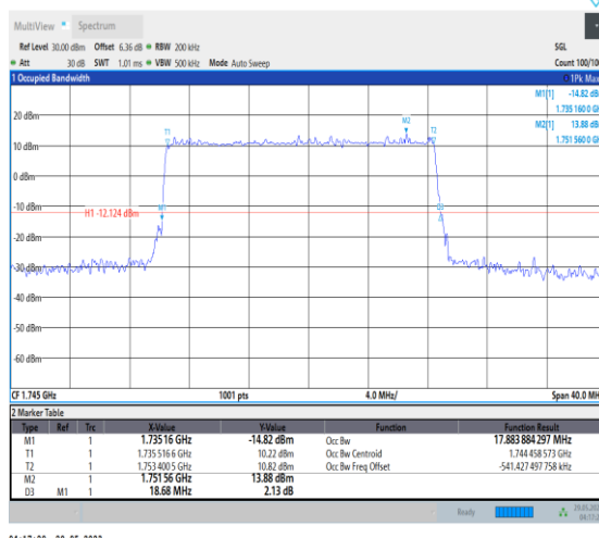
NTNV_N66_PC3_15_20_M_TID1_Ant1#1
