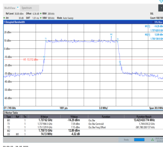
NTNV_N66_PC3_15_15_M_TID5_Ant1#1
