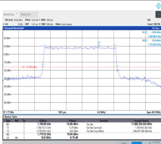
NTNV_N66_PC3_15_20_H_TID3_Ant1#1
