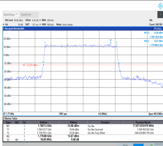
NTNV_N66_PC3_15_20_M_TID8_Ant1#1
