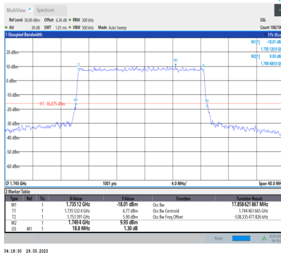
NTNV_N66_PC3_15_20_M_TID5_Ant1#1
