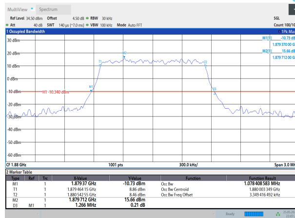
Band2-1.4MHz-QPSK-18900-6RB#0
