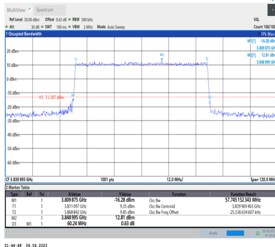
1-N77-3700-3980-PC3-30-60-M-3-DFT-16QAM-Outer_Full-162@0-Ant1-57.745-60.240-≤60-PASS
