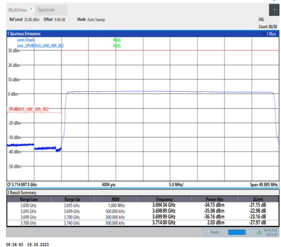
1-N77-3700-3980-PC3-30-40-L-6-CP-QPSK-Outer_Full-106@0-Ant1-1--PASS-see graph
