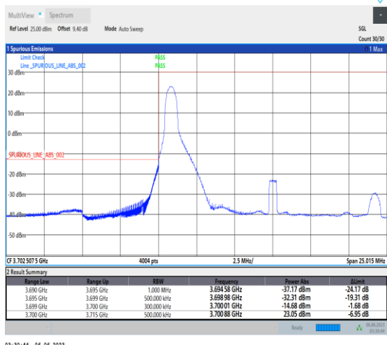
1-N77-3700-3980-PC3-30-15-L-1-DFT-PI2BPSK-Edge_1RB_Left-1@0-Ant1-1--PASS-see graph
