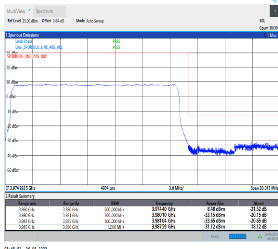
1-N77-3700-3980-PC3-30-20-H-3-DFT-PI2BPSK-Outer_Full-50@0-Ant1-1-PASS-see graph
