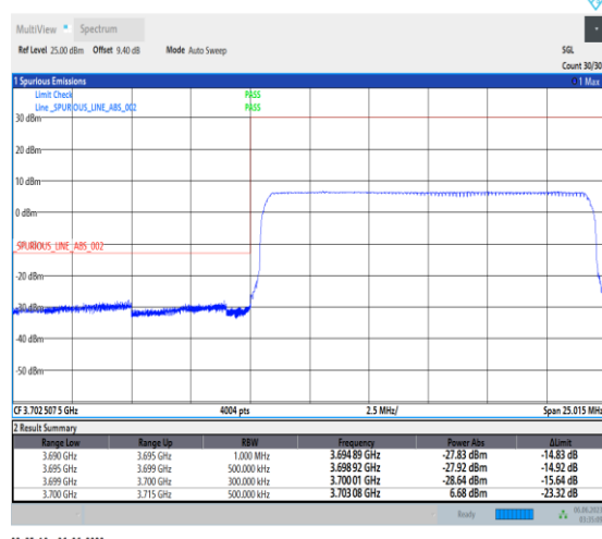
1-N77-3700-3980-PC3-30-15-L-6-CP-QPSK-Outer_Full-38@0-Ant1-1--PASS-see graph
