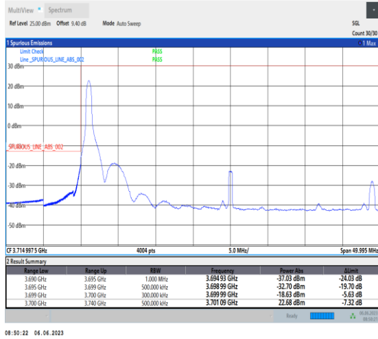
1-N77-3700-3980-PC3-30-40-L-1-DFT-PI2BPSK-Edge_1RB_Left-1@0-Ant1-1--PASS-see graph
