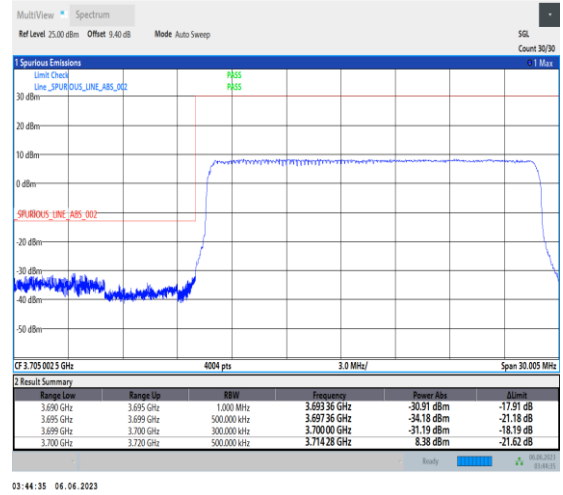
1-N77-3700-3980-PC3-30-20-L-3-DFT-PI2BPSK-Outer_Full-50@0-Ant1-1--PASS-see graph
