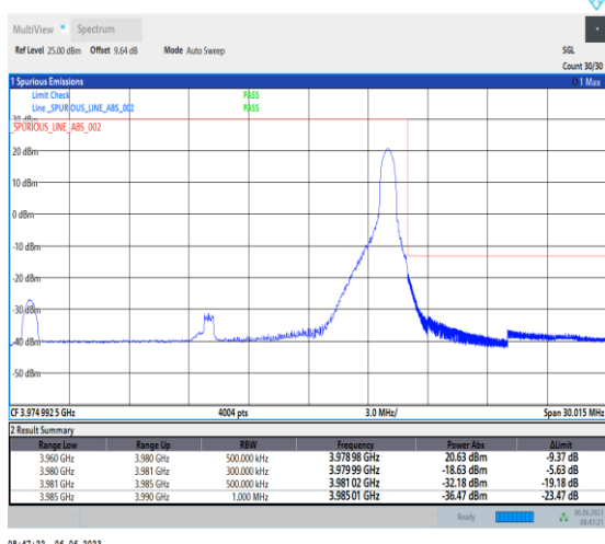
1-N77-3700-3980-PC3-30-20-H-5-CP-QPSK-Edge_1RB_Right-1@50-Ant1-1-PASS-see graph
