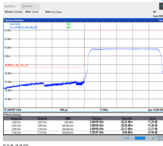
1-N77-3700-3980-PC3-30-10-L-6-CP-QPSK-Outer_Full-24@0-Ant1-1--PASS-see graph
