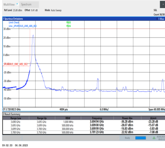
1-N77-3700-3980-PC3-30-50-L-1-DFT-PI2BPSK-Edge_1RB_Left-1@0-Ant1-1--PASS-see graph
