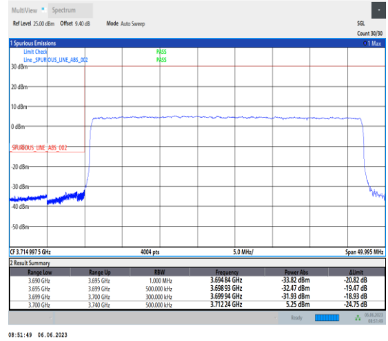
1-N77-3700-3980-PC3-30-40-L-3-DFT-PI2BPSK-Outer_Full-100@0-Ant1-1--PASS-see graph
