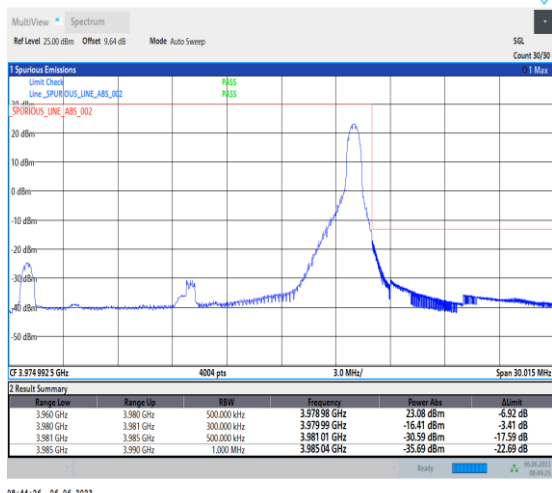
1-N77-3700-3980-PC3-30-20-H-2-DFT-PI2BPSK-Edge_1RB_Right-1@50-Ant1-1-PASS-see graph
