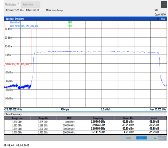
1-N77-3700-3980-PC3-30-50-L-3-DFT-PI2BPSK-Outer_Full-128@0-Ant1-1--PASS-see graph
