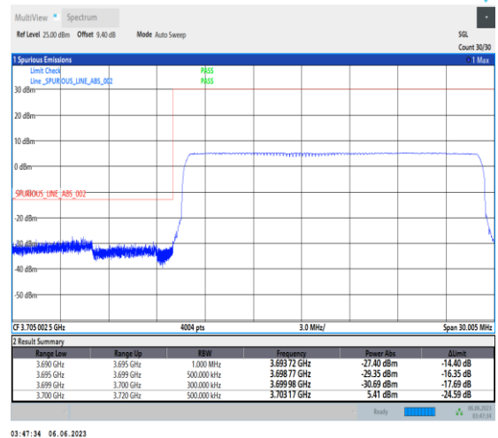
1-N77-3700-3980-PC3-30-20-L-6-CP-QPSK-Outer_Full-51@0-Ant1-1--PASS-see graph
