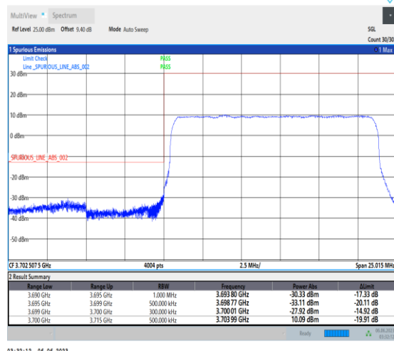
1-N77-3700-3980-PC3-30-15-L-3-DFT-PI2BPSK-Outer_Full-36@0-Ant1-1--PASS-see graph
