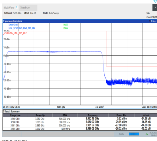
1-N77-3700-3980-PC3-30-20-H-6-CP-QPSK-Outer_Full-51@0-Ant1-1-PASS-see graph
