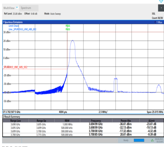
1-N77-3700-3980-PC3-30-15-L-4-CP-QPSK-Edge_1RB_Left-1@0-Ant1-1--PASS-see graph
