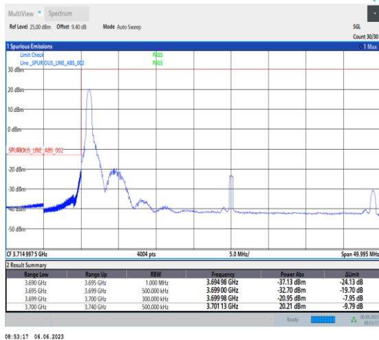
1-N77-3700-3980-PC3-30-40-L-4-CP-QPSK-Edge_1RB_Left-1@0-Ant1-1--PASS-see graph
