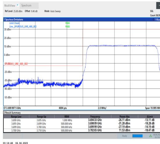
1-N77-3700-3980-PC3-30-10-L-3-DFT-PI2BPSK-Outer_Full-24@0-Ant1-1--PASS-see graph
