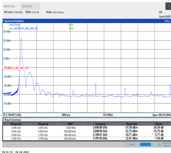
1-N77-3700-3980-PC3-30-90-L-1-DFT-PI2BPSK-Edge_1RB_Left-1@0-Ant1-1--PASS-see graph
