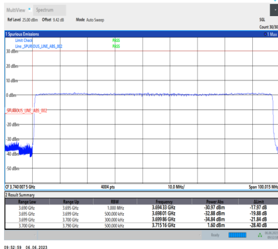
1-N77-3700-3980-PC3-30-90-L-3-DFT-PI2BPSK-Outer_Full-240@0-Ant1-1--PASS-see graph
