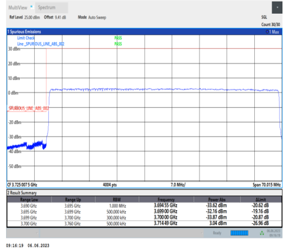
1-N77-3700-3980-PC3-30-60-L-3-DFT-PI2BPSK-Outer_Full-162@0-Ant1-1--PASS-see graph
