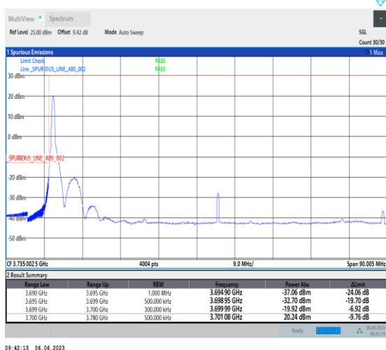
1-N77-3700-3980-PC3-30-80-L-4-CP-QPSK-Edge_1RB_Left-1@0-Ant1-1--PASS-see graph
