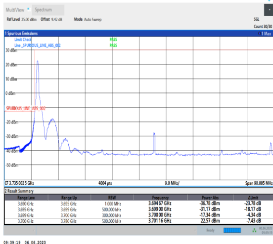
1-N77-3700-3980-PC3-30-80-L-1-DFT-PI2BPSK-Edge_1RB_Left-1@0-Ant1-1--PASS-see graph
