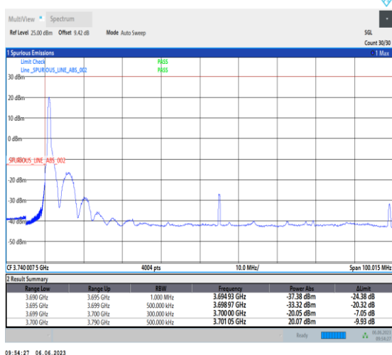
1-N77-3700-3980-PC3-30-90-L-4-CP-QPSK-Edge_1RB_Left-1@0-Ant1-1--PASS-see graph
