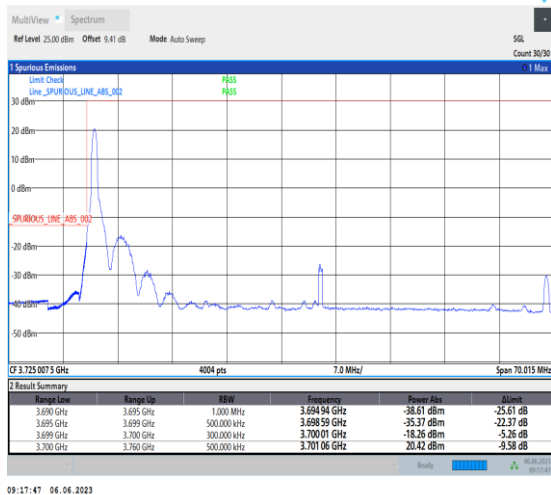
1-N77-3700-3980-PC3-30-60-L-4-CP-QPSK-Edge_1RB_Left-1@0-Ant1-1--PASS-see graph
