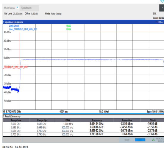
1-N77-3700-3980-PC3-30-90-L-6-CP-QPSK-Outer_Full-245@0-Ant1-1--PASS-see graph
