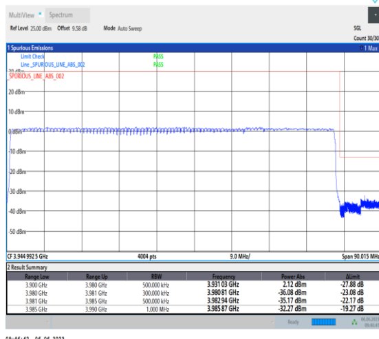
1-N77-3700-3980-PC3-30-80-H-3-DFT-PI2BPSK-Outer_Full-216@0-Ant1-1--PASS-see graph
