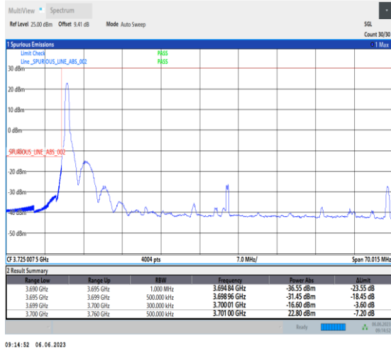
1-N77-3700-3980-PC3-30-60-L-1-DFT-PI2BPSK-Edge_1RB_Left-1@0-Ant1-1--PASS-see graph
