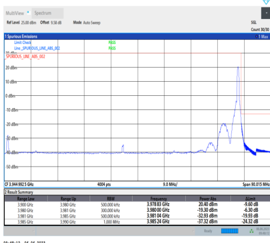
1-N77-3700-3980-PC3-30-80-H-5-CP-QPSK-Edge_1RB_Right-1@216-Ant1-1--PASS-see graph
