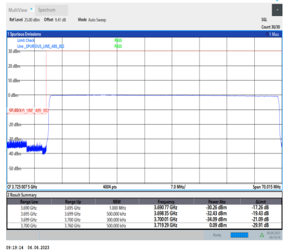
1-N77-3700-3980-PC3-30-60-L-6-CP-QPSK-Outer_Full-162@0-Ant1-1--PASS-see graph
