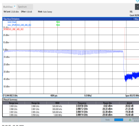
1-N77-3700-3980-PC3-30-80-H-6-CP-QPSK-Outer_Full-217@0-Ant1-1--PASS-see graph
