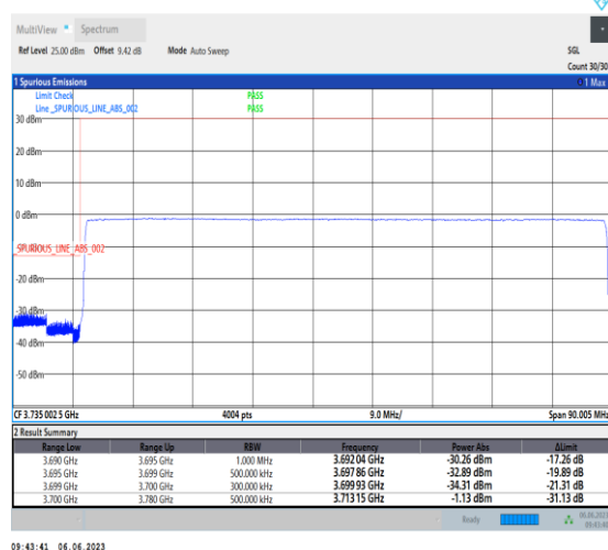
1-N77-3700-3980-PC3-30-80-L-6-CP-QPSK-Outer_Full-217@0-Ant1-1--PASS-see graph
