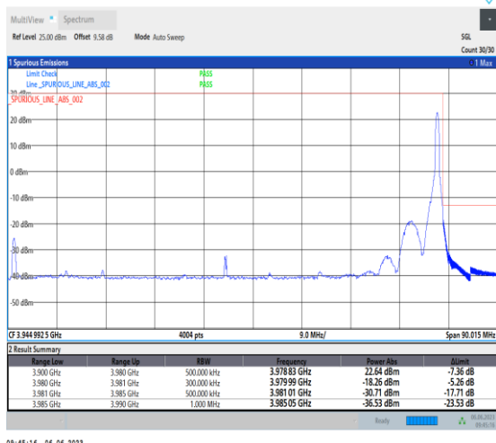
1-N77-3700-3980-PC3-30-80-H-2-DFT-PI2BPSK-Edge_1RB_Right-1@216-Ant1-1--PASS-see graph
